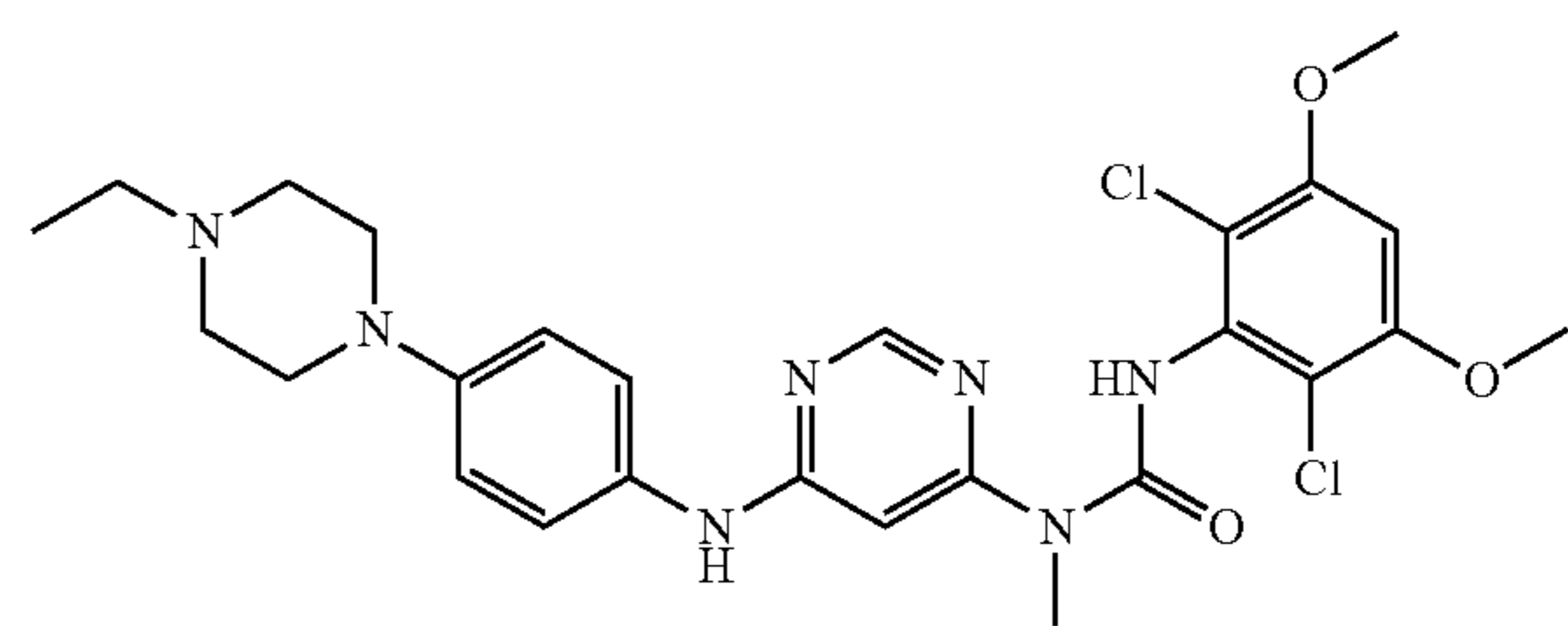
A. N-[4-(4-ethyl-piperazin-1-yl)-phenyl]-N'-methyl-pyrimidine-4,6-diamine
