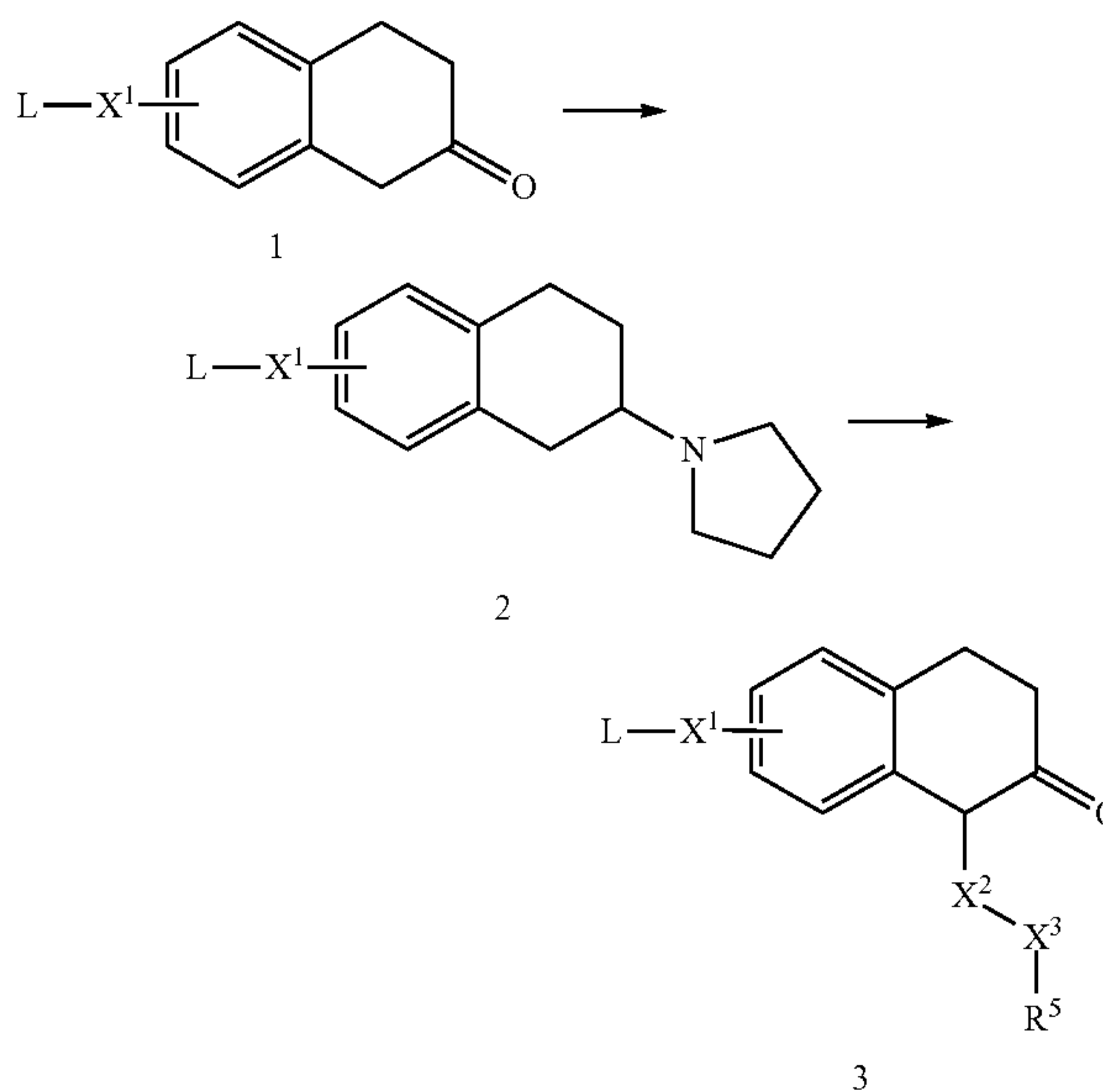
Scheme 1:
