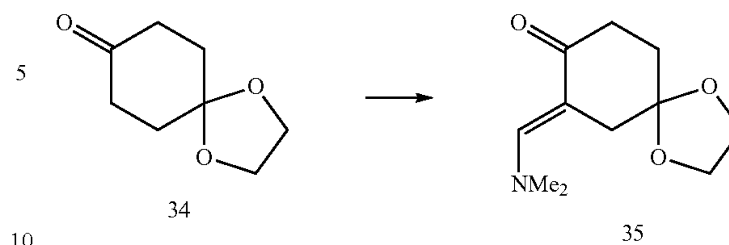
Scheme 7:
