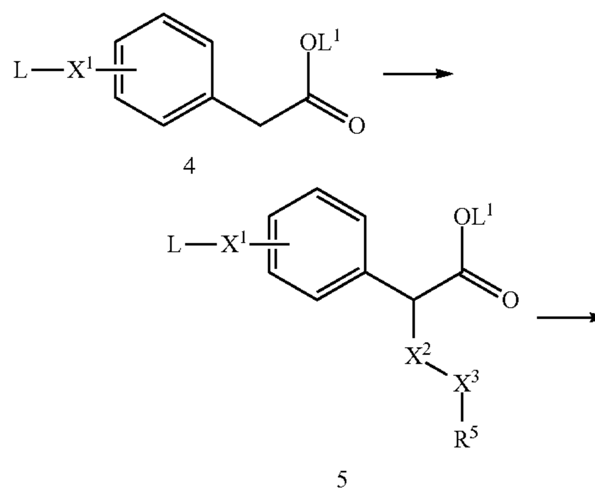
Scheme 2:
