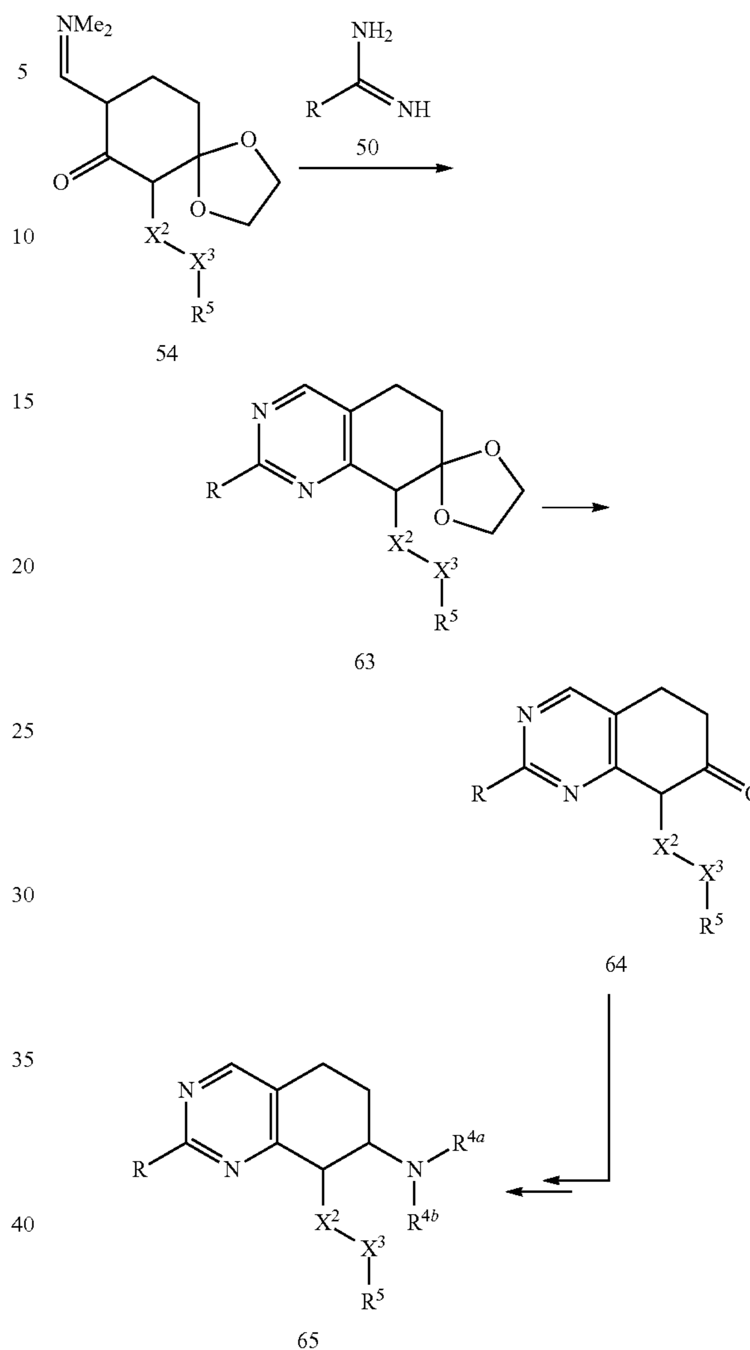
Scheme 15:
