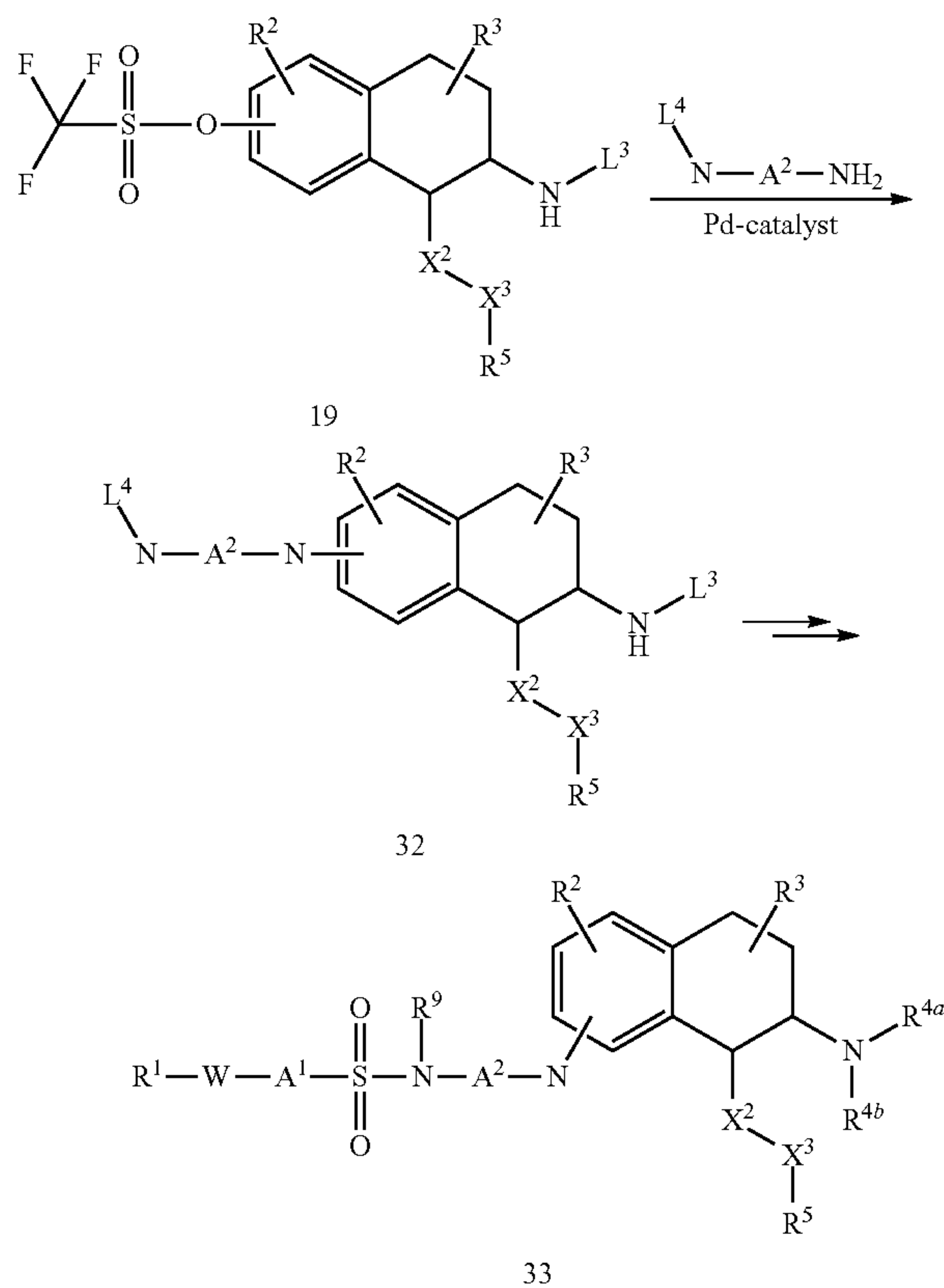
Scheme 6:
