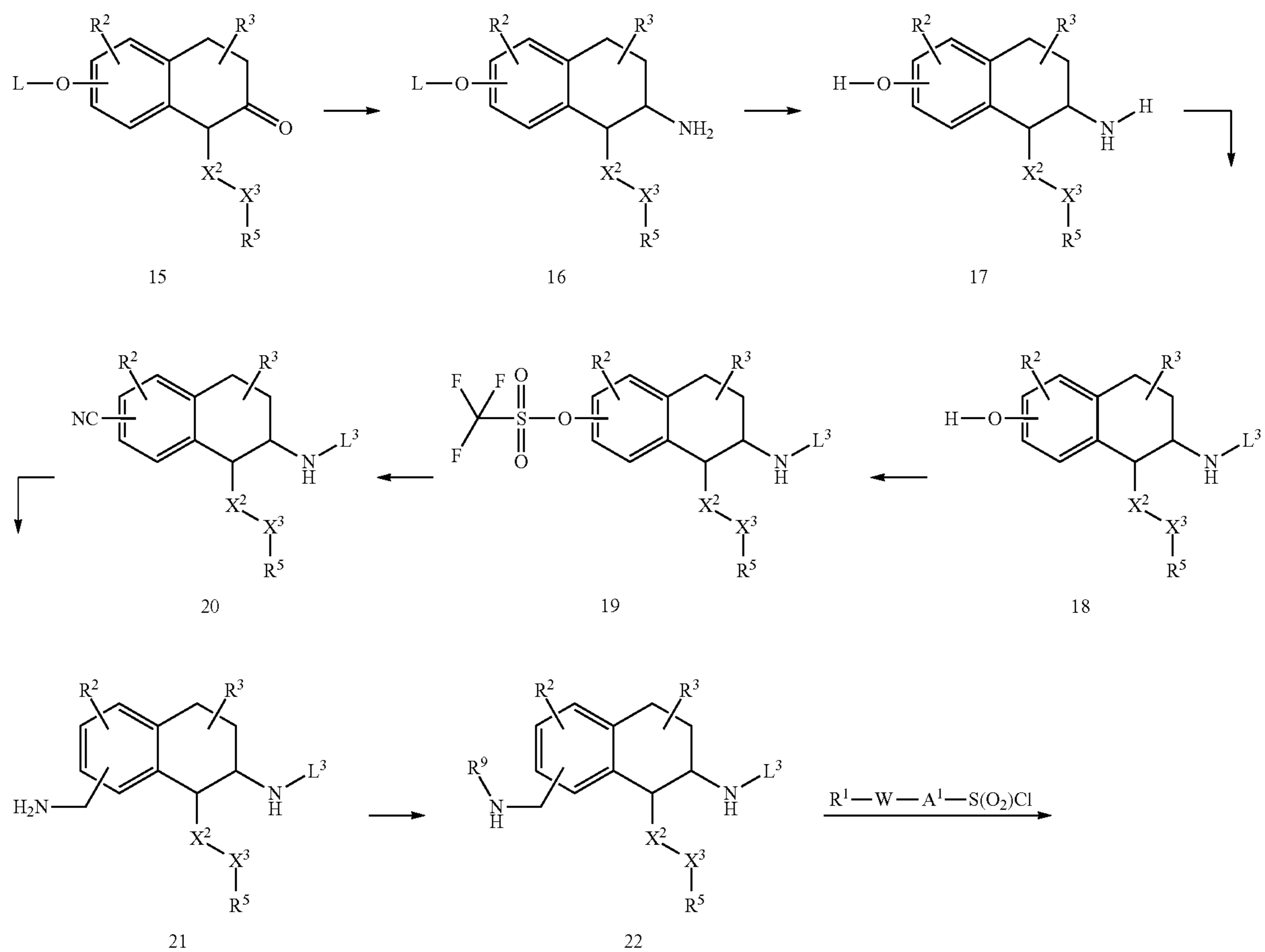
Scheme 4:
