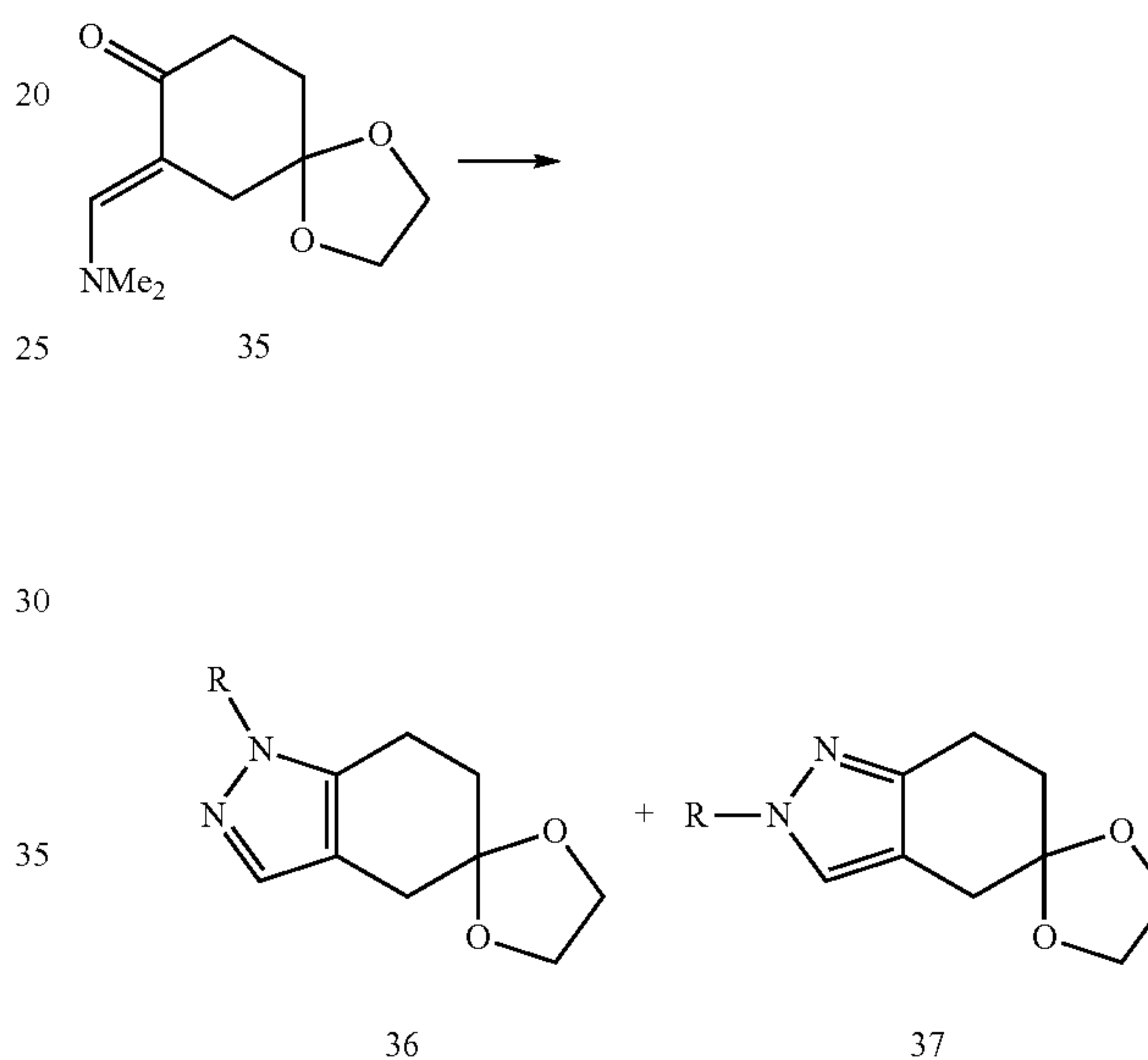
Scheme 8:
