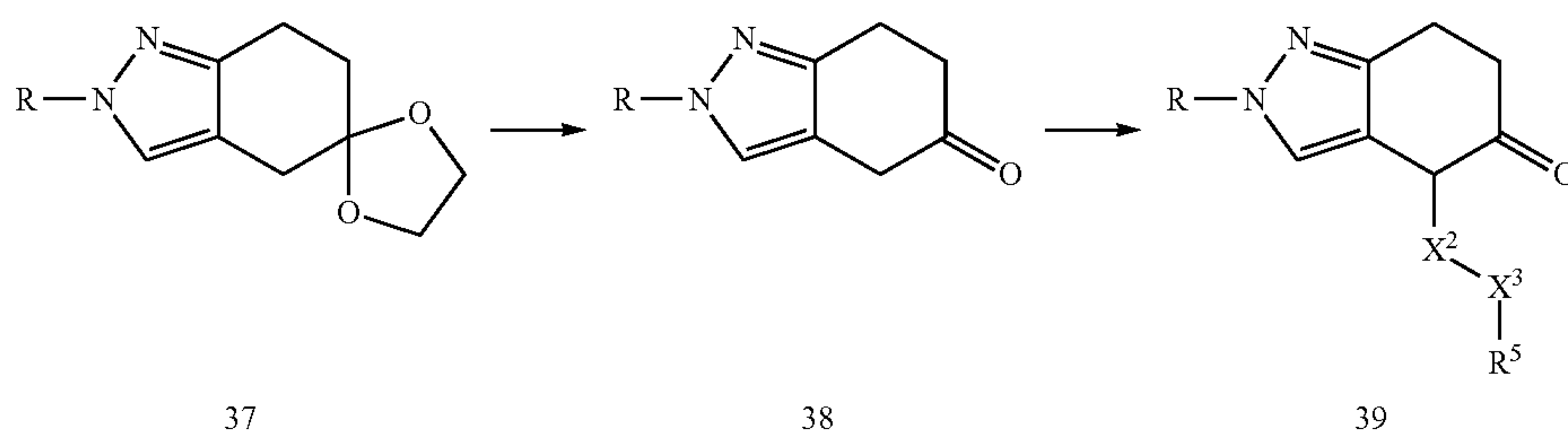
Scheme 9:
