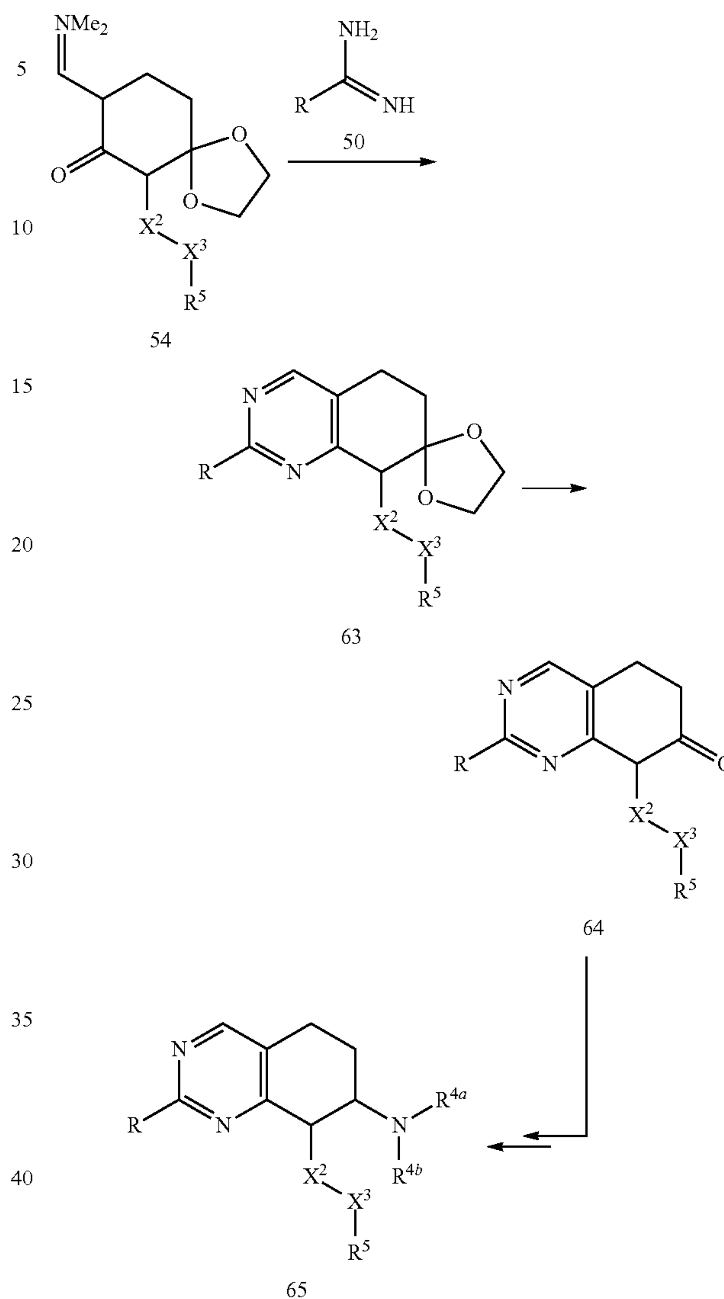
Scheme 15:
