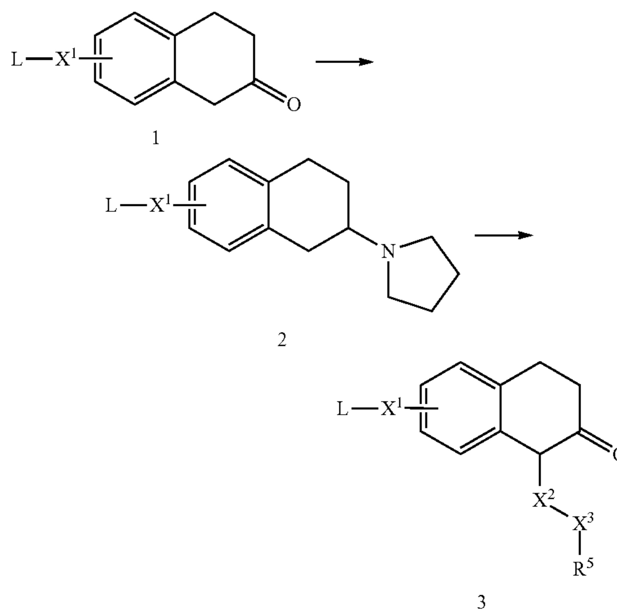
Scheme 1:
