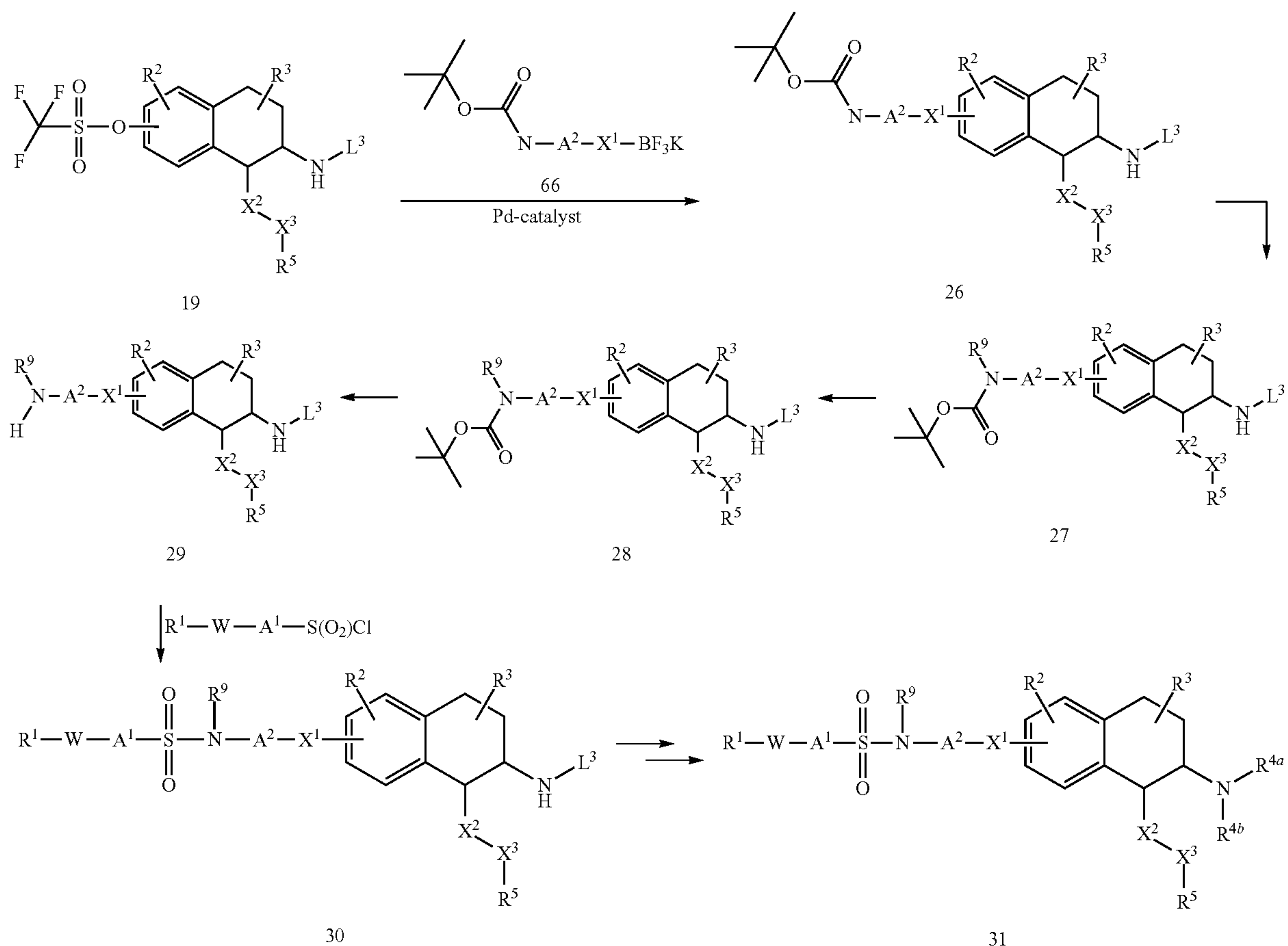
Scheme 5:
