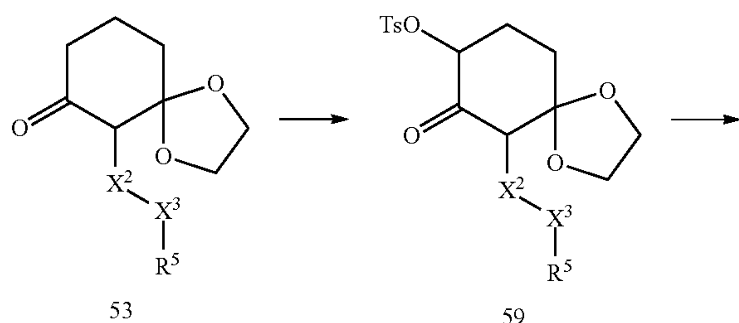
Scheme 14:
