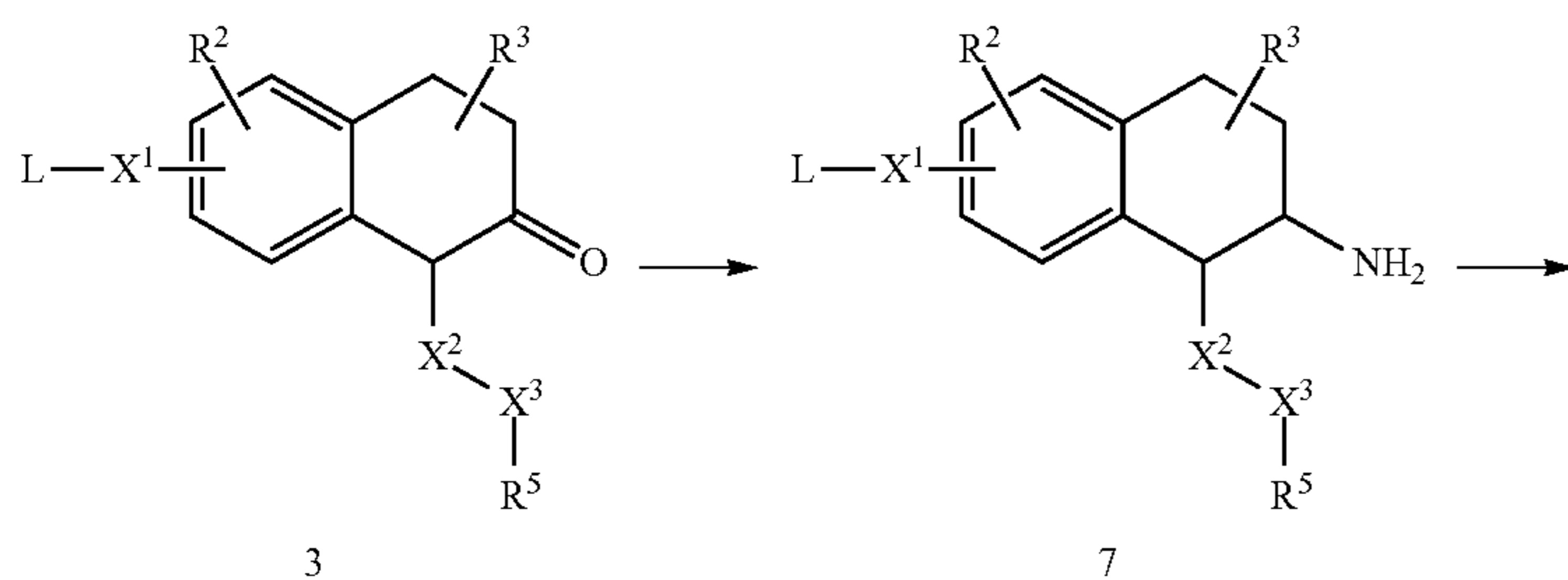
Scheme 3:
