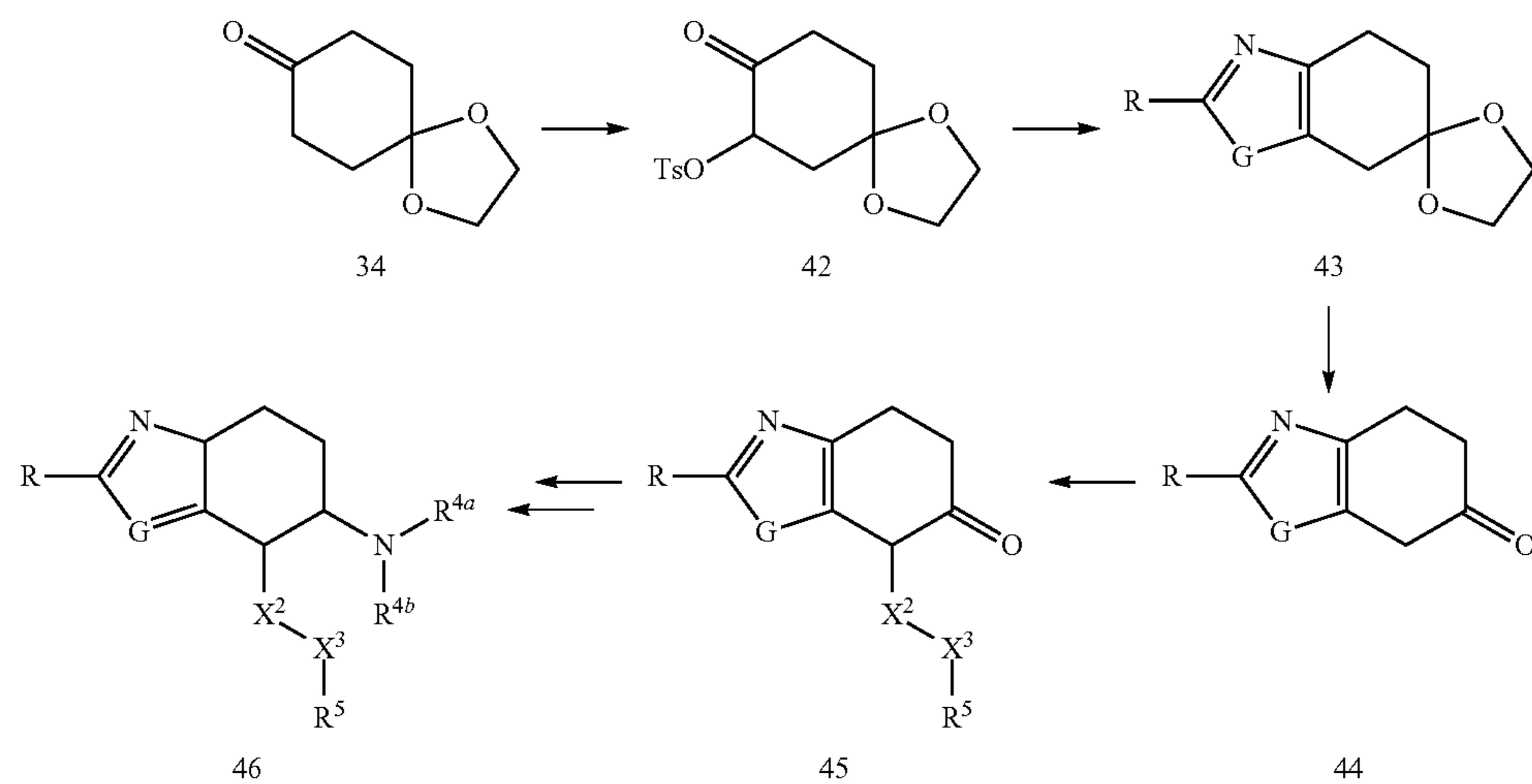
Scheme 10:
