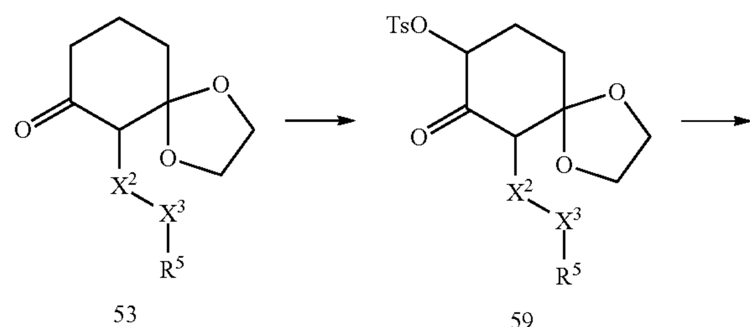
Scheme 14:
