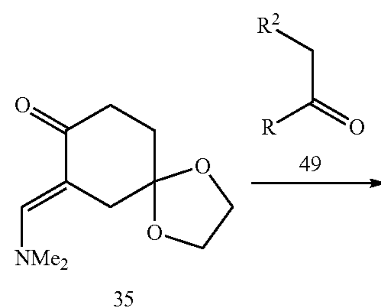
Scheme 11:
