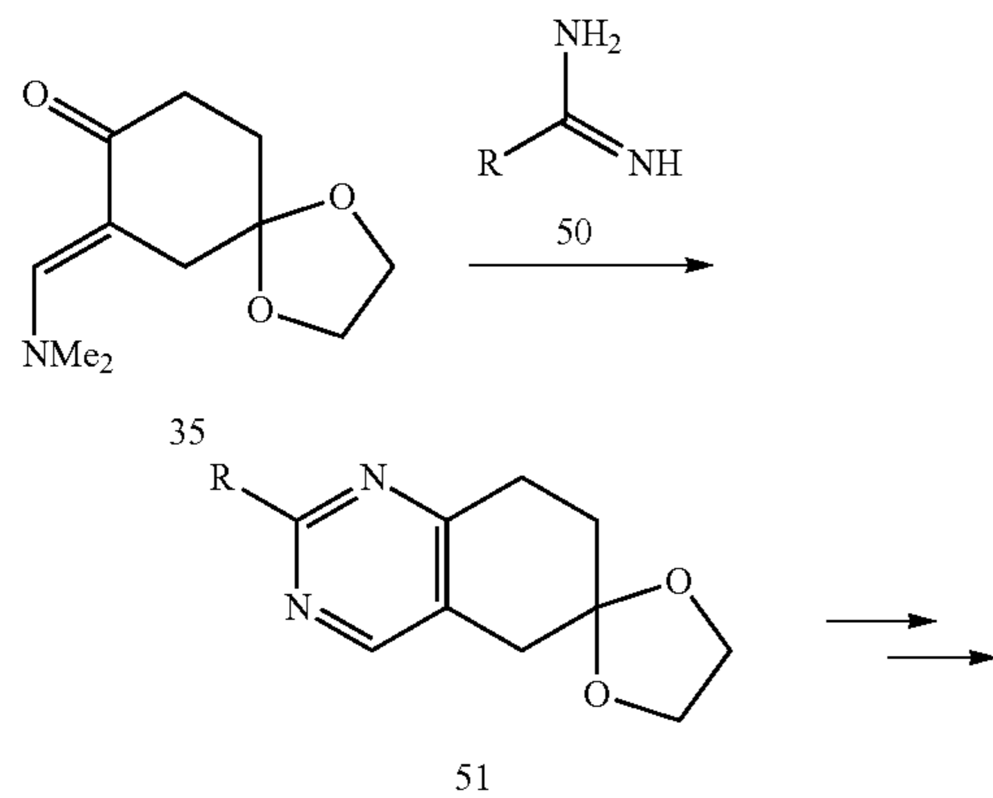
Scheme 12:
