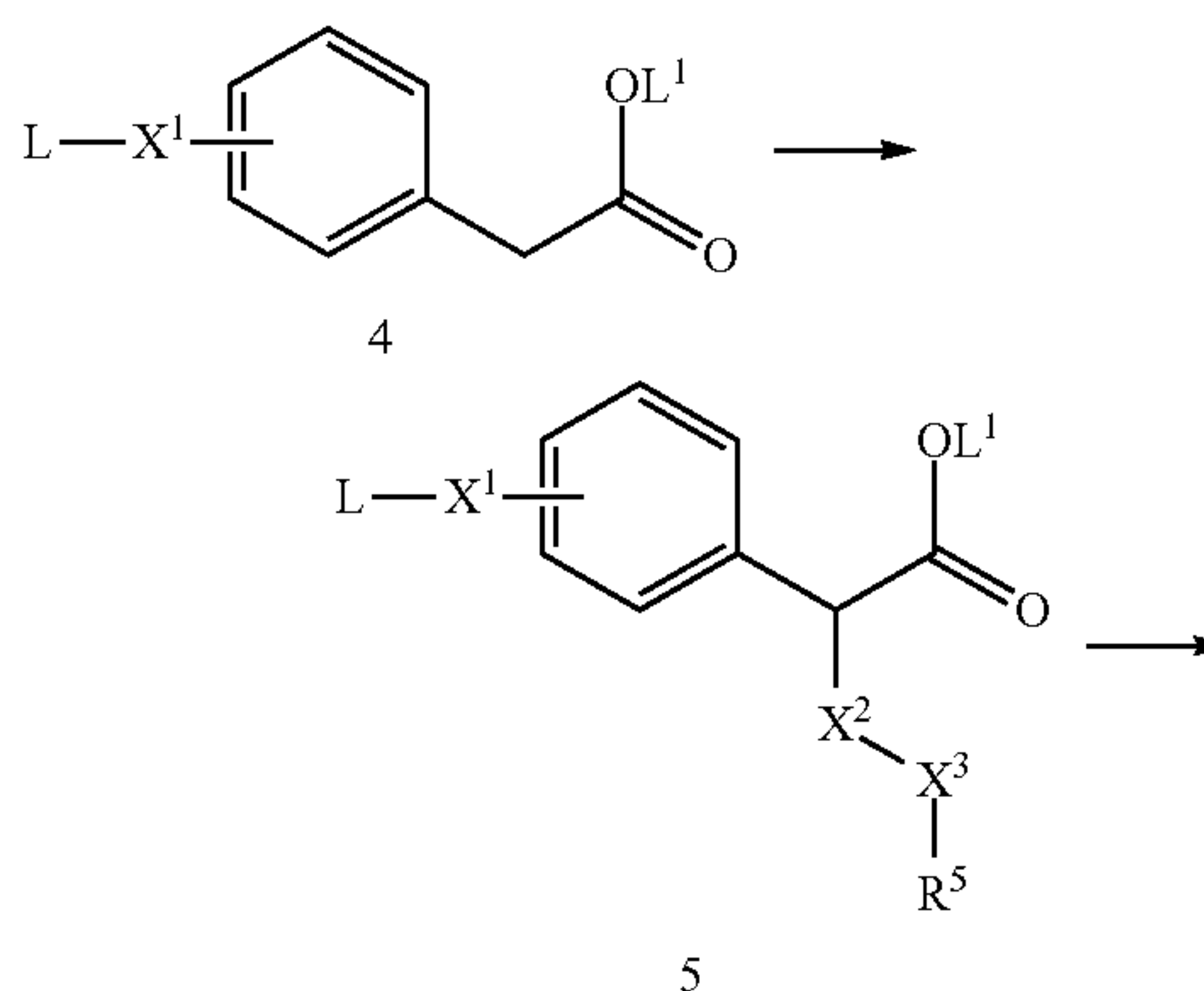
Scheme 2:
