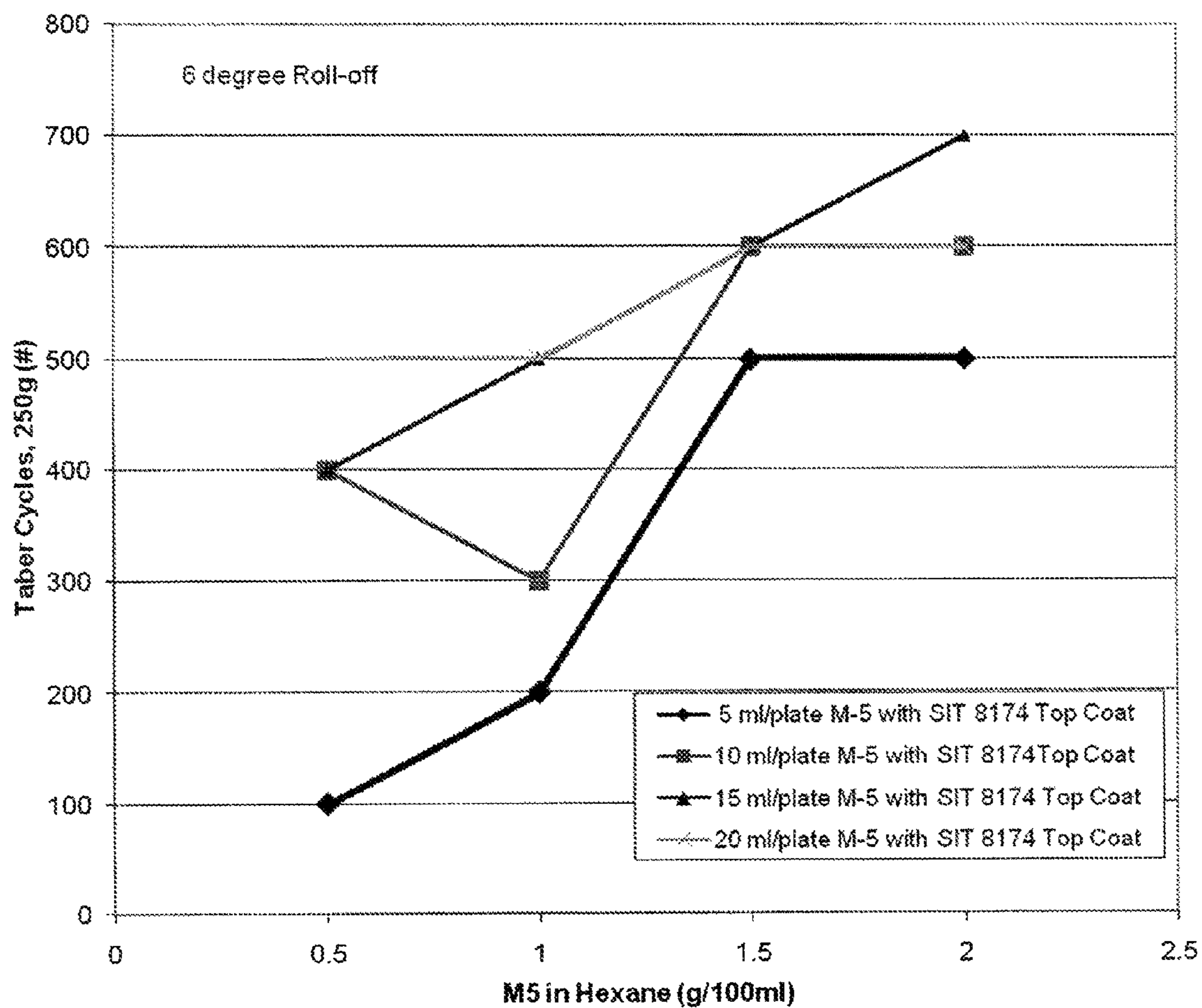
Figure 3: Taber cycles as affected by concentration of M5 and the amount of M5 used per 4- x 4-in. aluminum plate.
