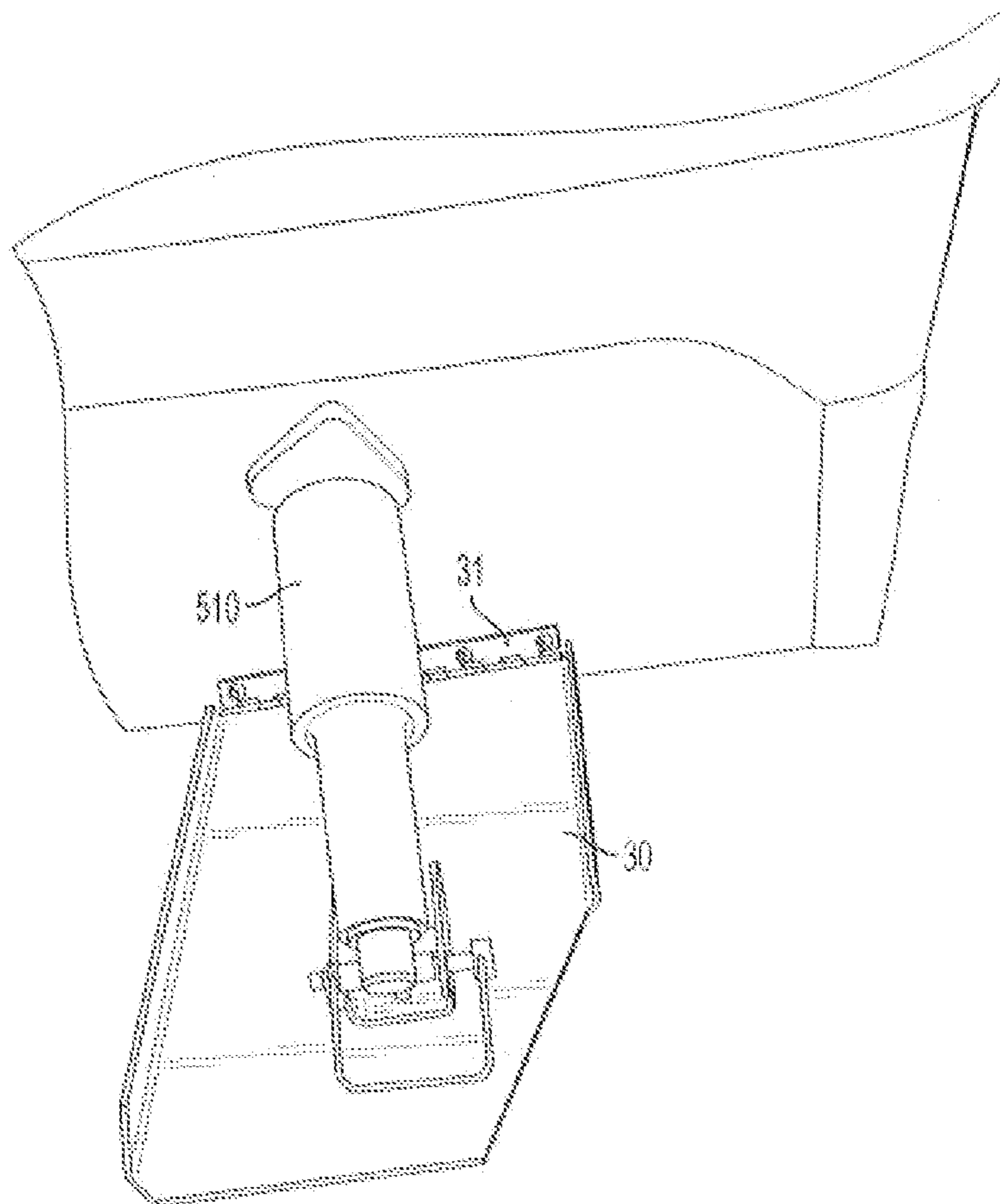
FIG. 2 PRIOR ART
