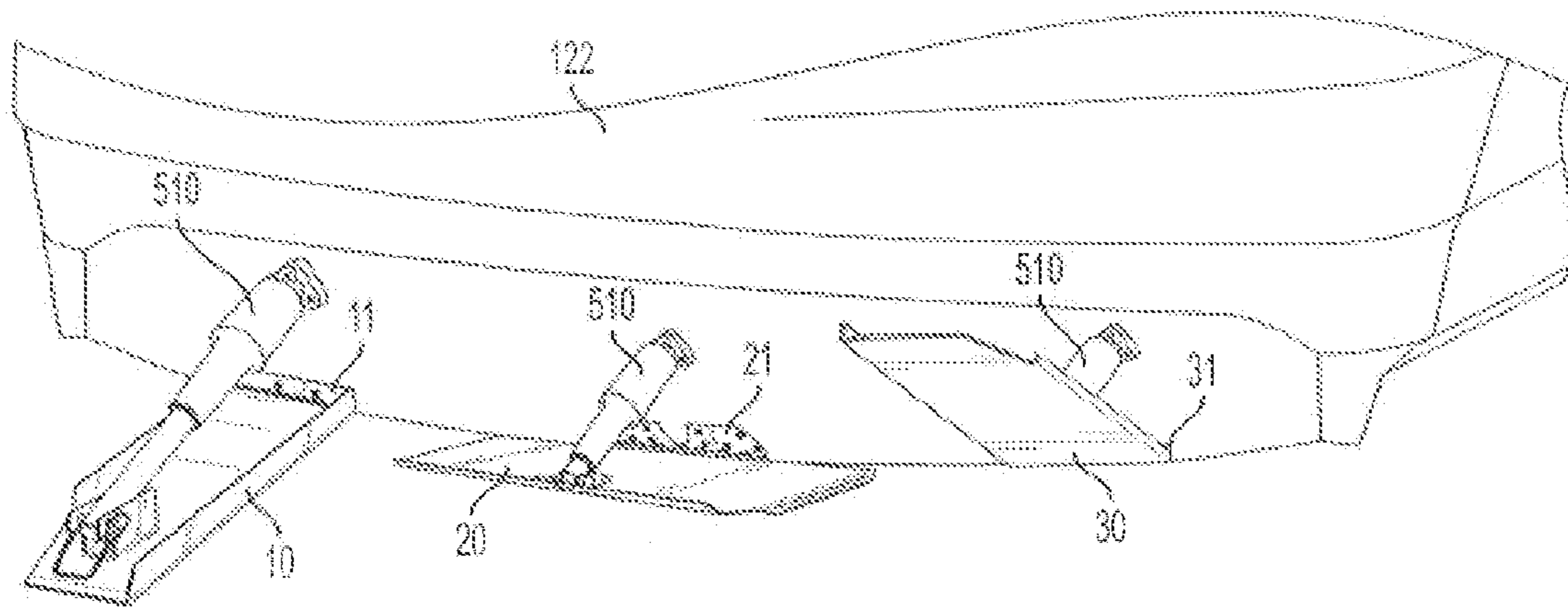
FIG. 1 PRIOR ART
