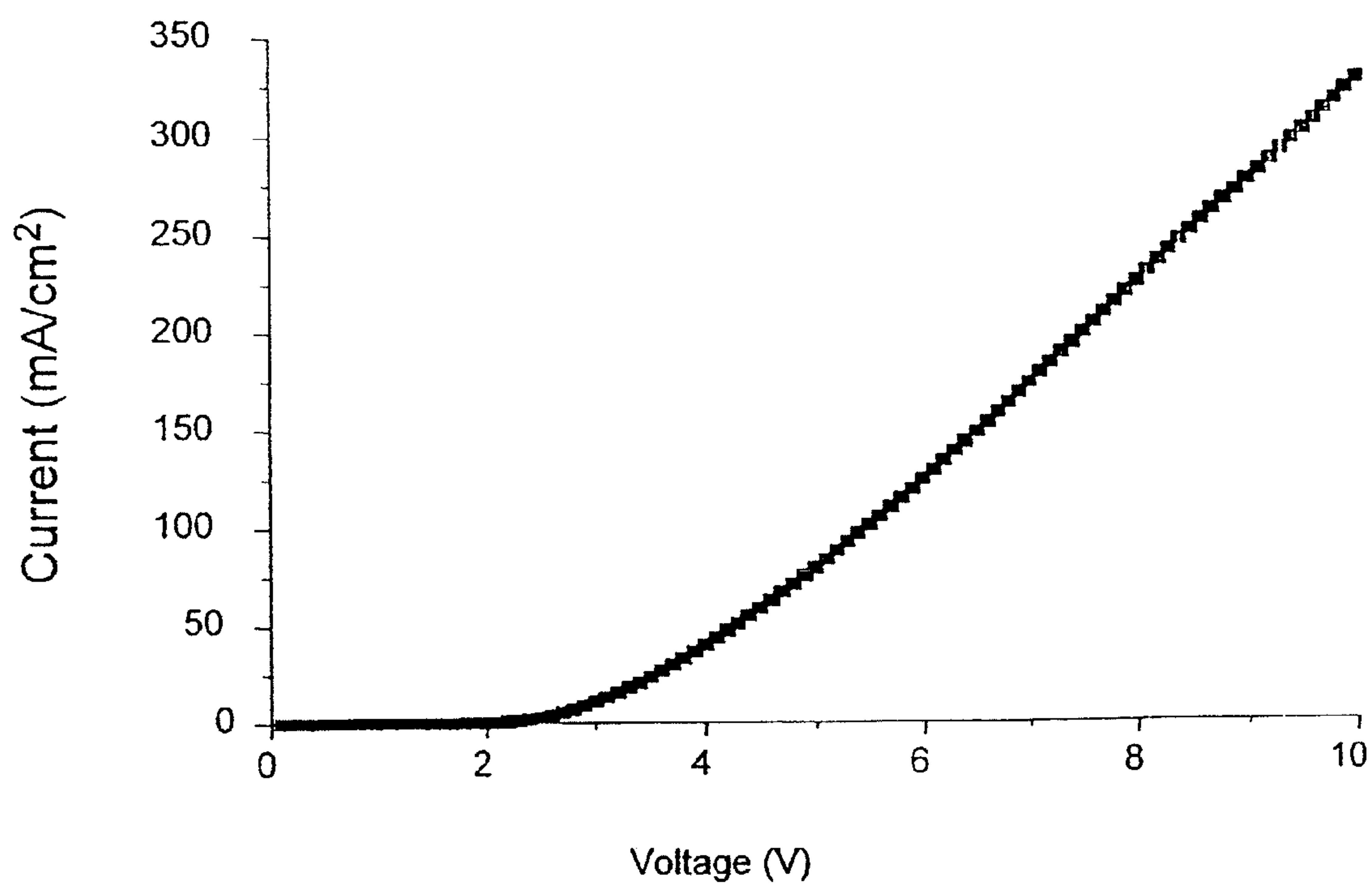
Figure 4(a): Current-voltage characteristics of device in figure 3
