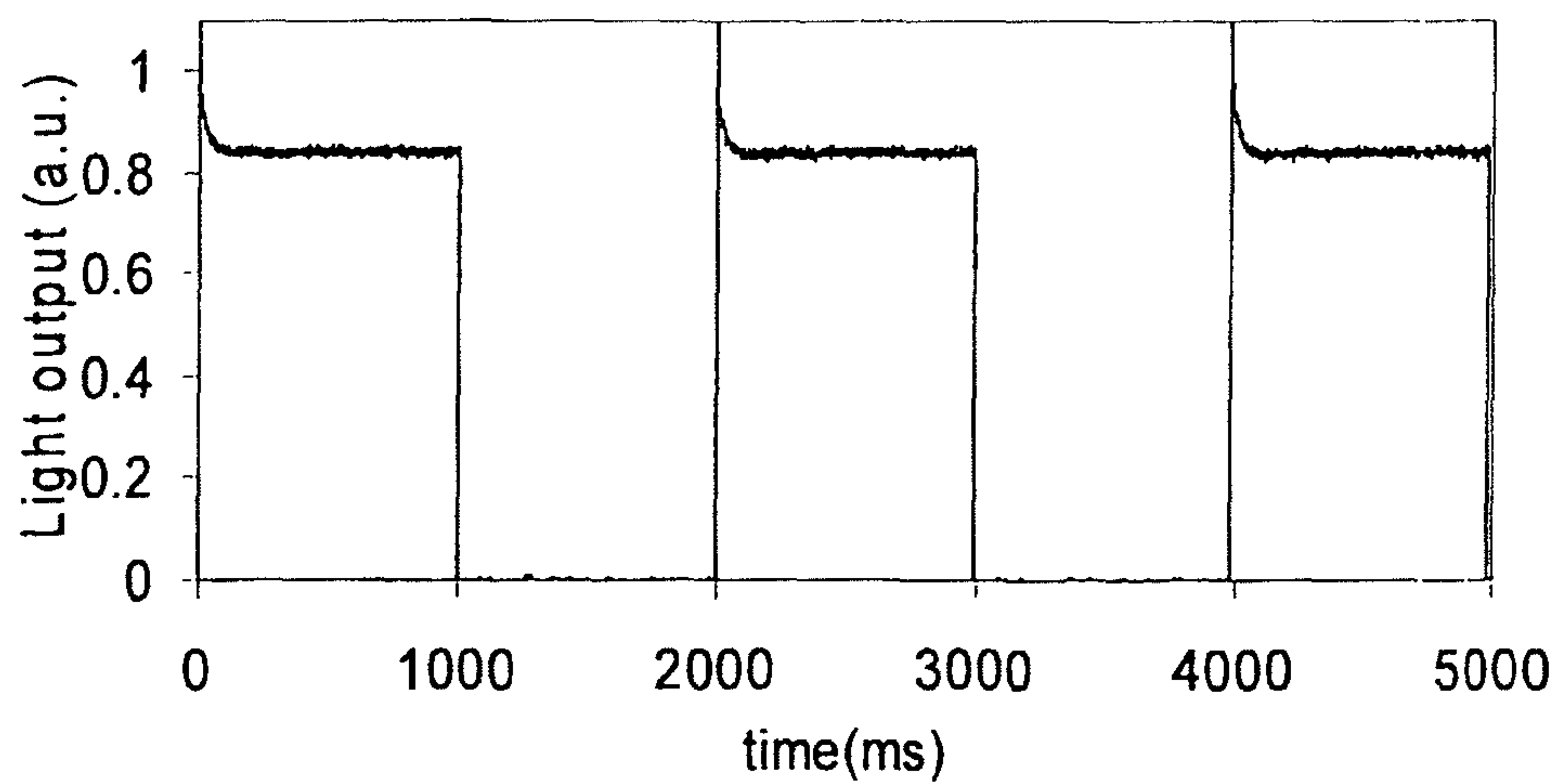
Fig. 7(c): Light output for pulsed operation of OC 1 C 10 -PPV devices
