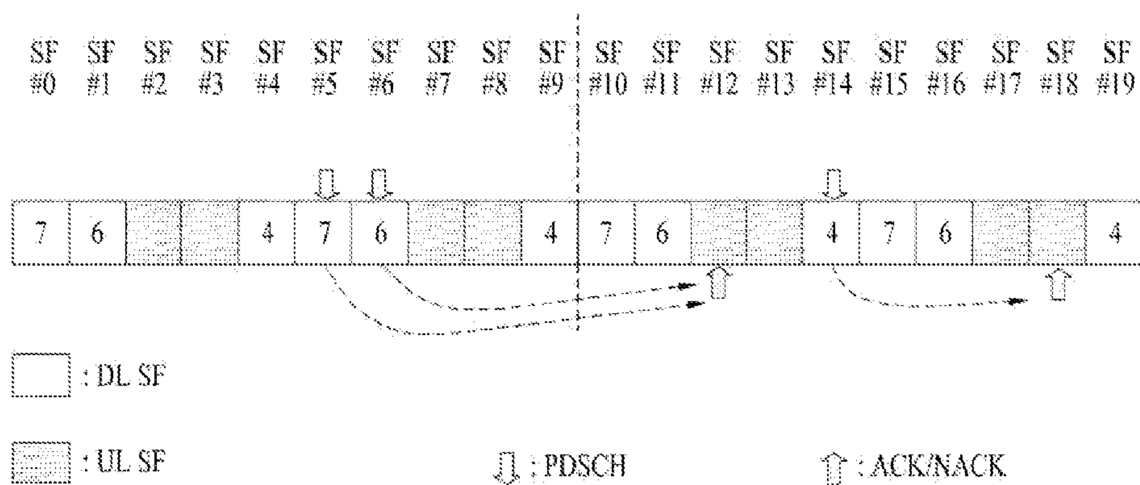
PDSCH-ACK/NACK timing (UL-DL configuration #1)
