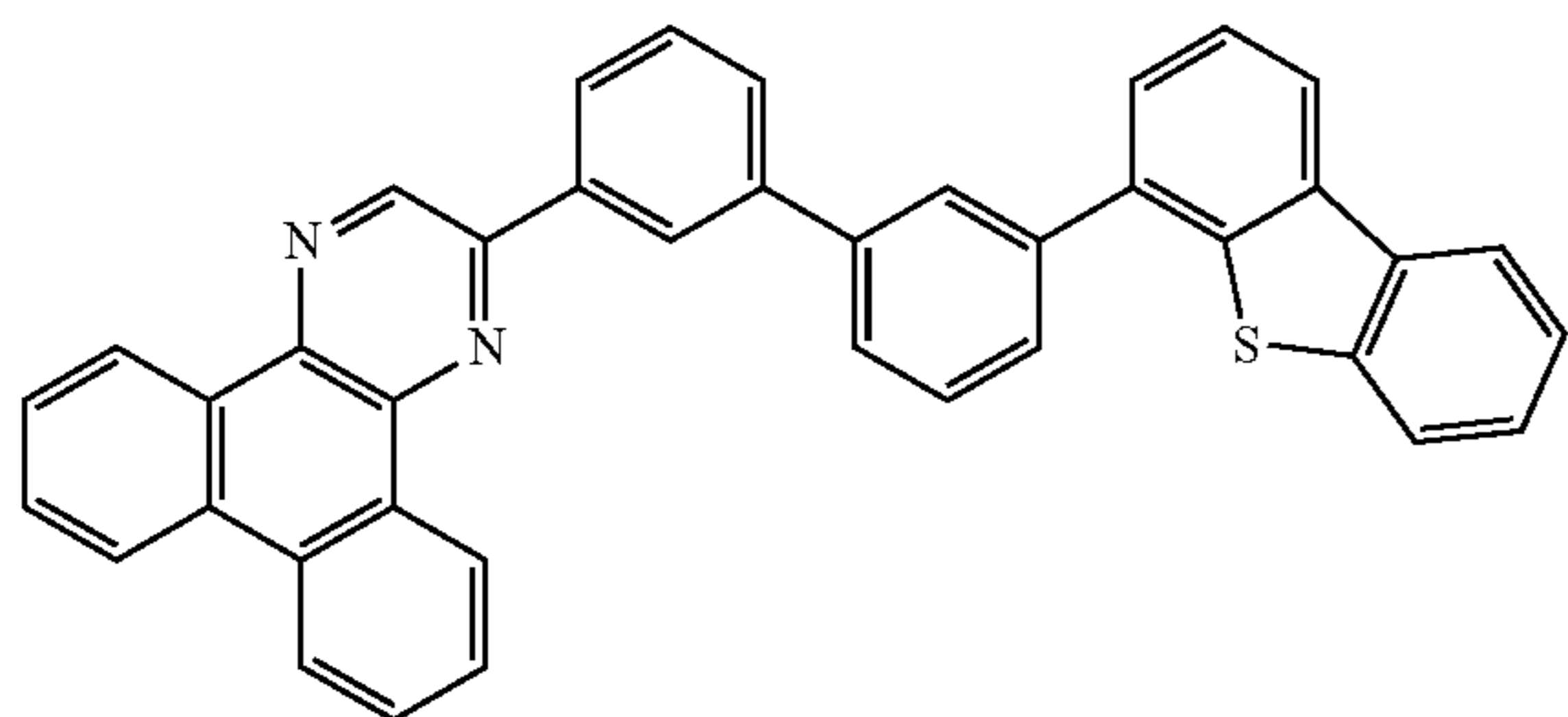
2mDBTBPDBq-II
