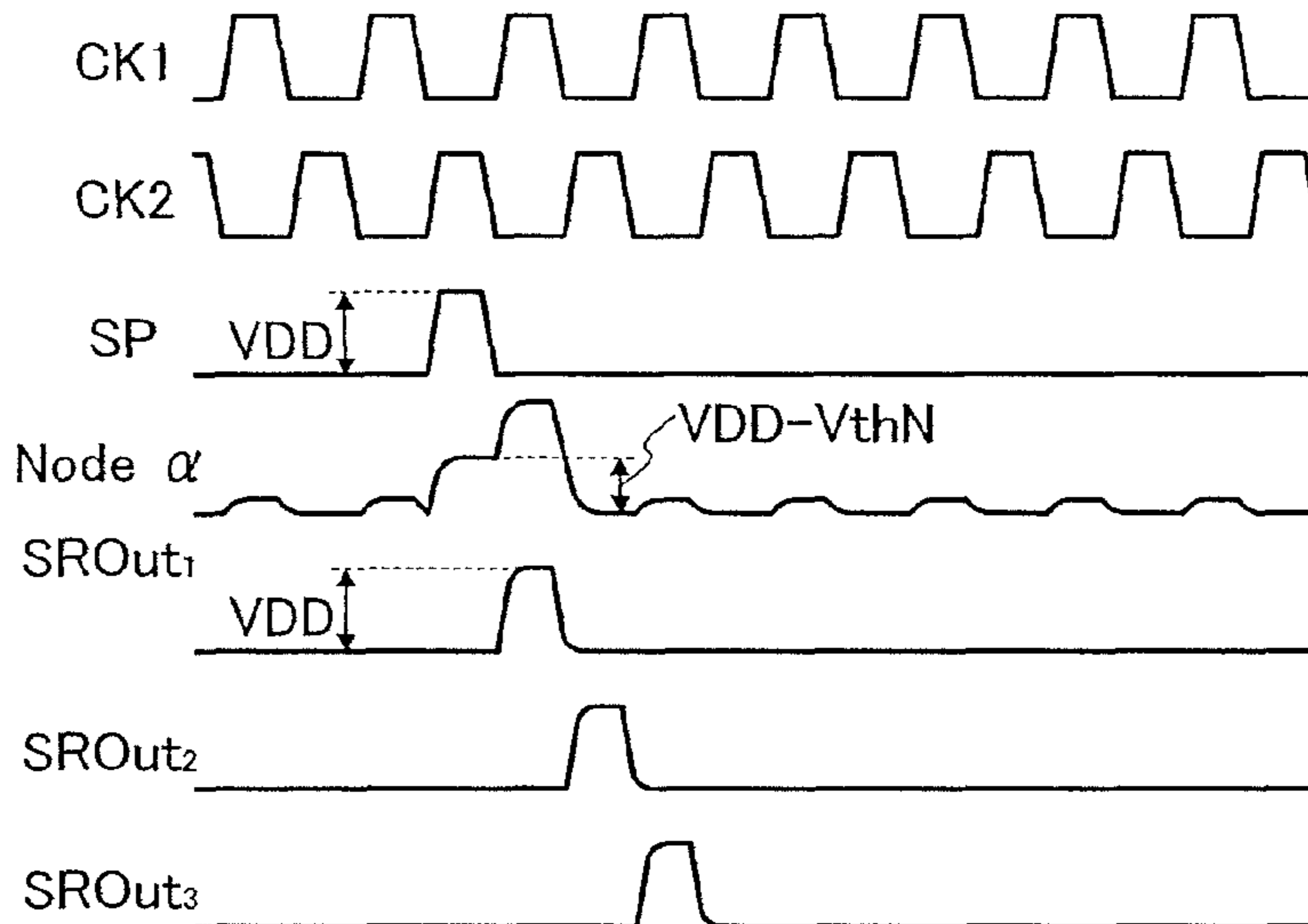
FIG. 7C PRIOR ART
