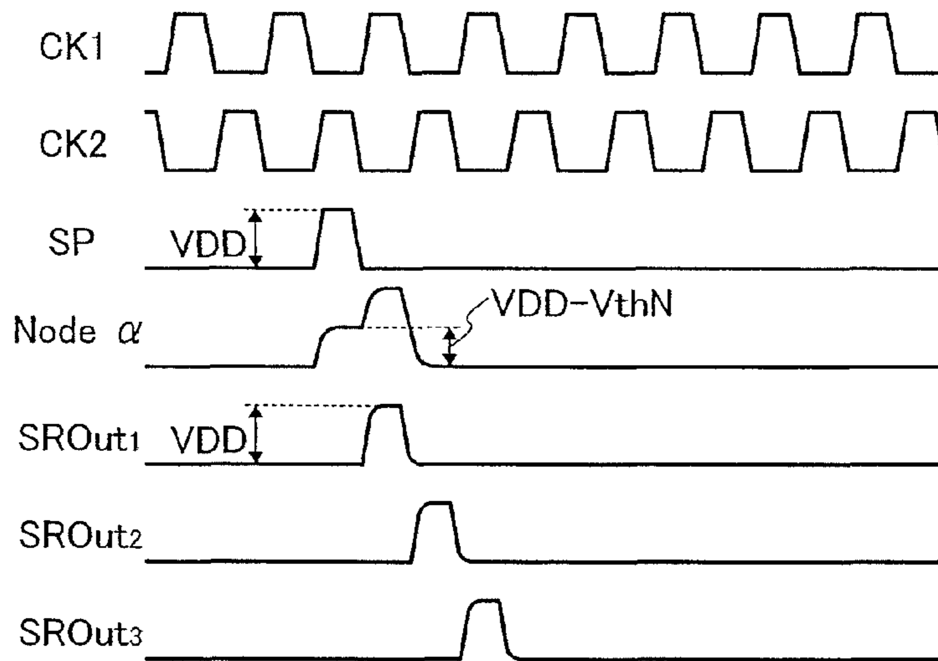
FIG. 8C PRIOR ART
