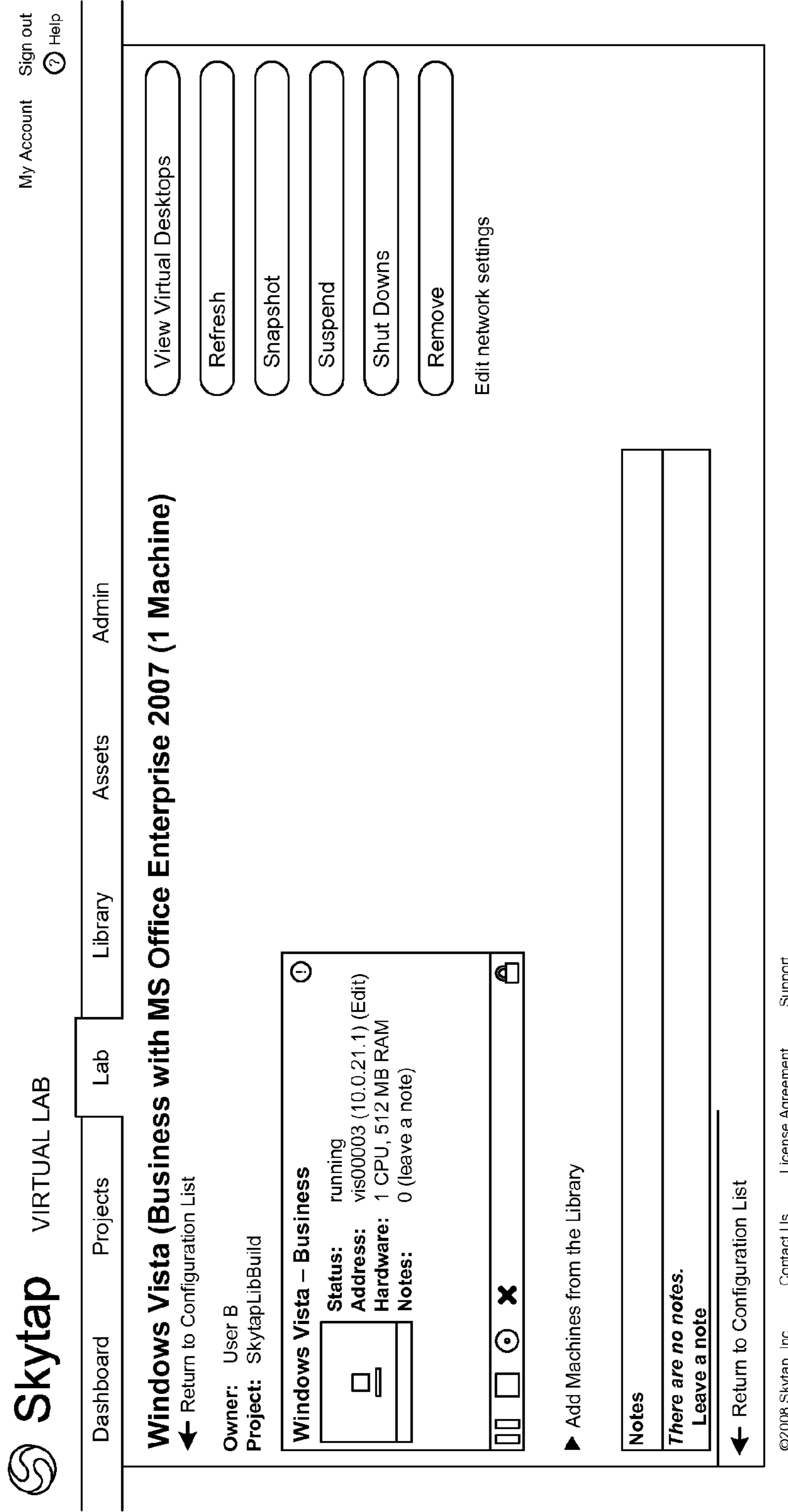
Interface showing current configuration of MTVMI.
