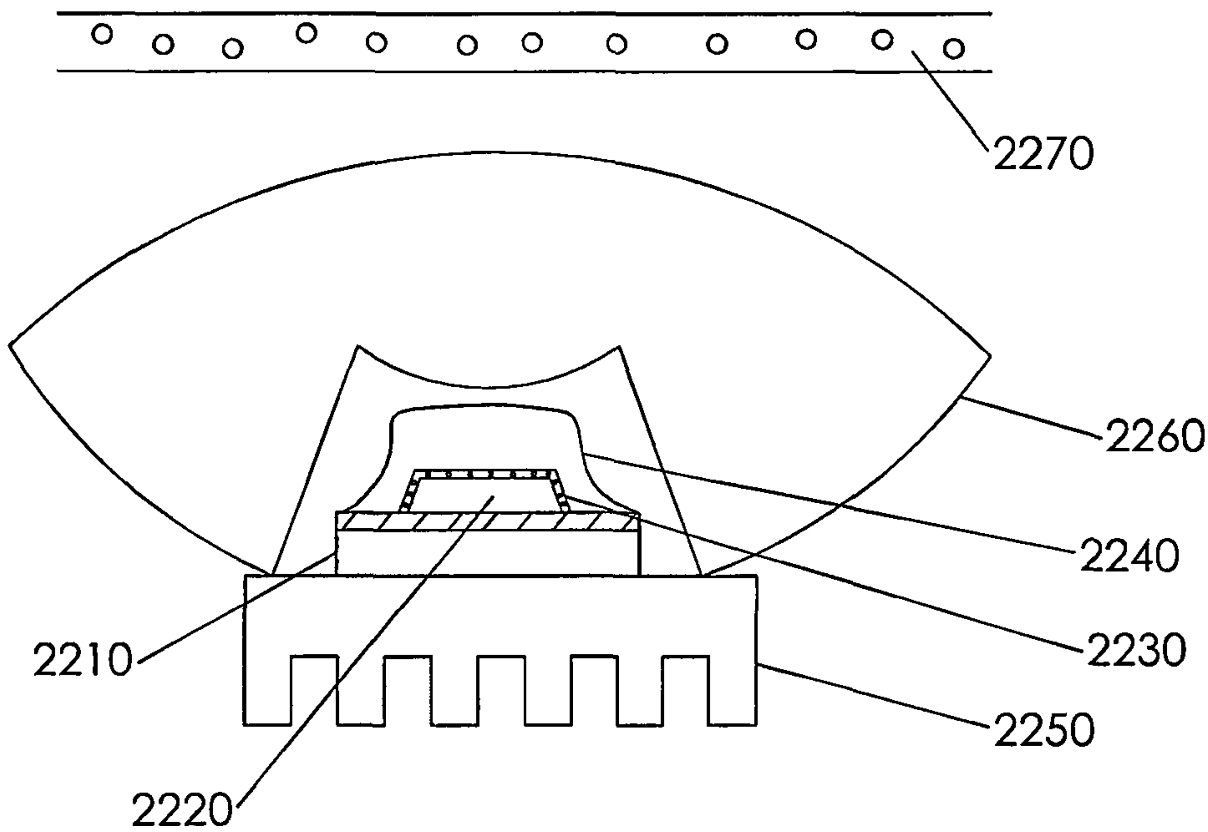
FIG. 22 (Prior Art)
