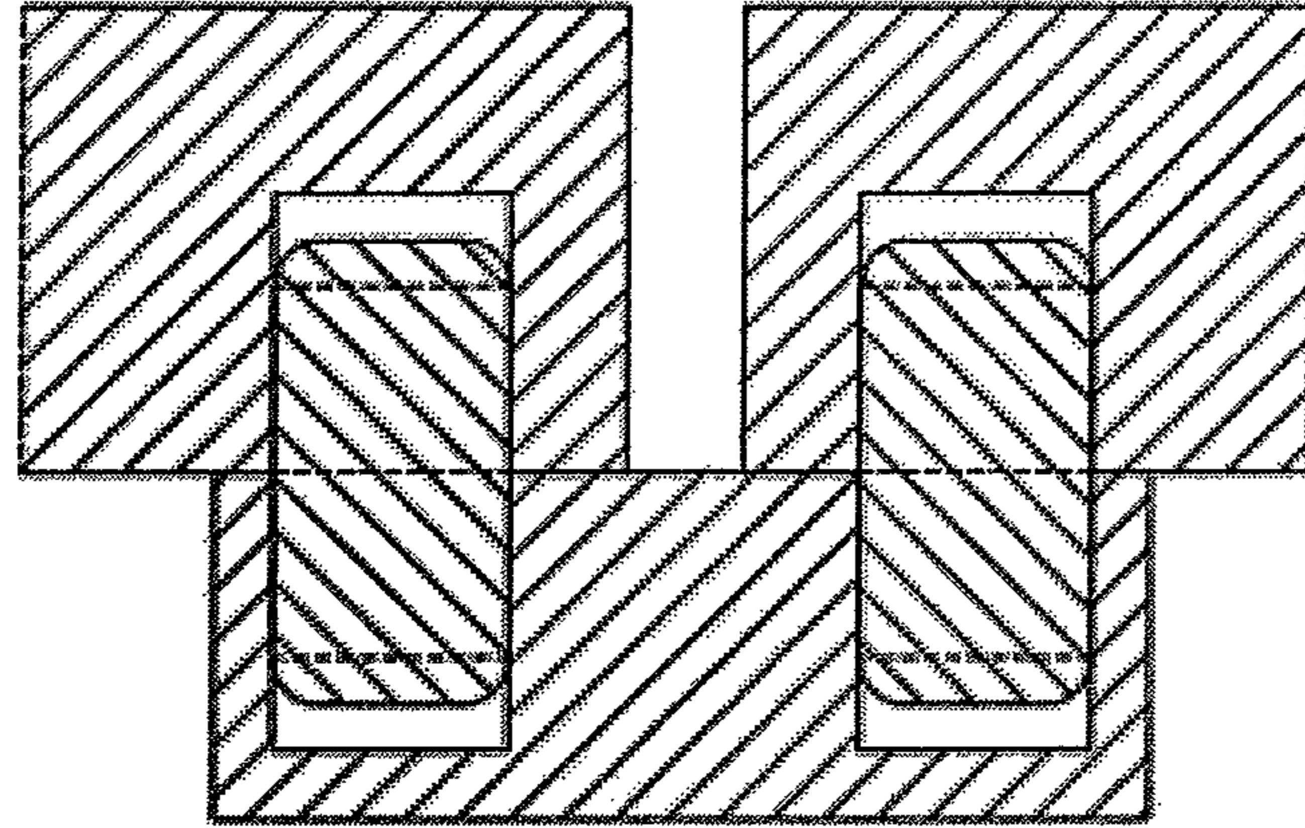
Section C-C
