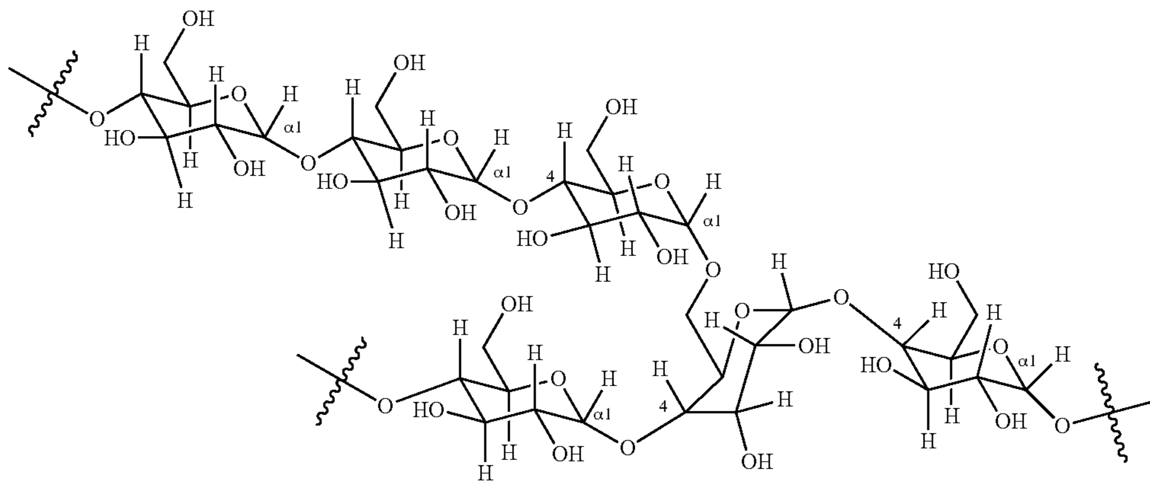
Figure 3. Representative partial structure of amylopectin
