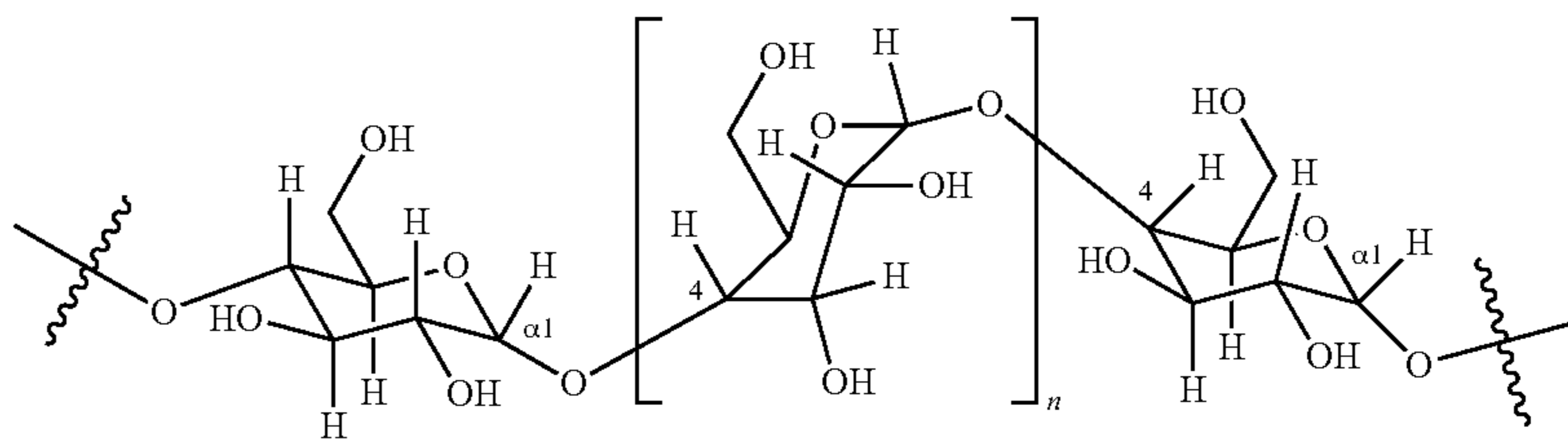
Figure 2. Representative Partial Structure of Amylose
