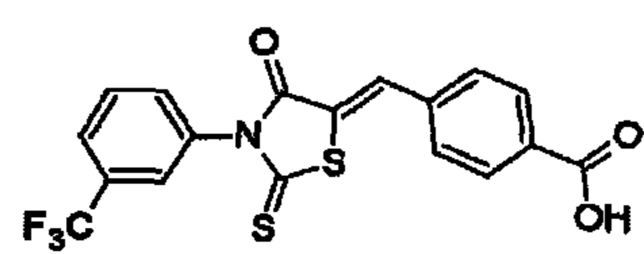
CFTR inh -172
