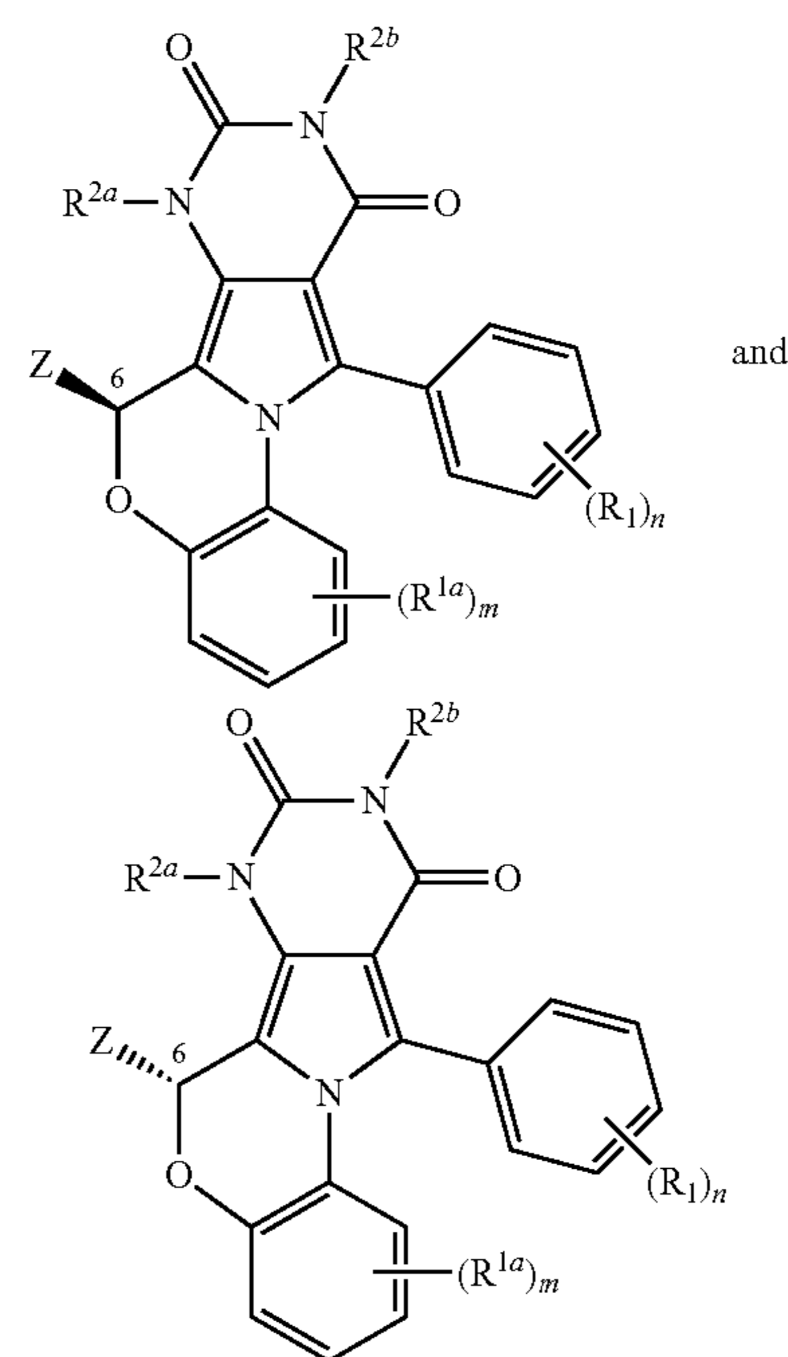
Structure (I) as Isolated Enantiomers
