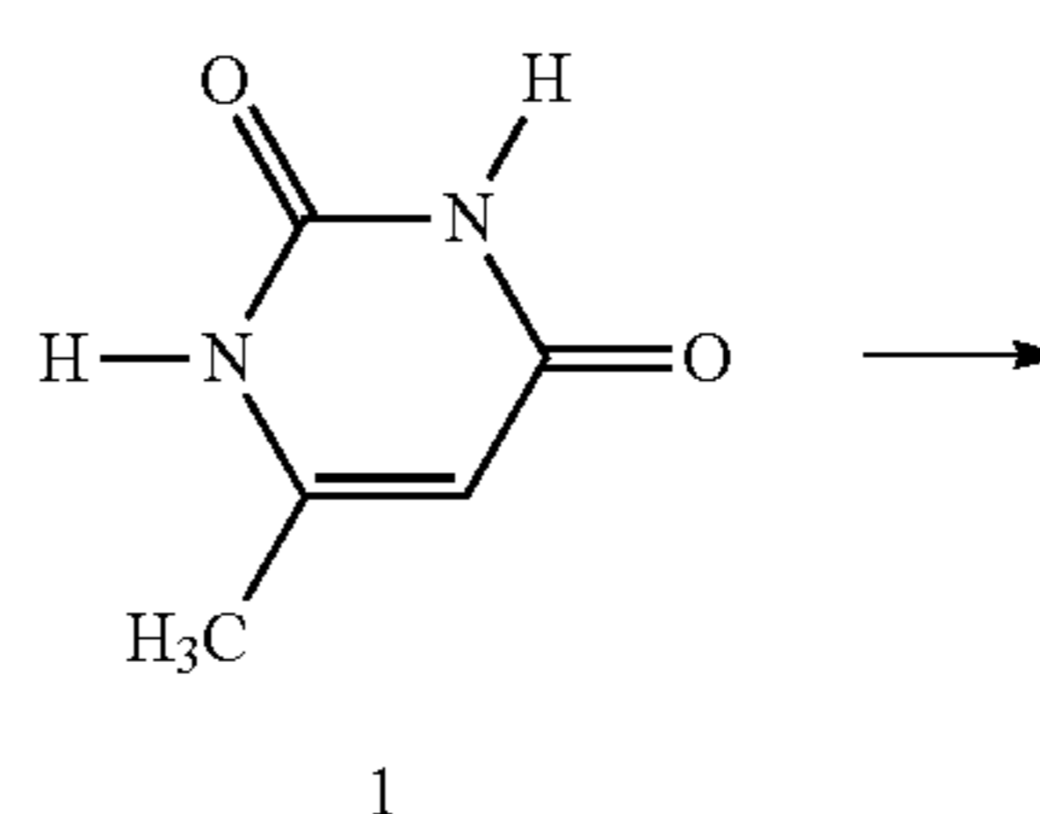
General Reaction Scheme (I)
