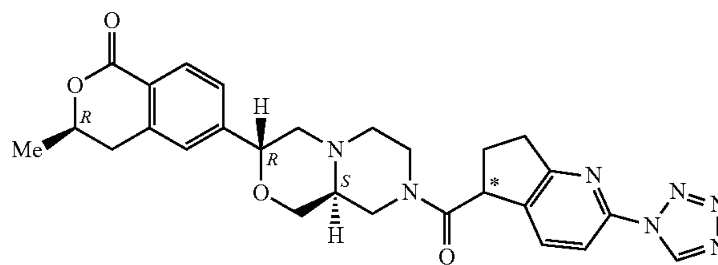
(3R)-3-methyl-6-[(3R,9aS)-8-{[2-(1H-tetrazol-1-yl)-6,7-dihydro-5H-cyclopenta[b]pyridin-5-yl]carbonyl}octahydropyrazino 2,1-c][1,4]oxazin-3-yl]-3,4-dihydro-1H-isochromen-1-one
