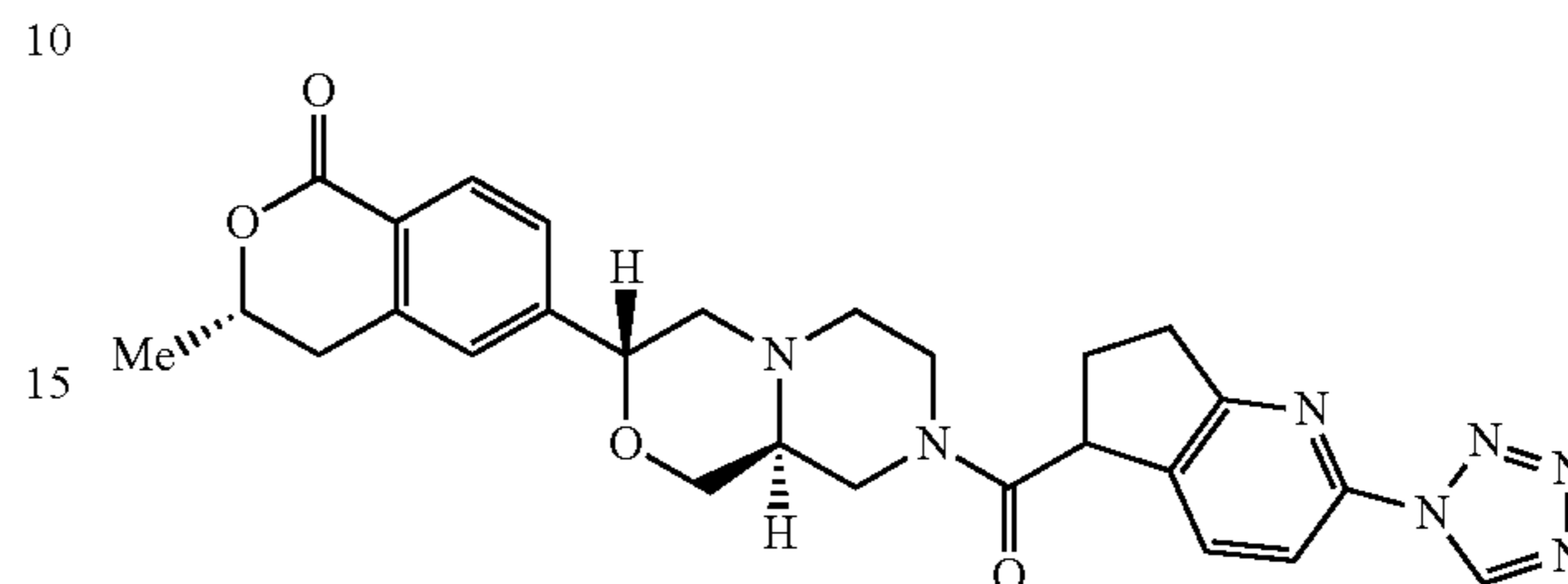
(3S)-3-methyl-6-[(3R,9aS)-8-{[2-(1H-tetrazol-1-yl)-6,7-dihydro-5H-cyclopenta[b]pyridin-5-yl]carbonyl}octahydropyrazino[2,1-c][1,4]oxazin-3-yl]-3,4-dihydro-1H-isochromen-1-one
