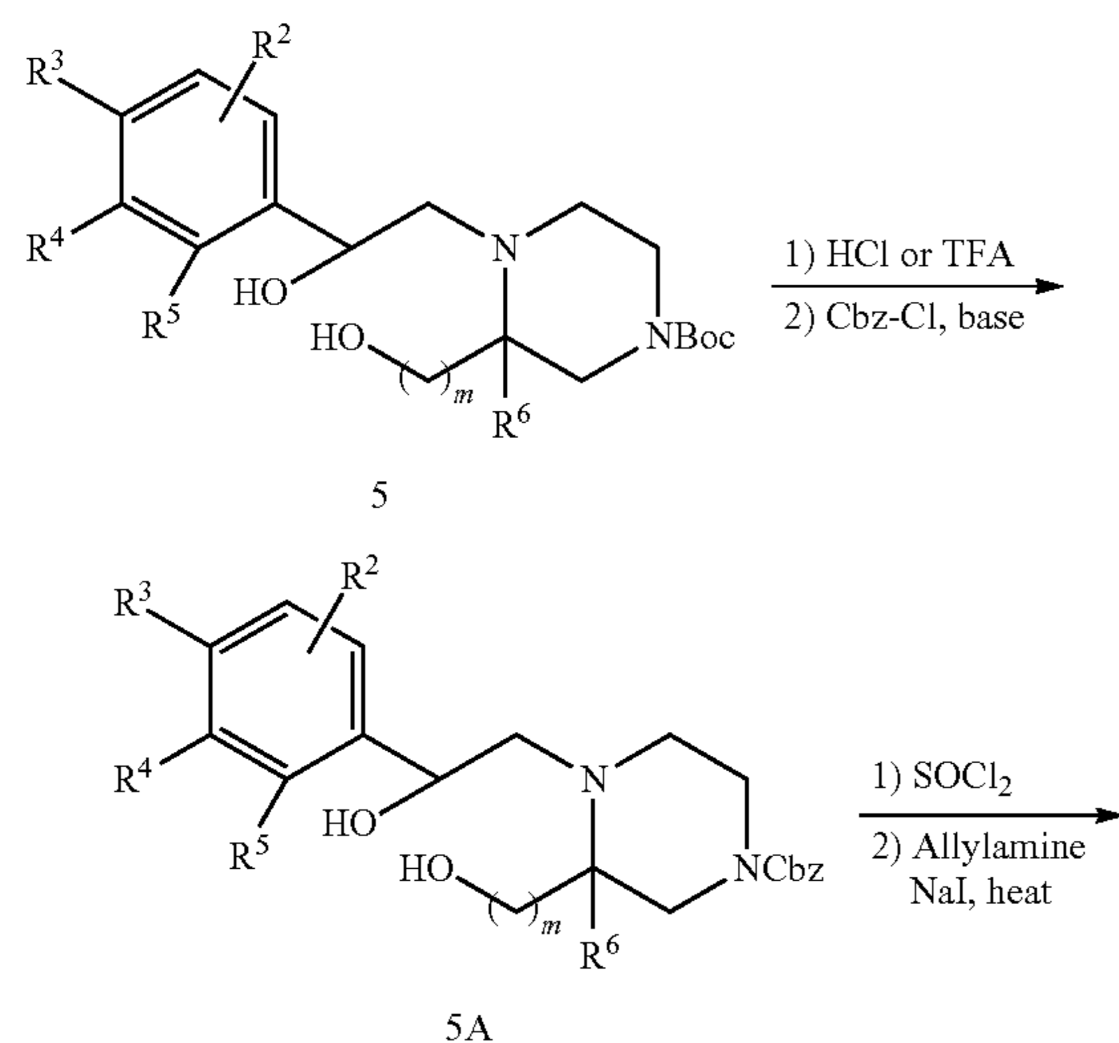
Scheme 4
