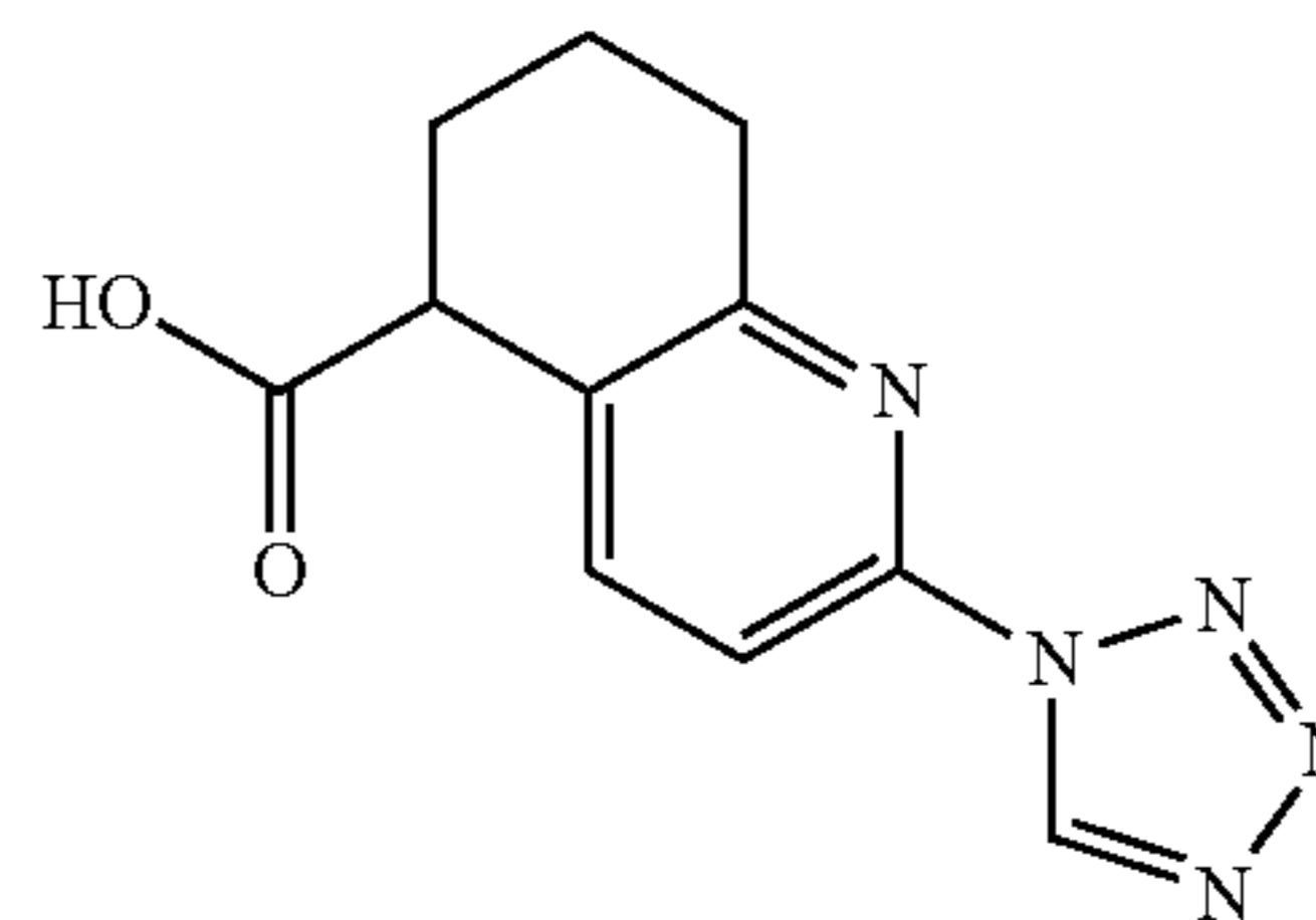
2-(1H-tetrazol-1-yl)-5,6,7,8-tetrahydroquinoline-5-carboxylic acid
