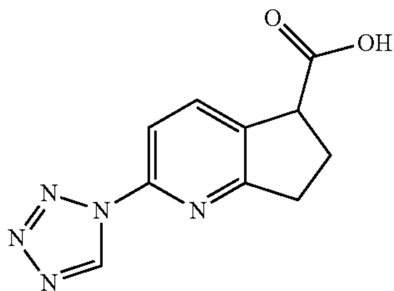
2-(1H-tetrazol-1-yl)-6,7-dihydro-5H-cyclopenta[b]pyridine-5-carboxylic acid
