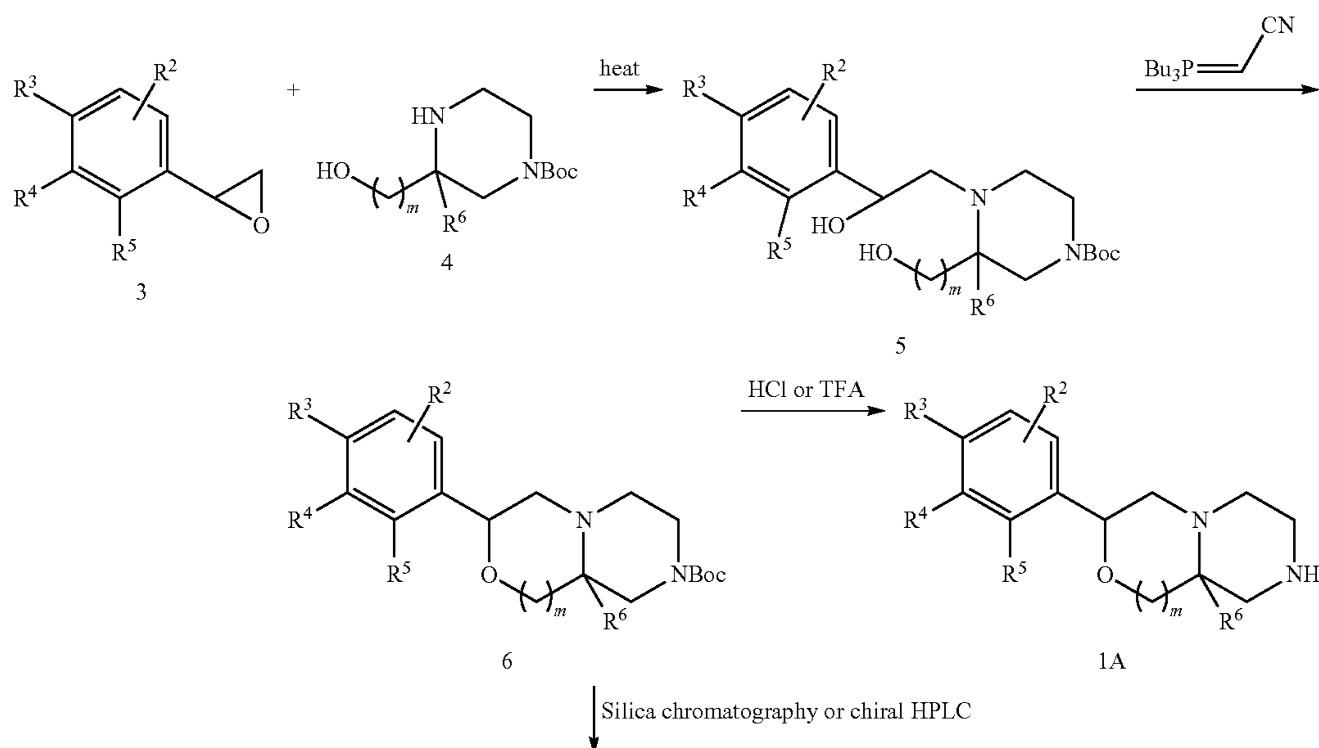
Scheme 2
