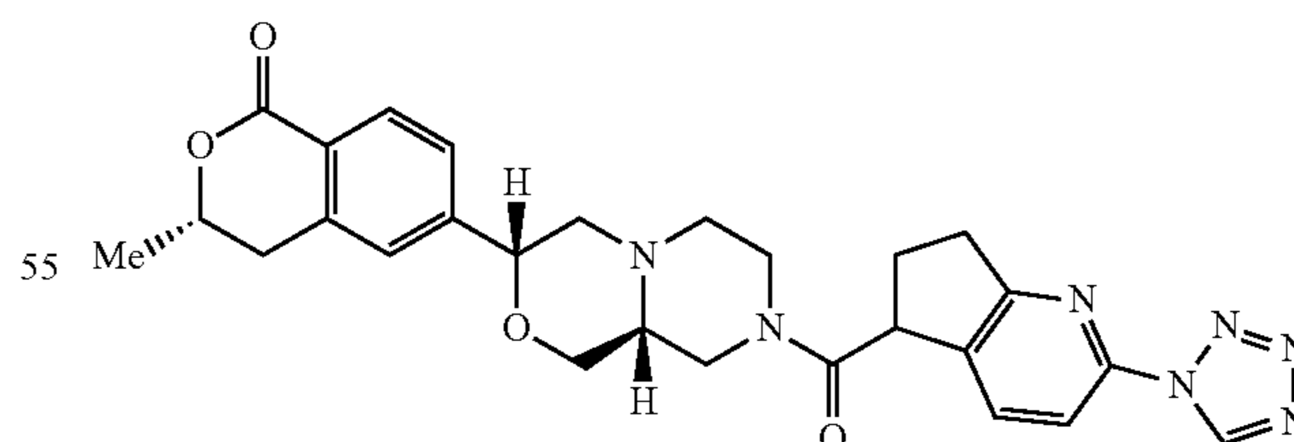
(3S)-3-methyl-6-[(3R,9aR)-8-{[2-(1H-tetrazol-1-yl)-6,7-dihydro-5H-cyclopenta[b]pyridin-5-yl]carbonyl}octahydropyrazino[2,1-c][1,4]oxazin-3-yl]-3,4-dihydro-1H-isochromen-1-one
