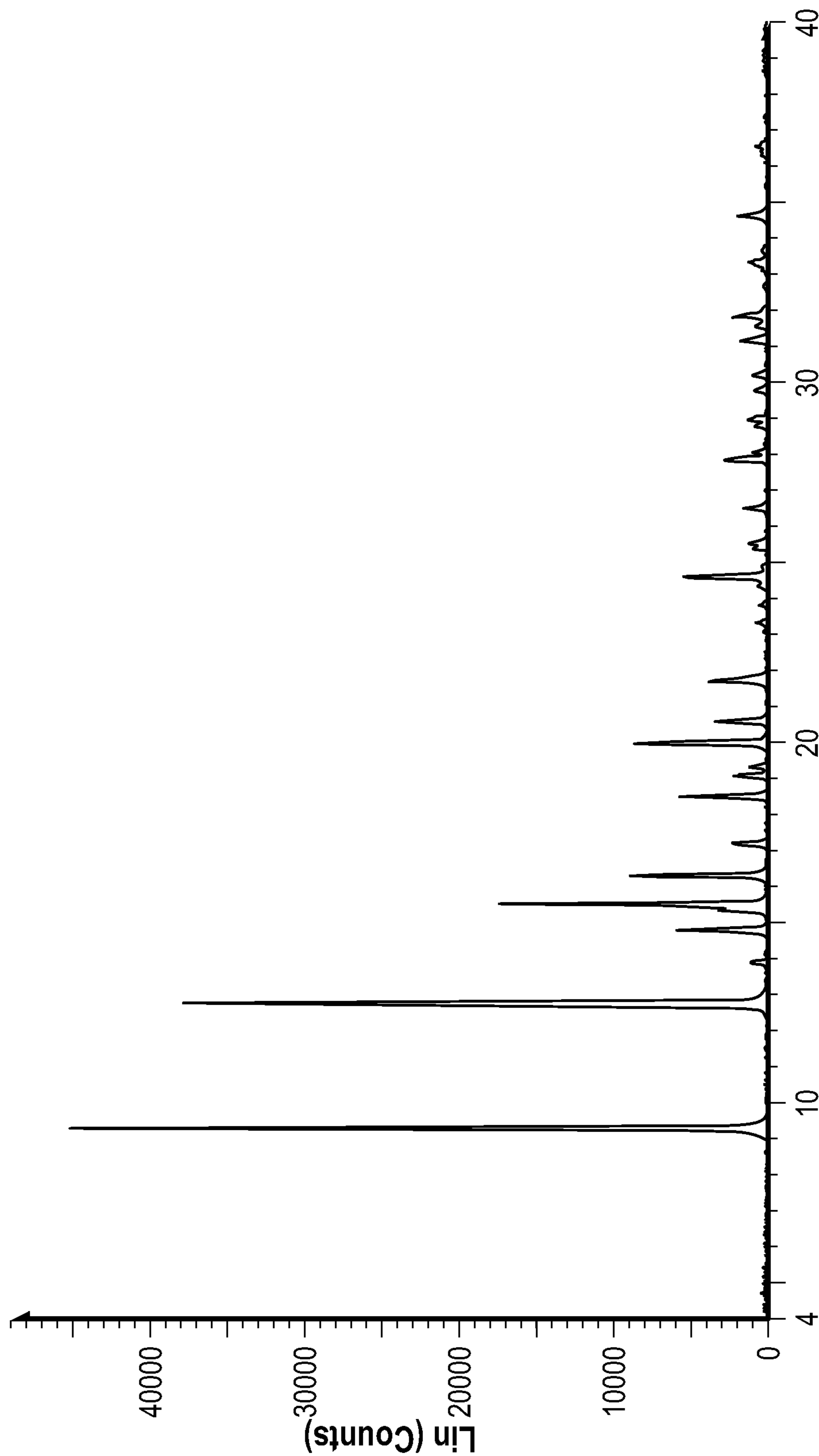
2-Theta - Scale XRPD pattern of Oxymorphone HCl Form E FIG. 5
