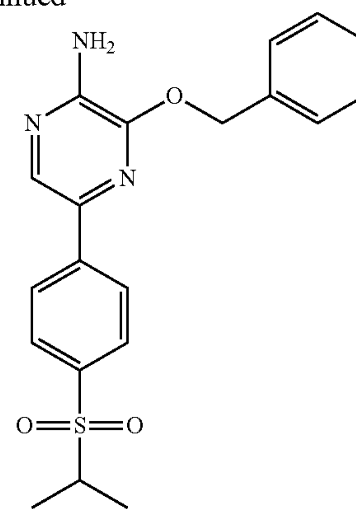
Compound V-9
