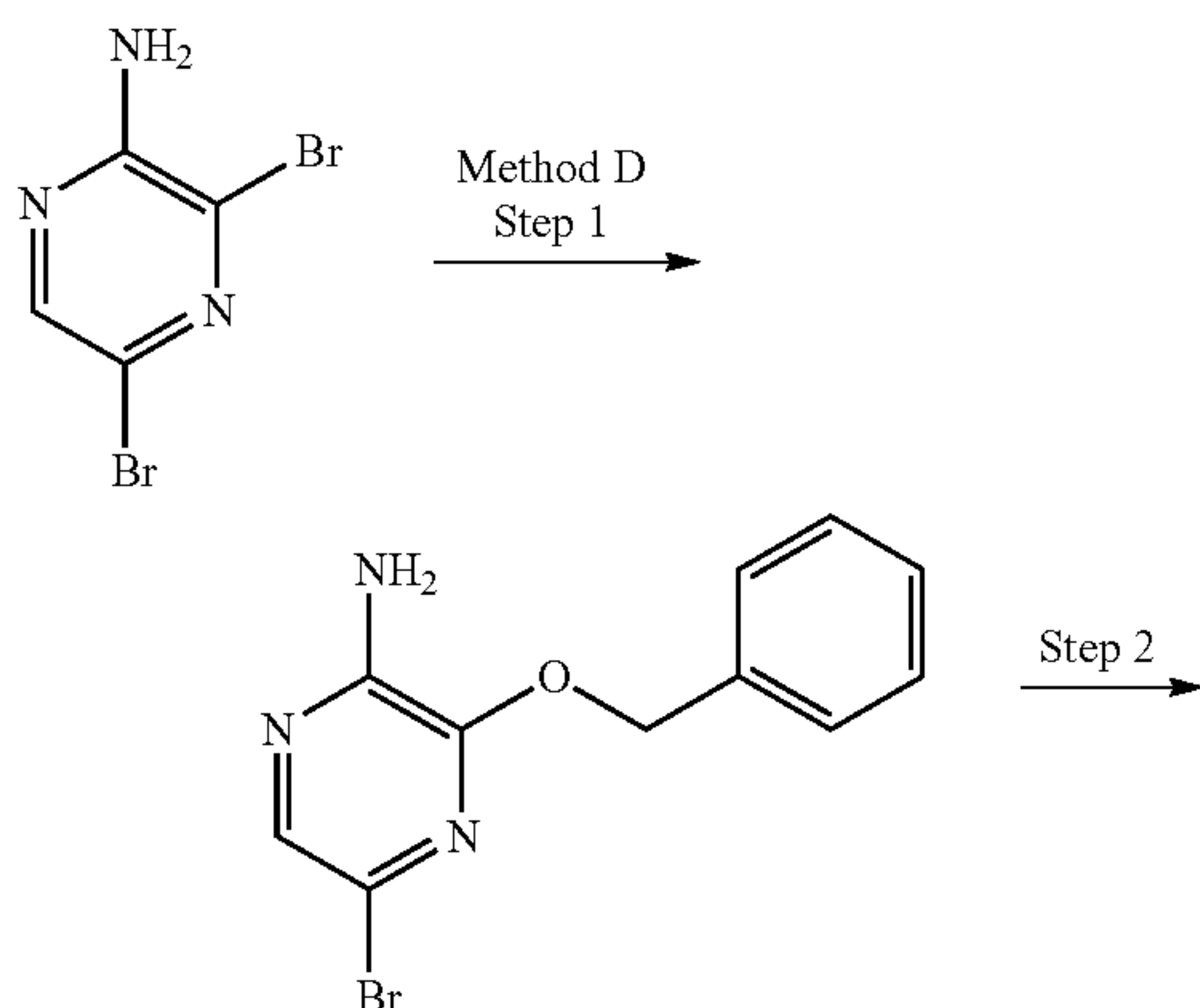
SCHEME IV
