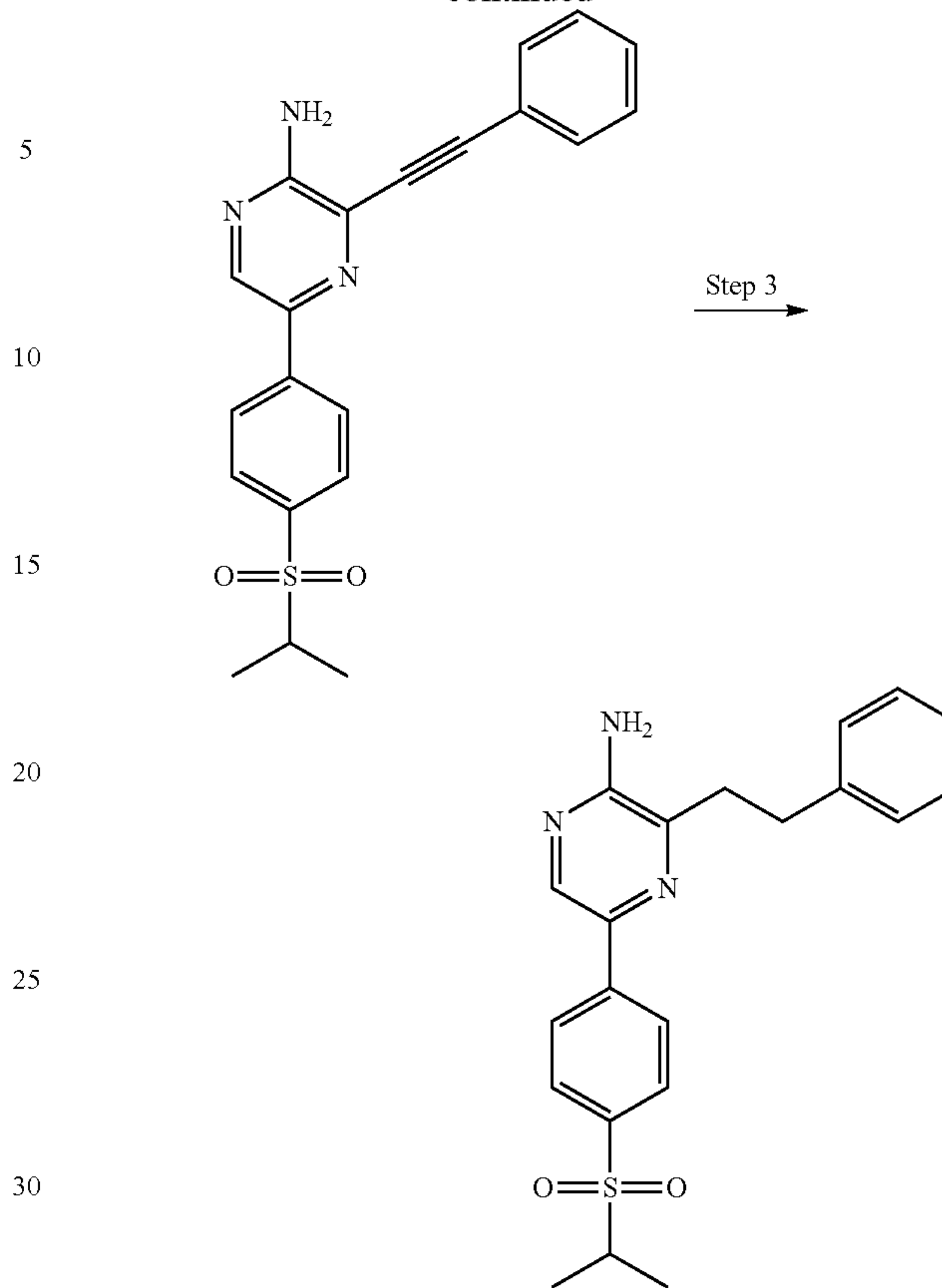
Compound V-11
