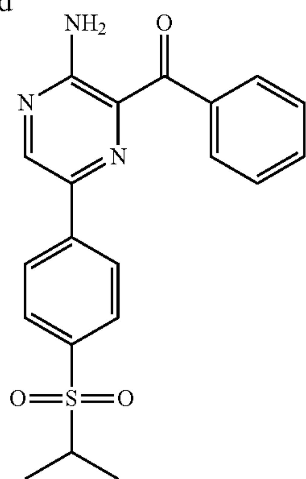
Compound V-12
