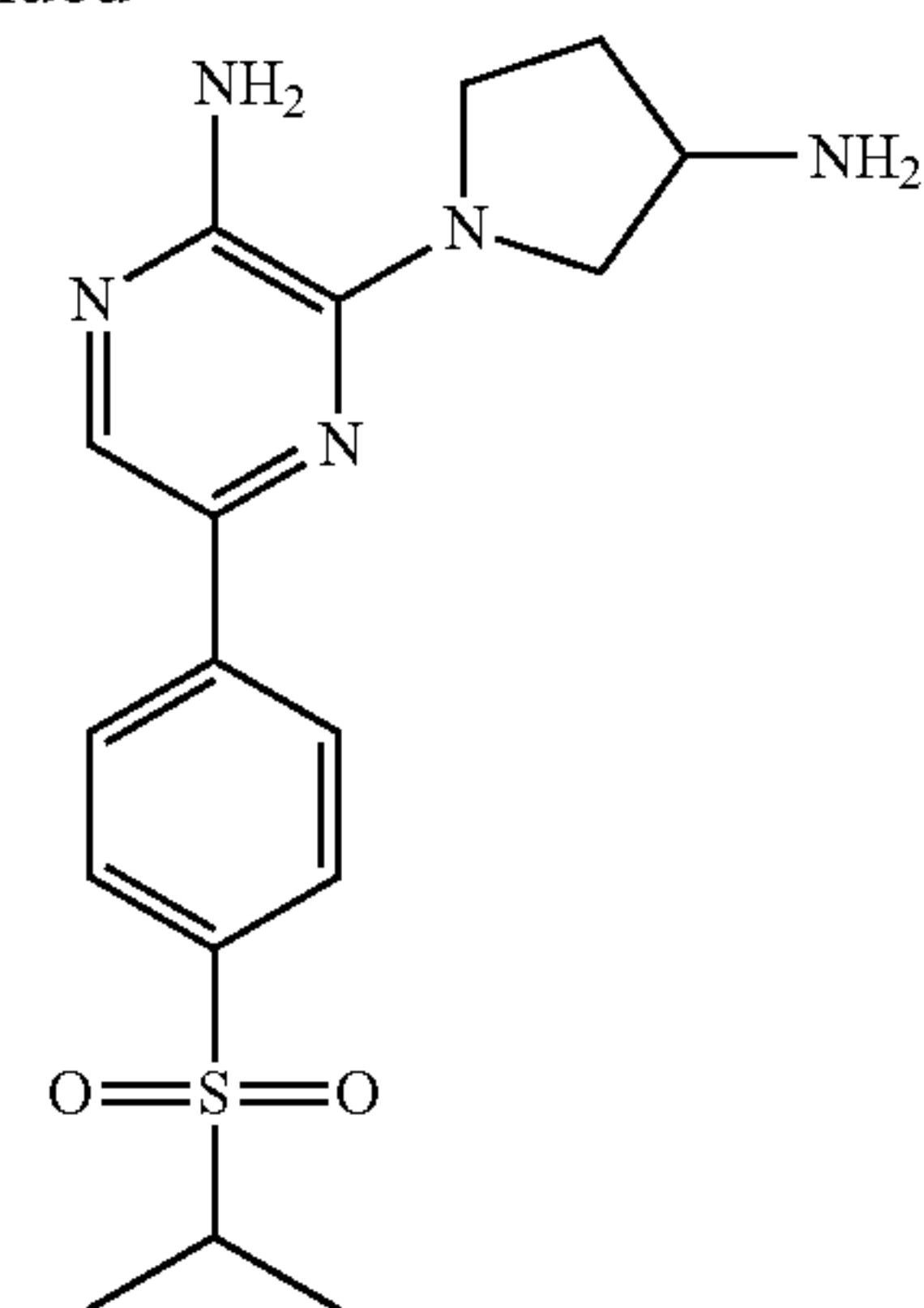
Compound V-2
