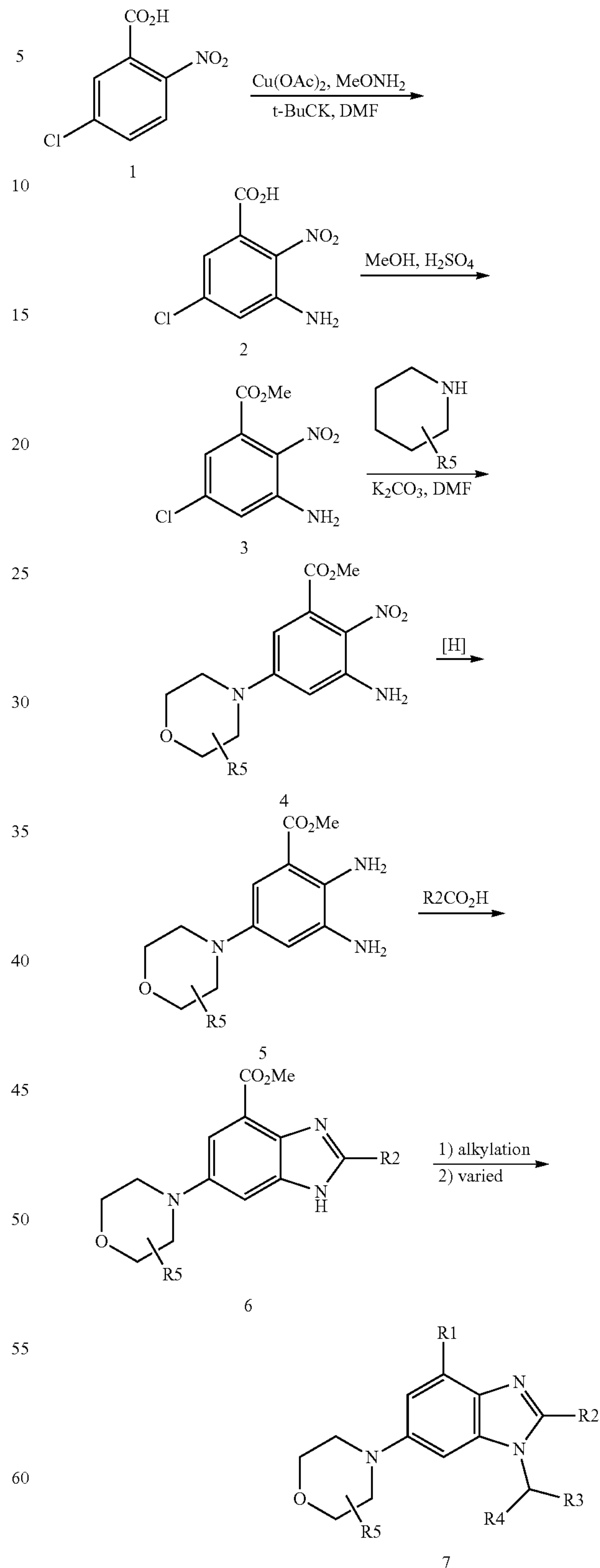
Scheme VII
