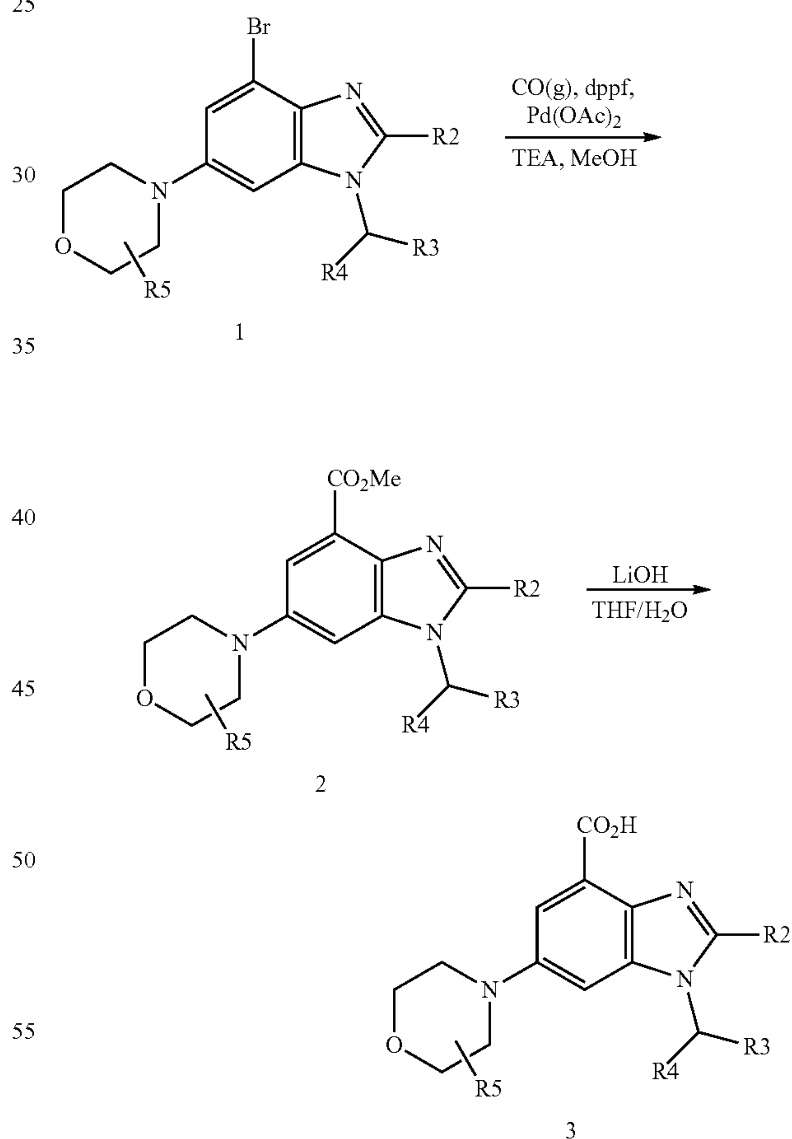
Scheme V
