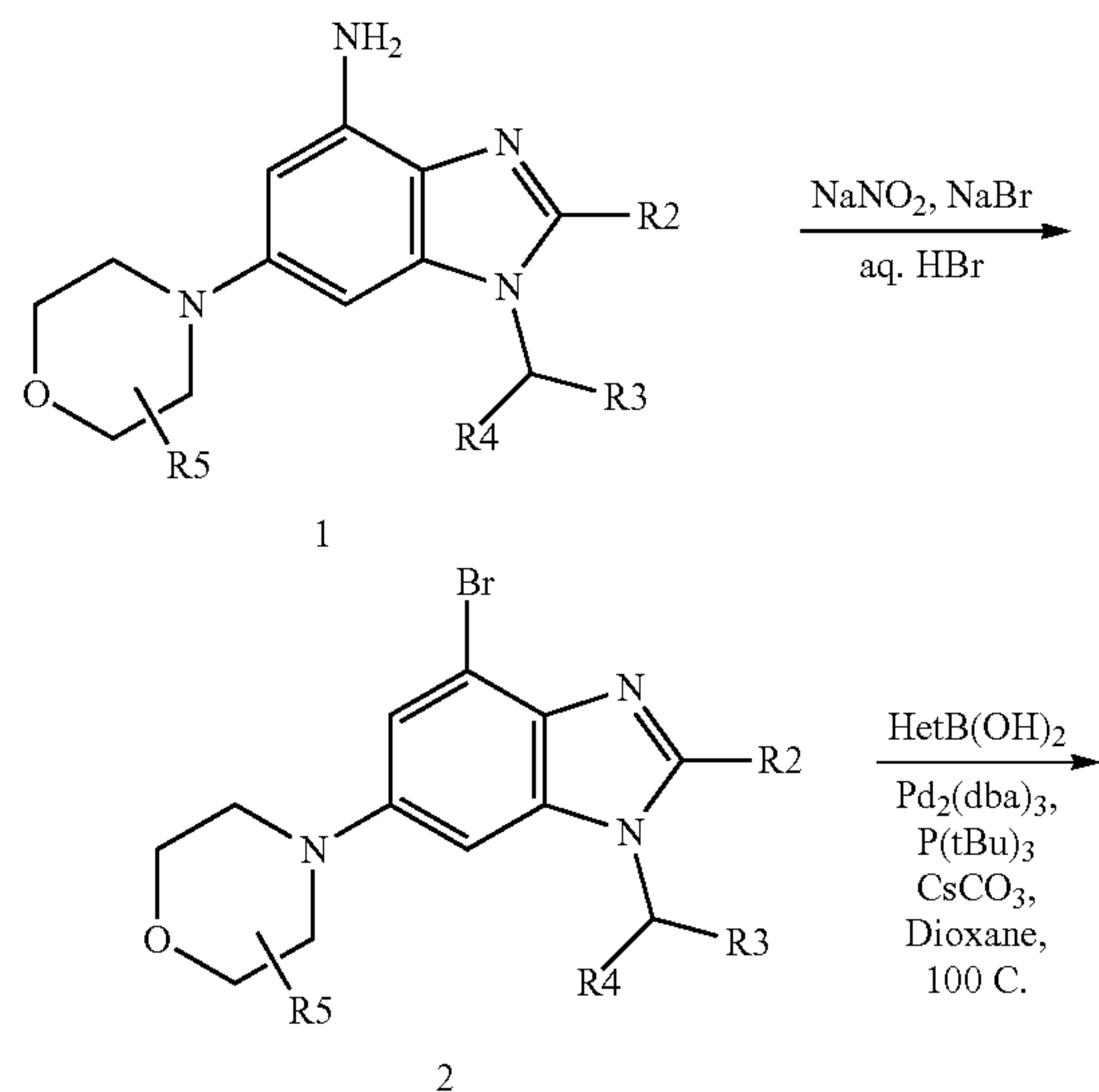
Scheme IV
