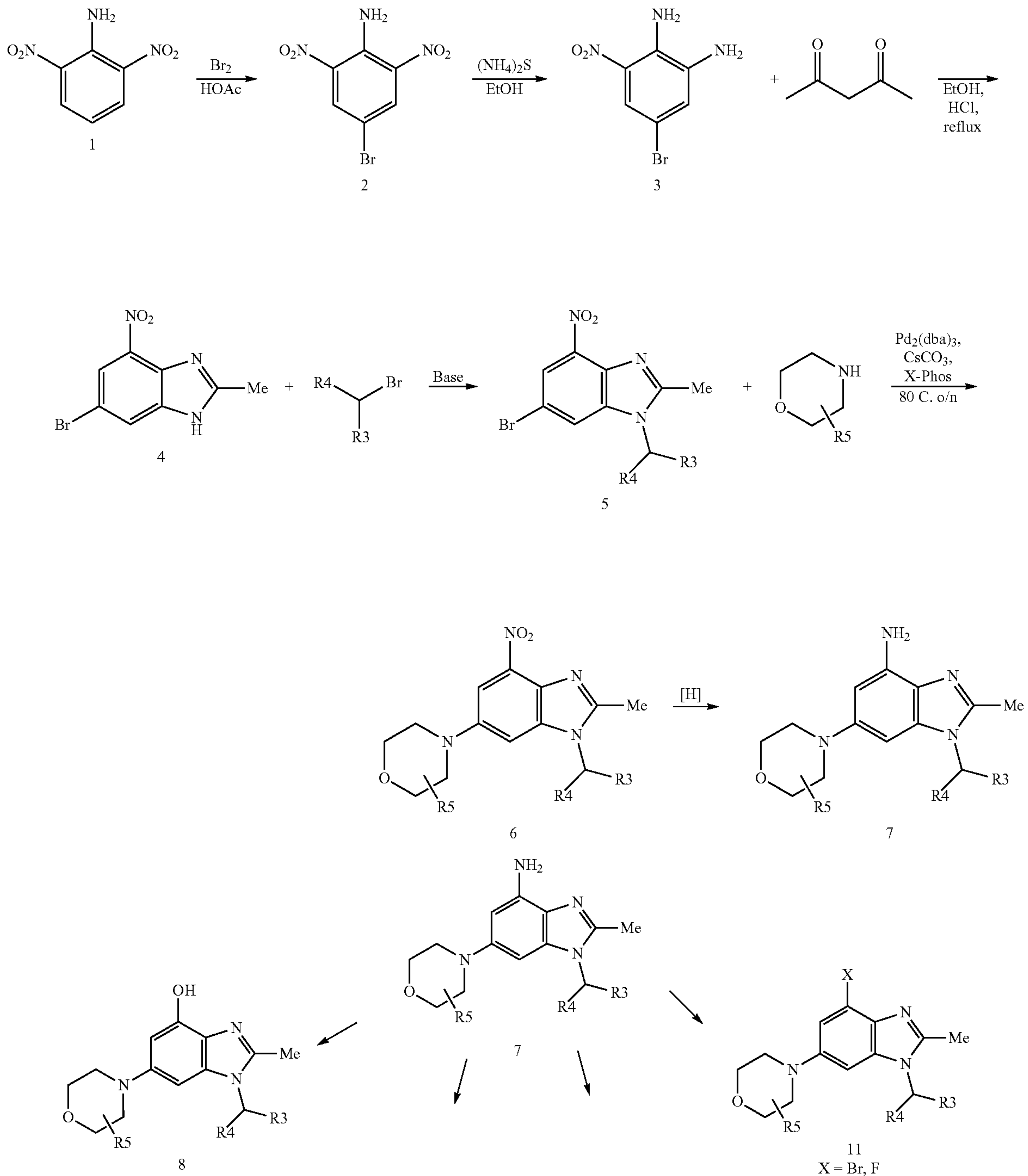
Scheme 1 (R2 = Me)
