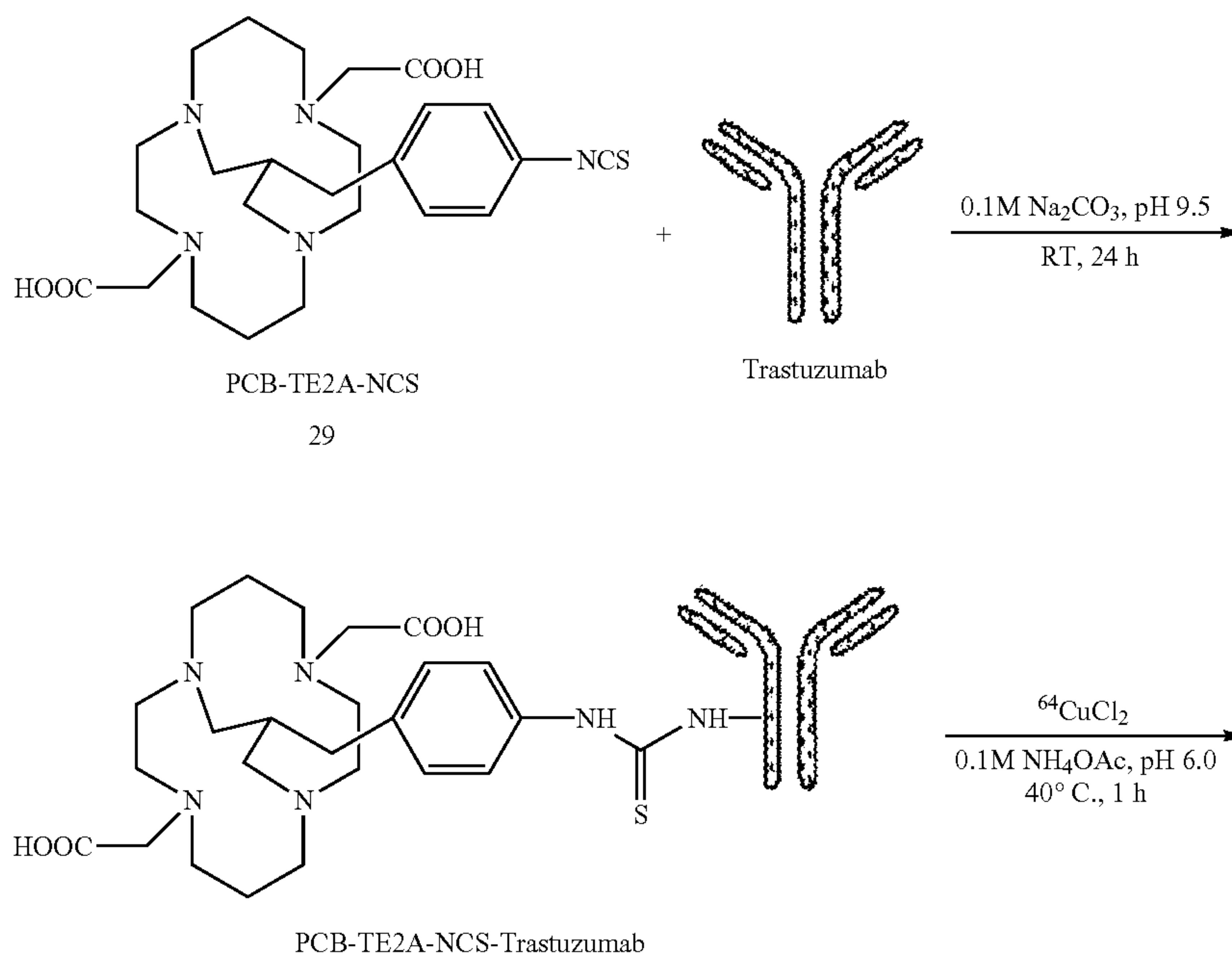
[Scheme 16]
