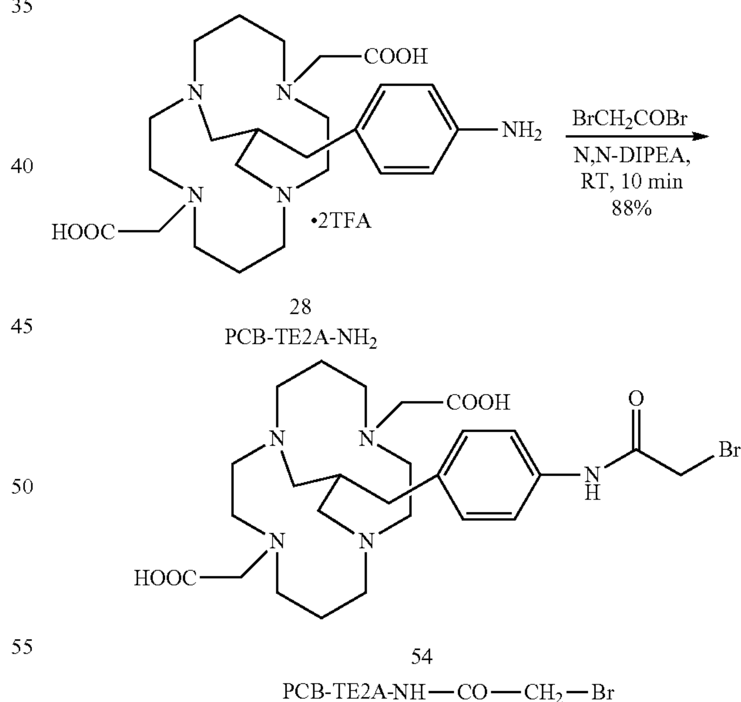
[Scheme 22]
