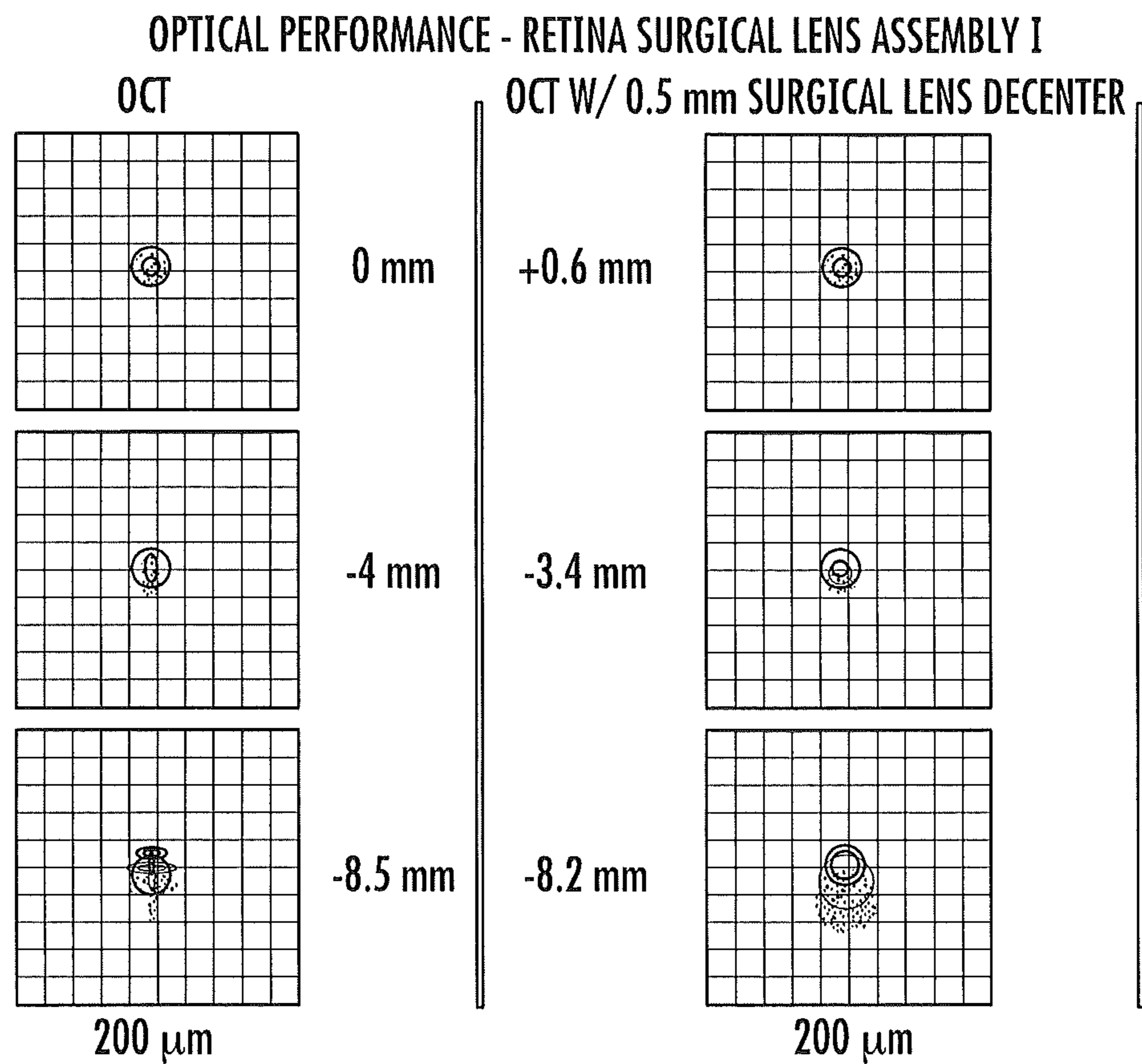
LOW MAG. SINGLET OPTICAL PERFORMANCE SUMMARY
