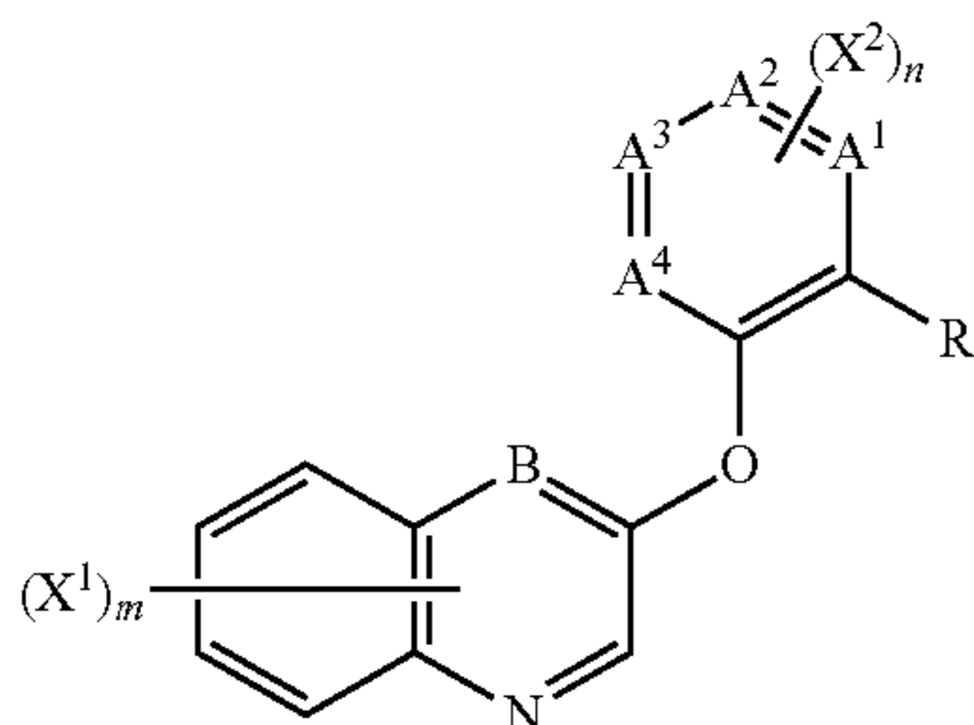
[Chemical Formula 13]
