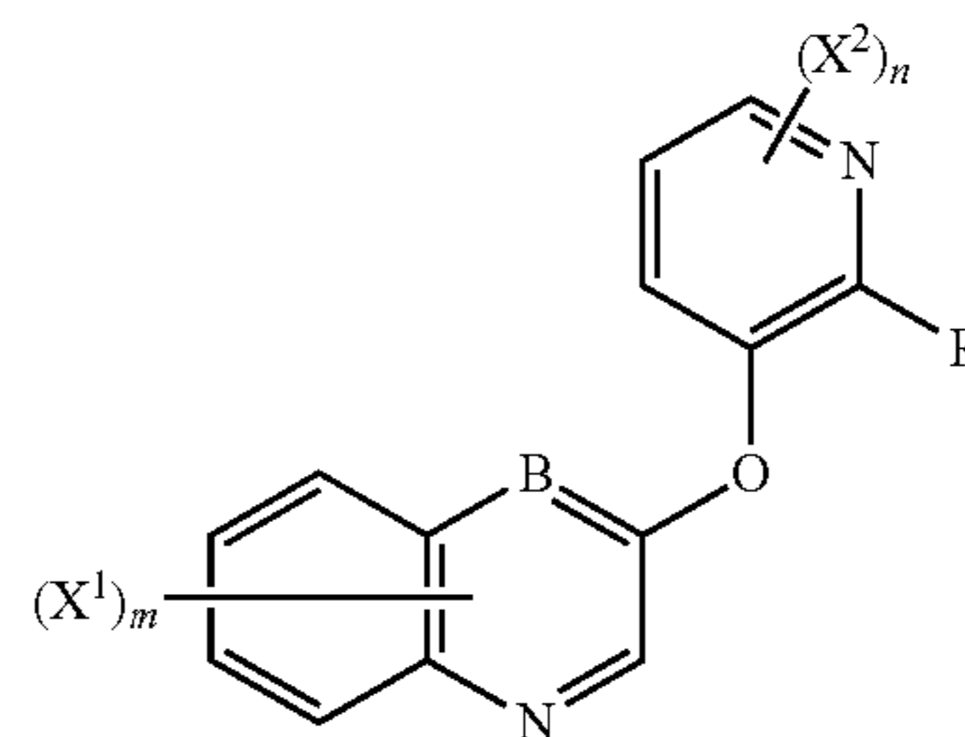
[Chemical Formula 8]
