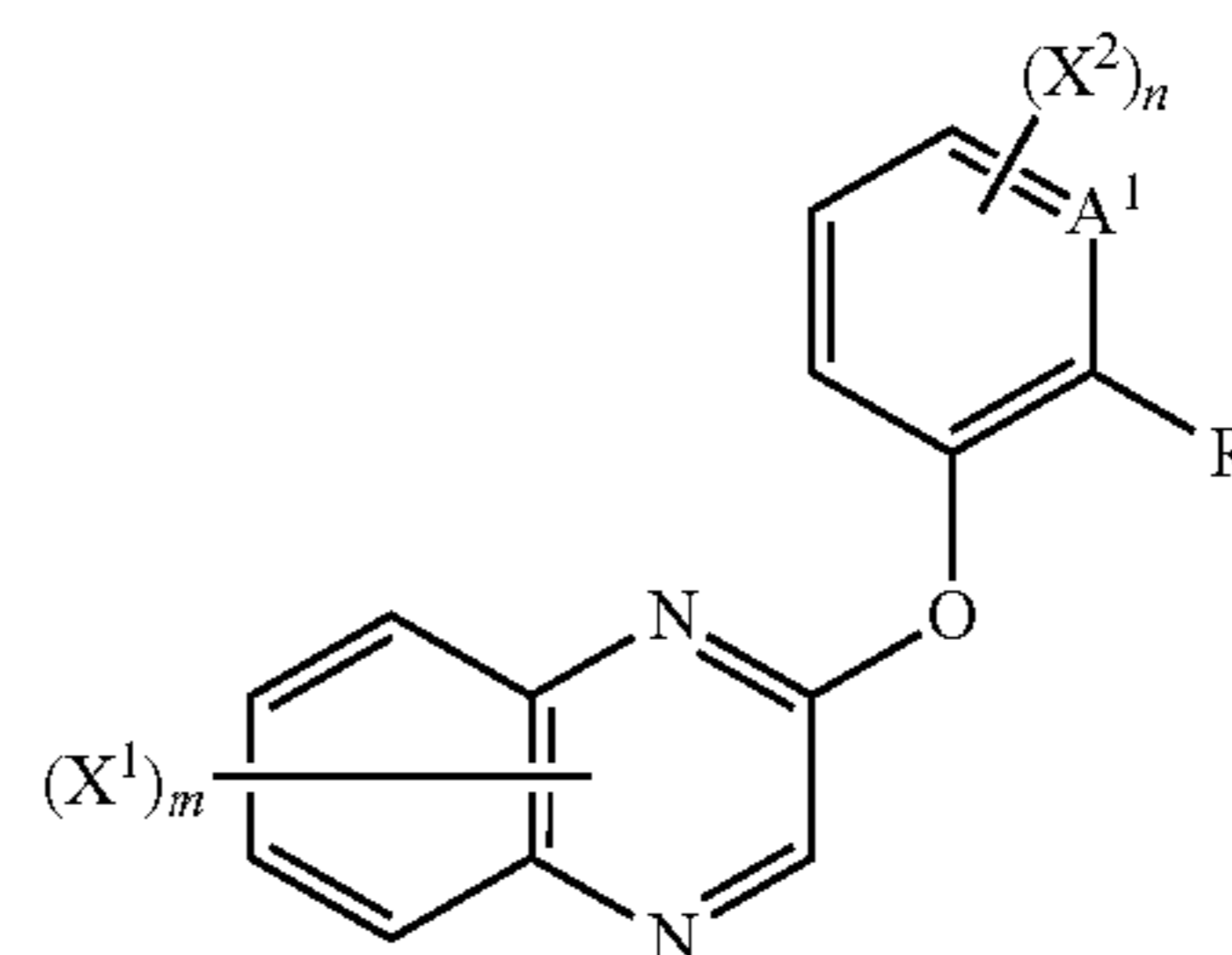
[Chemical Formula 16]
