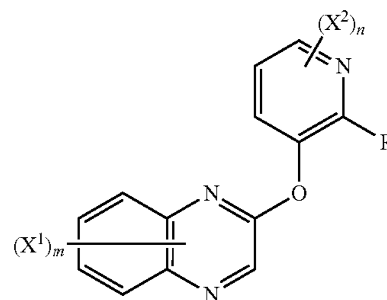
[Chemical Formula 17]
