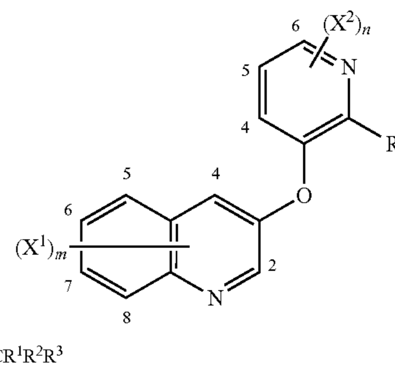
[Chemical Formula 50]
