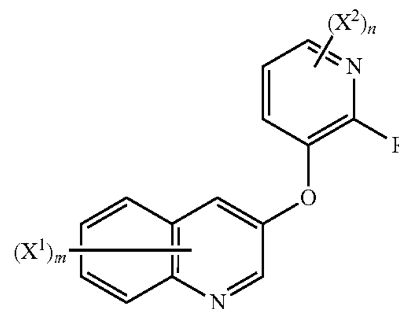
[Chemical Formula 15]
