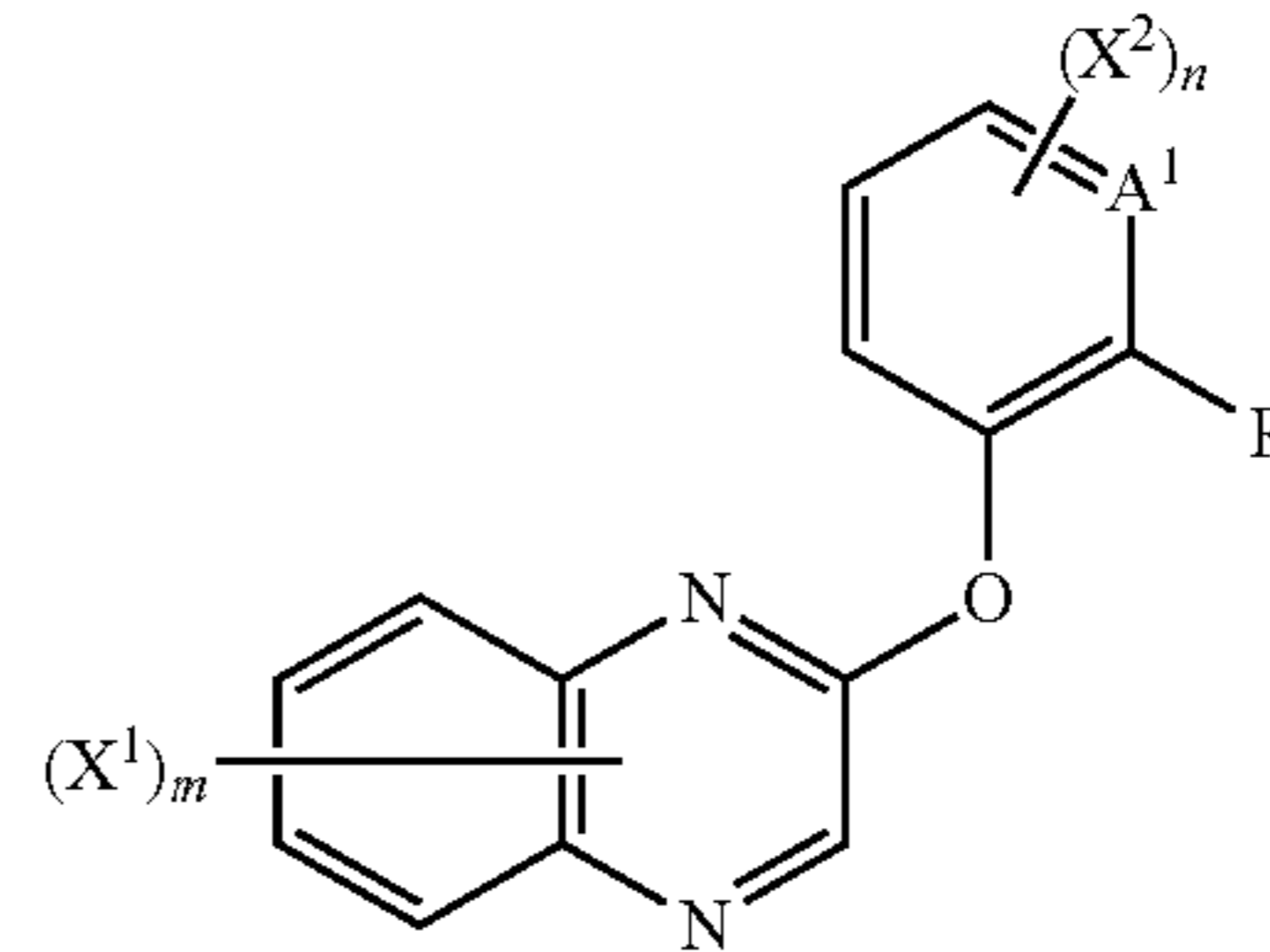
[Chemical Formula 10]
