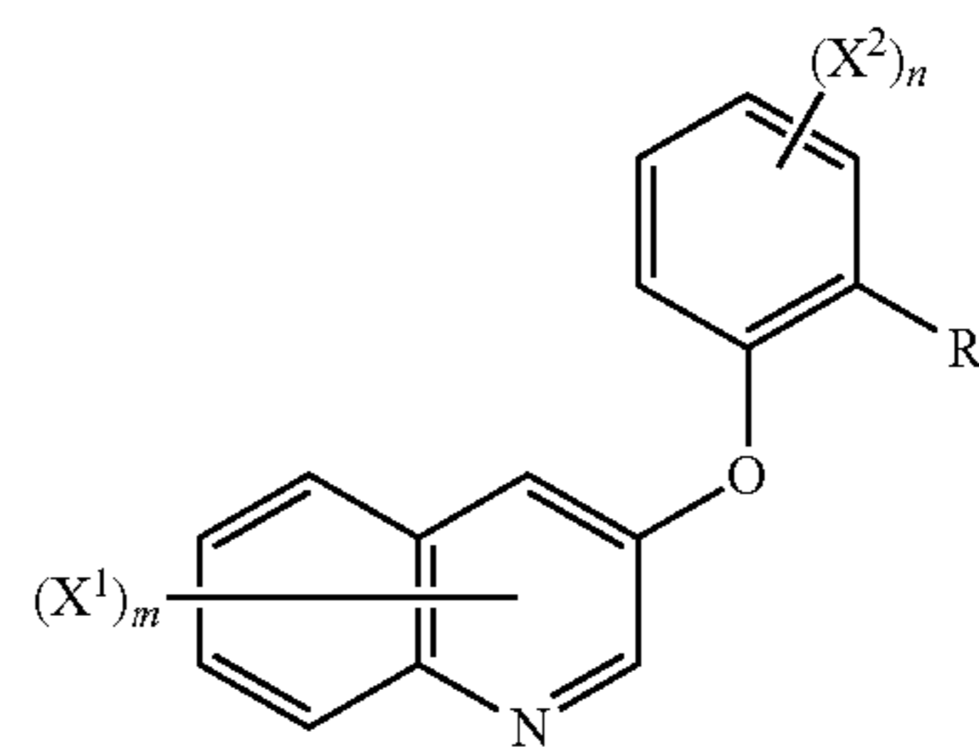
[Chemical Formula 9]
