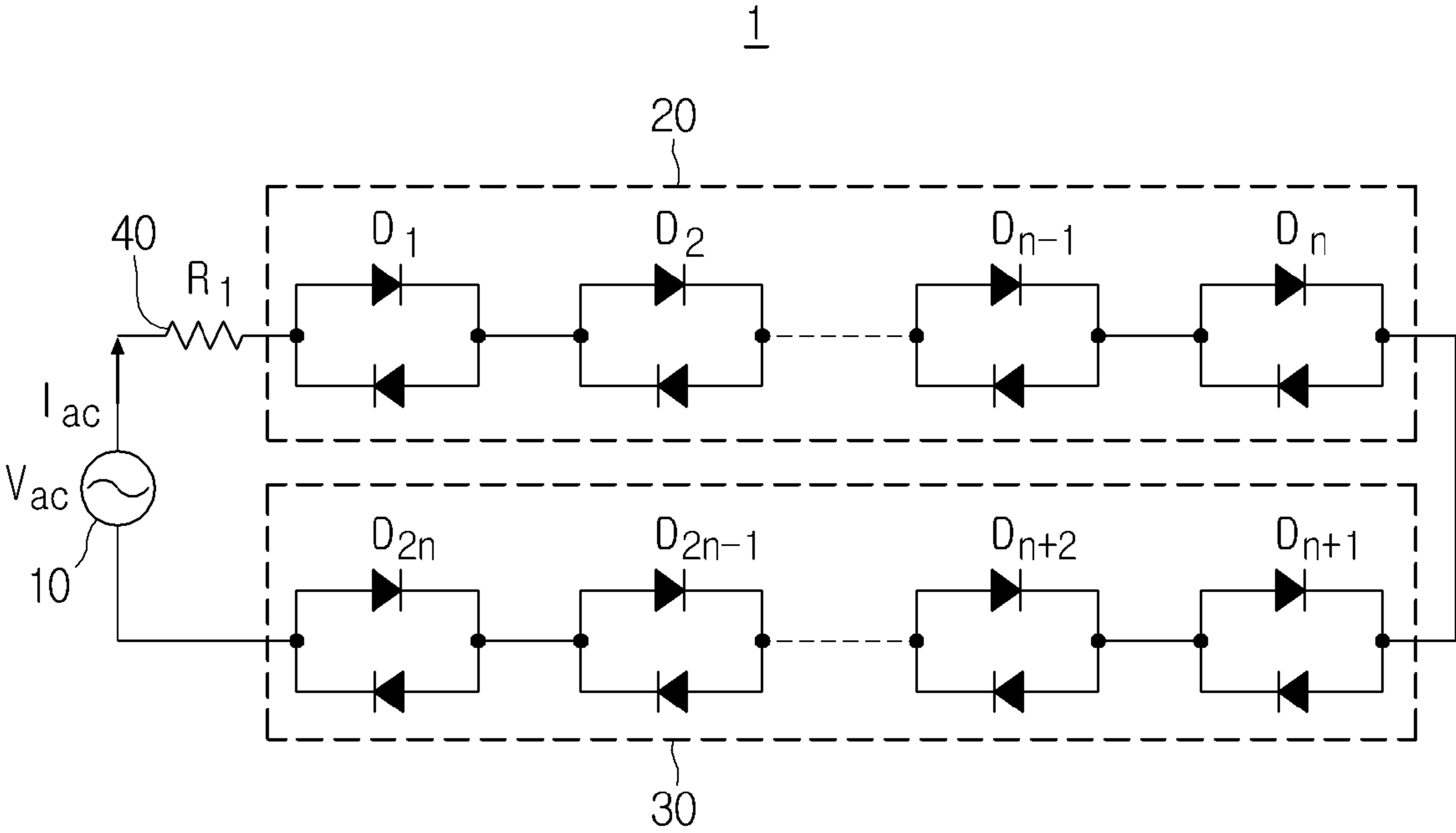
FIG. 1 (Prior Art)
