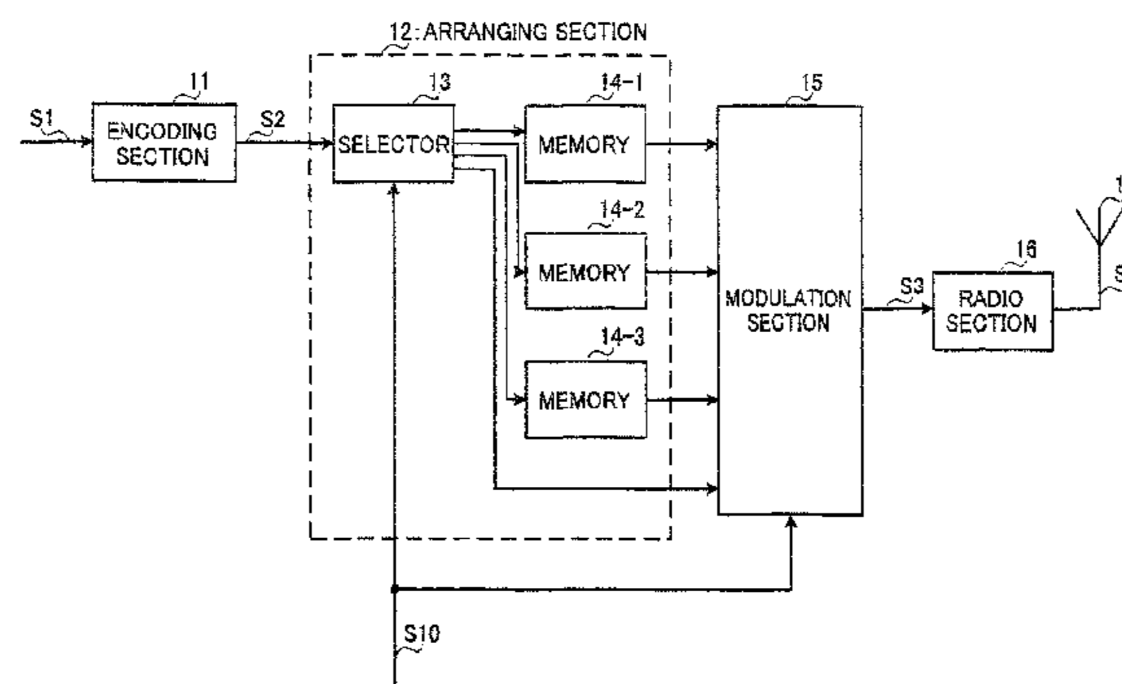
10 TRANSMITTING APPARATUS
