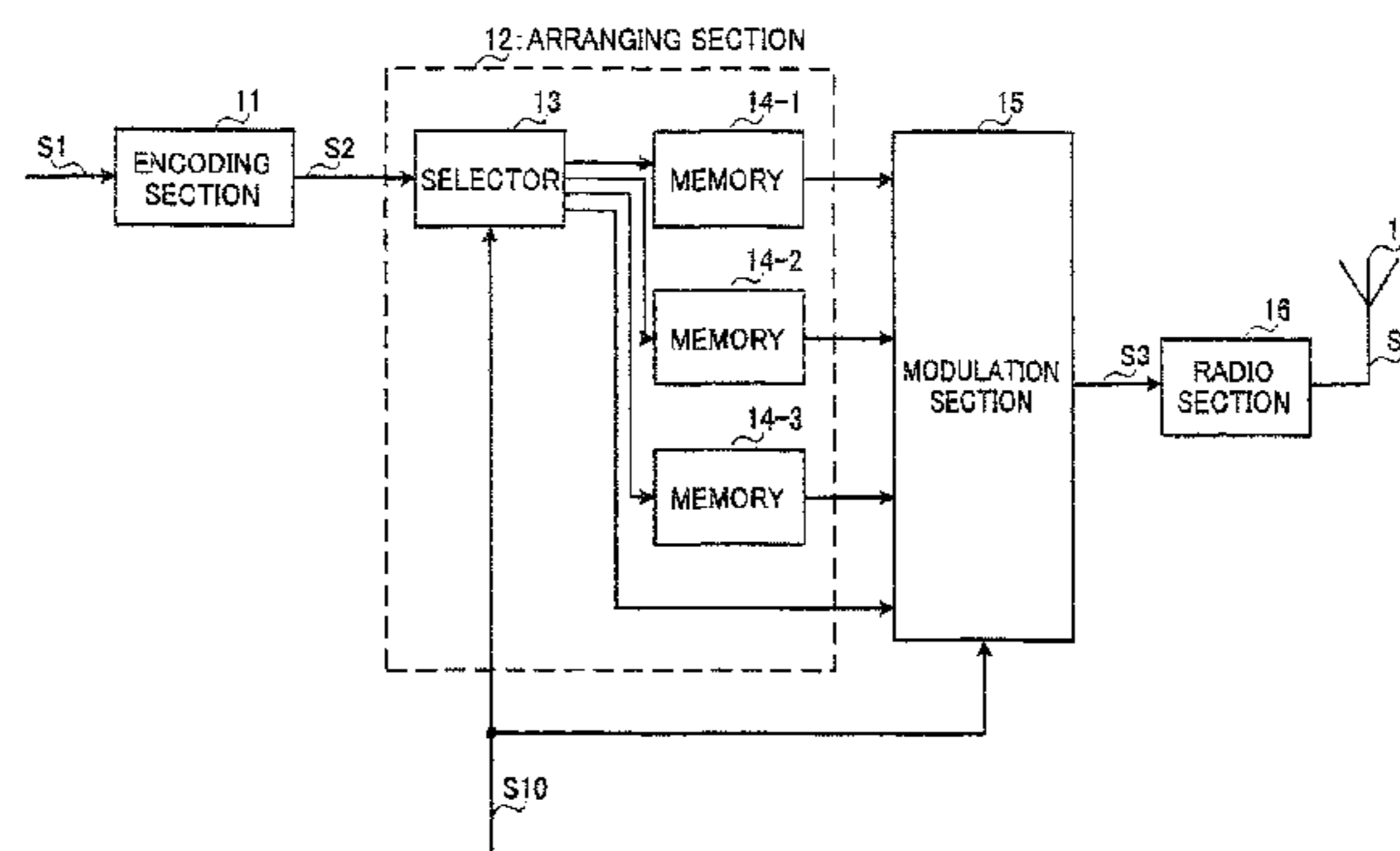
10 TRANSMITTING APPARATUS
