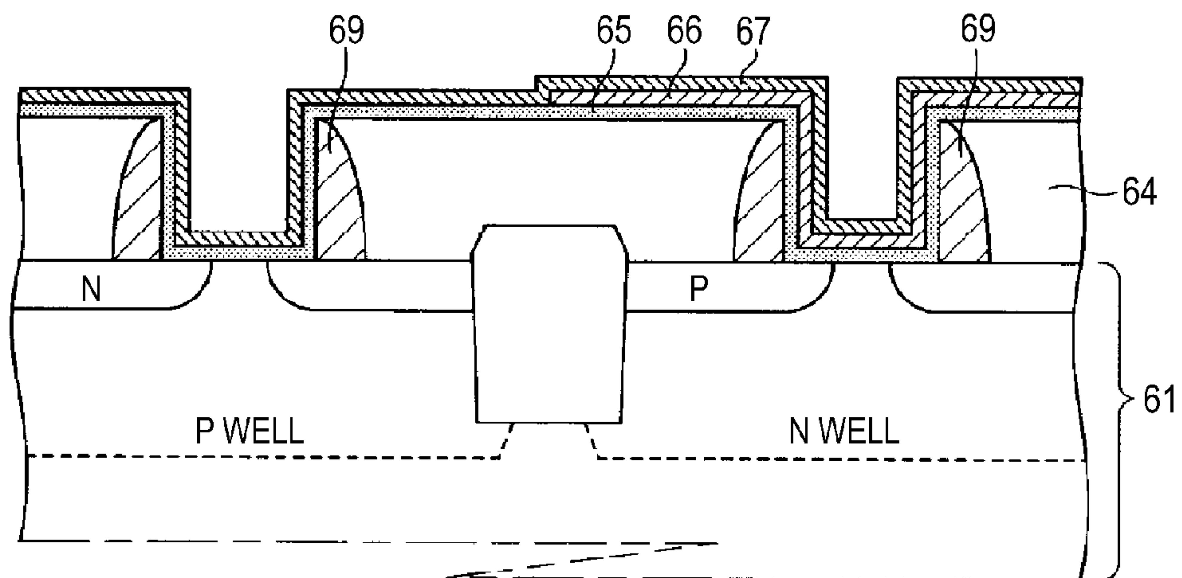
RELATED ART - FIG.15C
