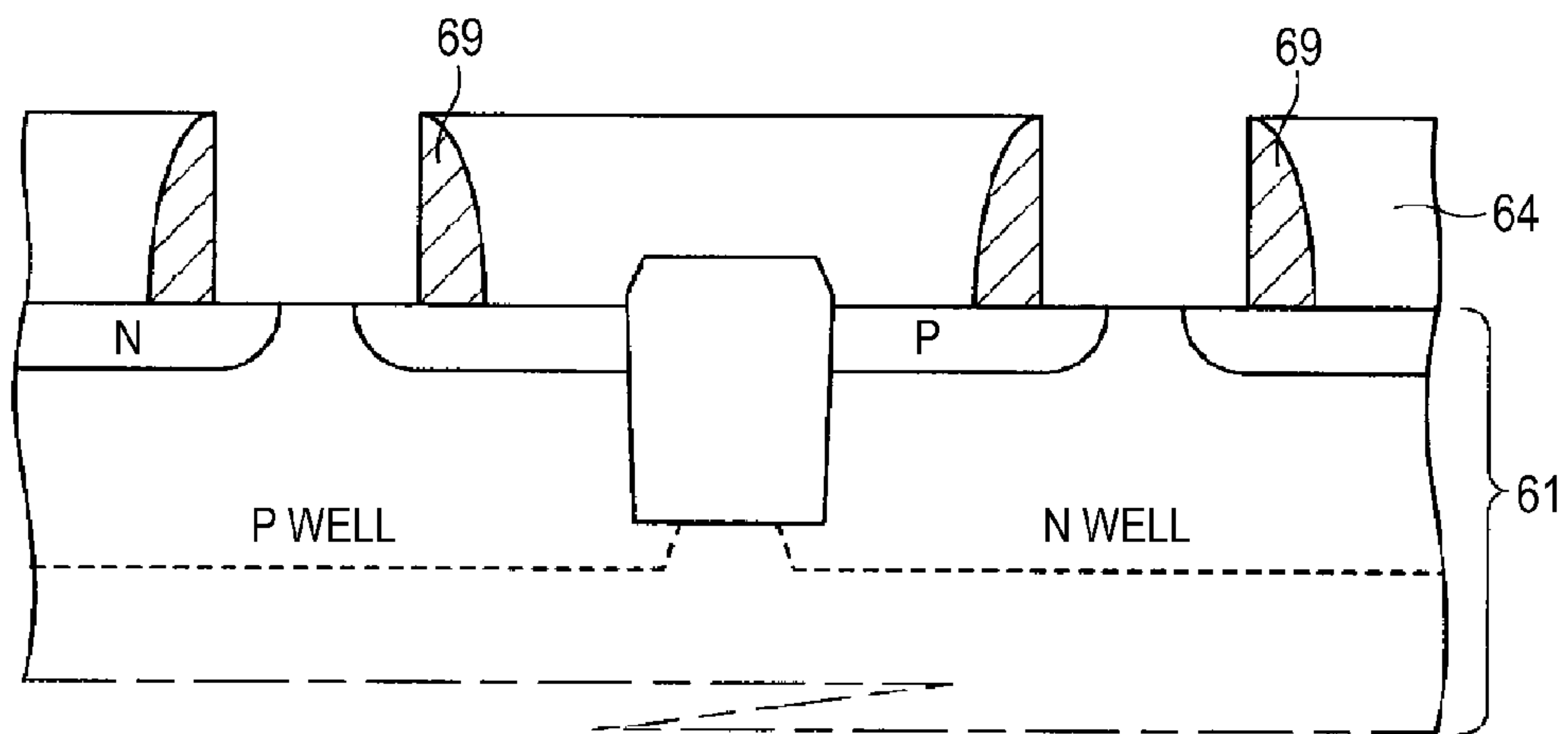
RELATED ART - FIG.15C
