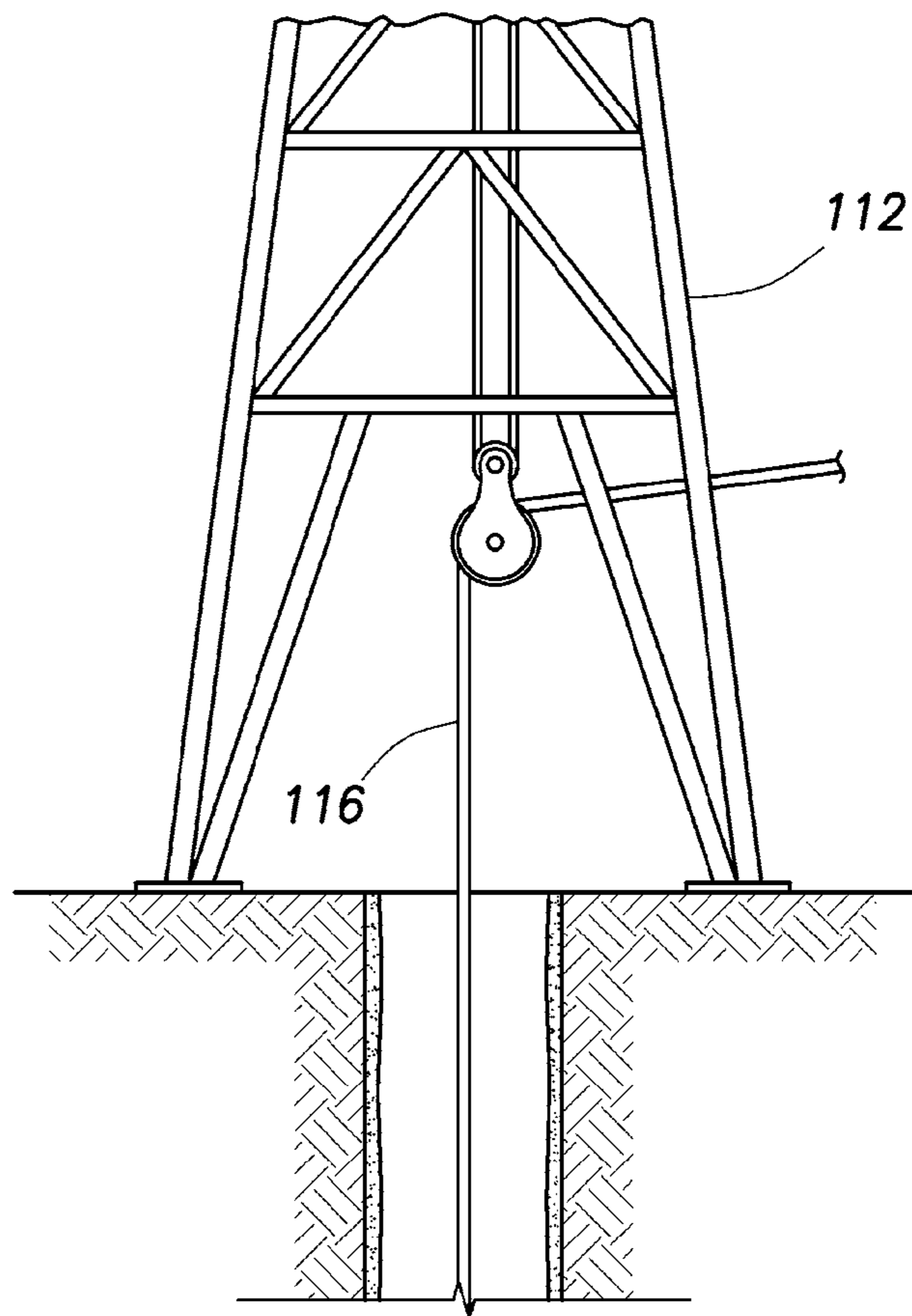
Fig. 12 (PRIOR ART)
