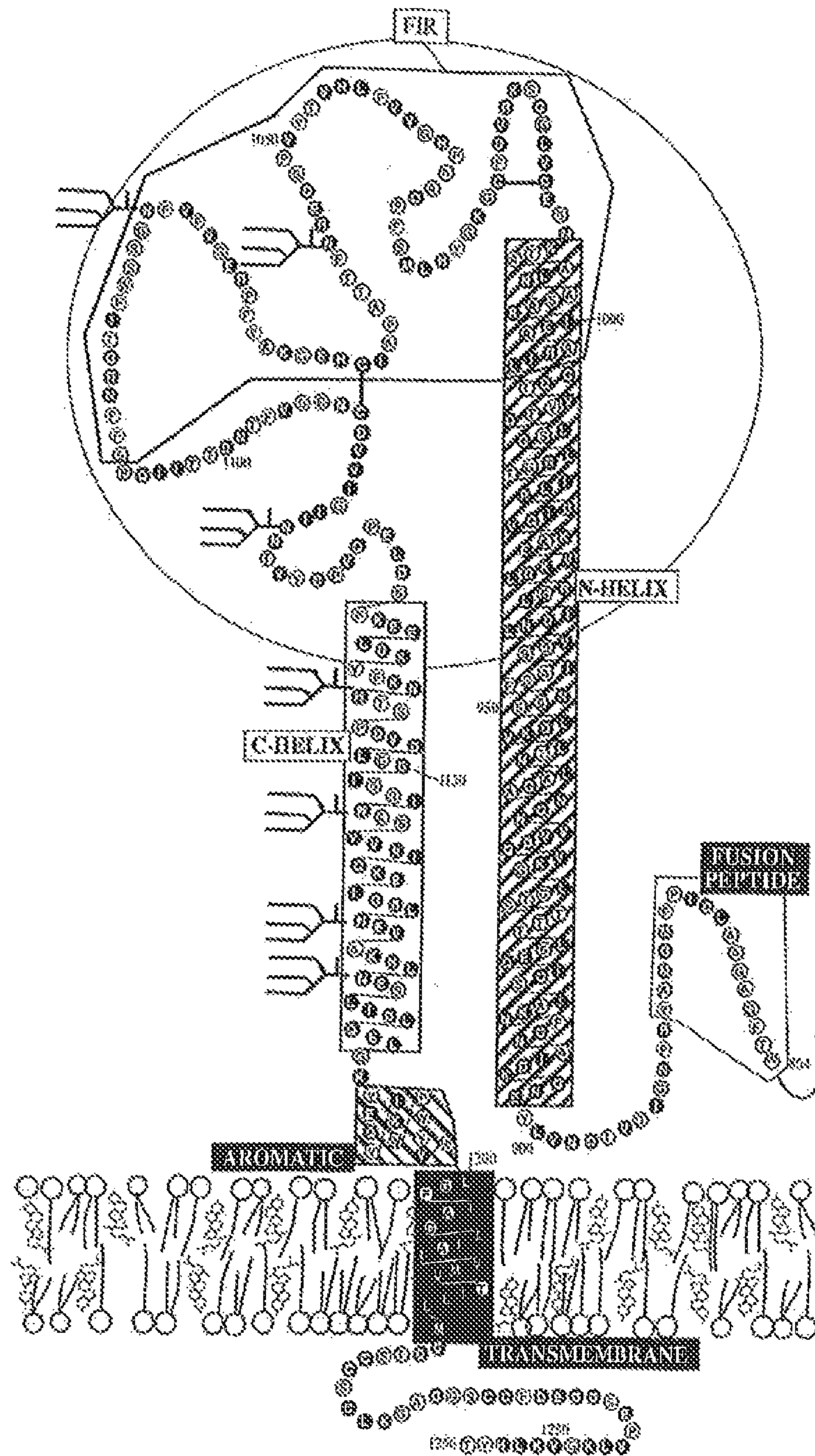
SARS CoV S Figure 3
