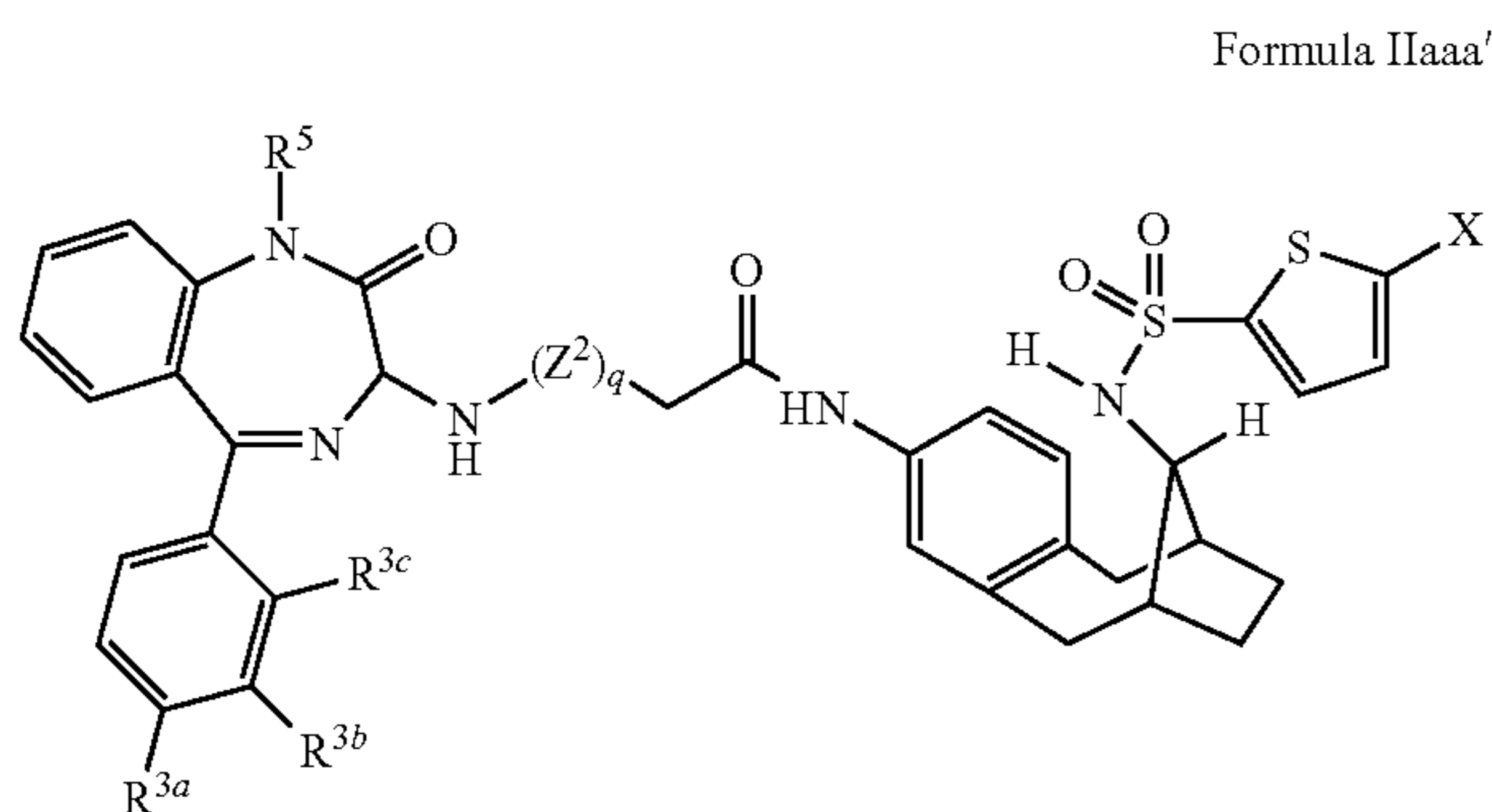
Formula IIaaa''
