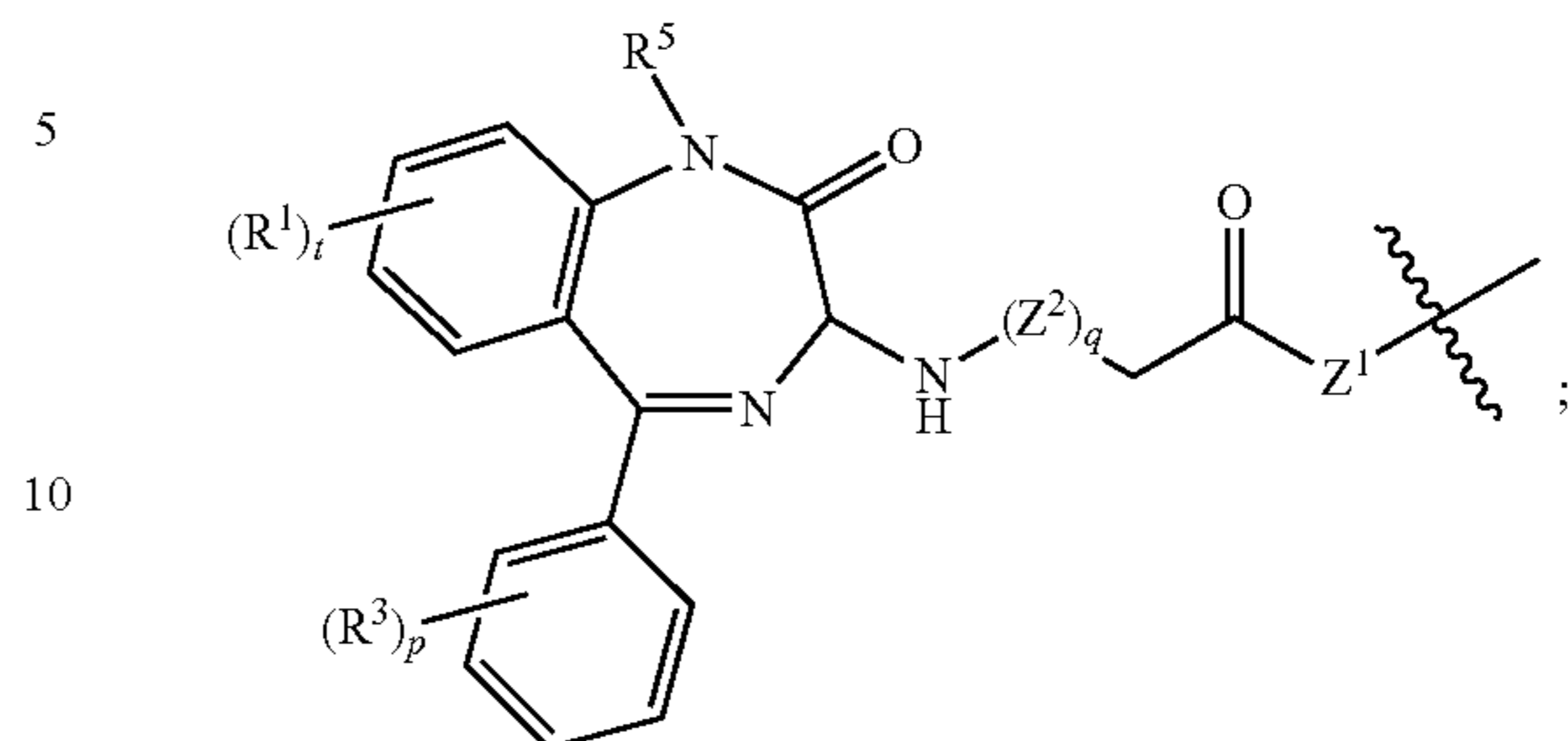
Formula II
