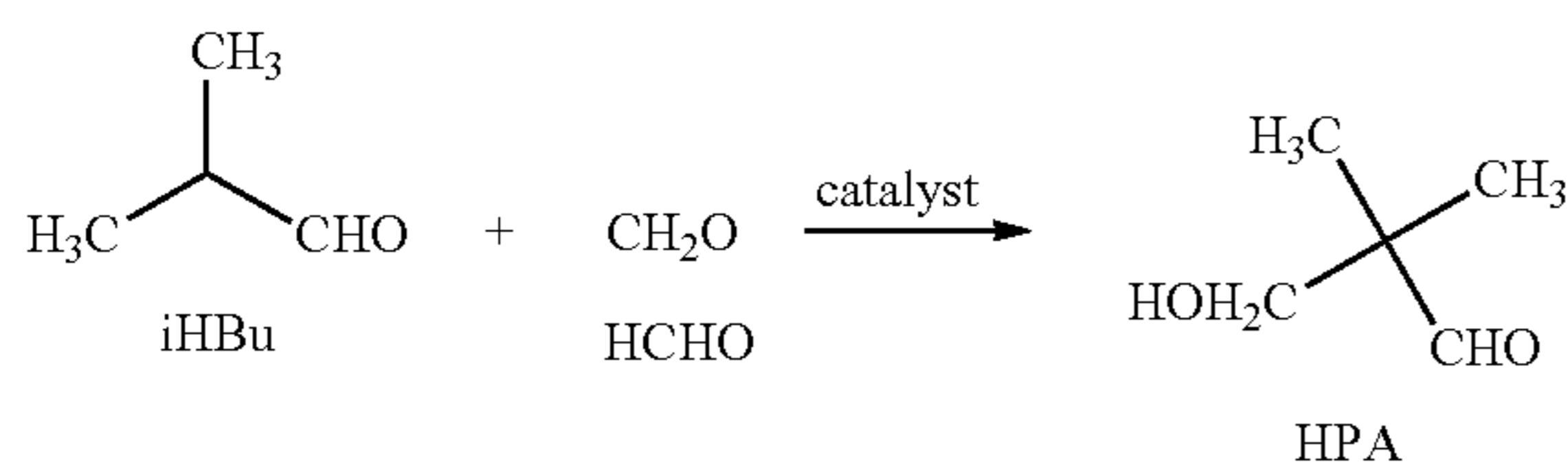
Scheme 1 Preparation of Hydroxypivaldehyde in an Aldol Condensation
