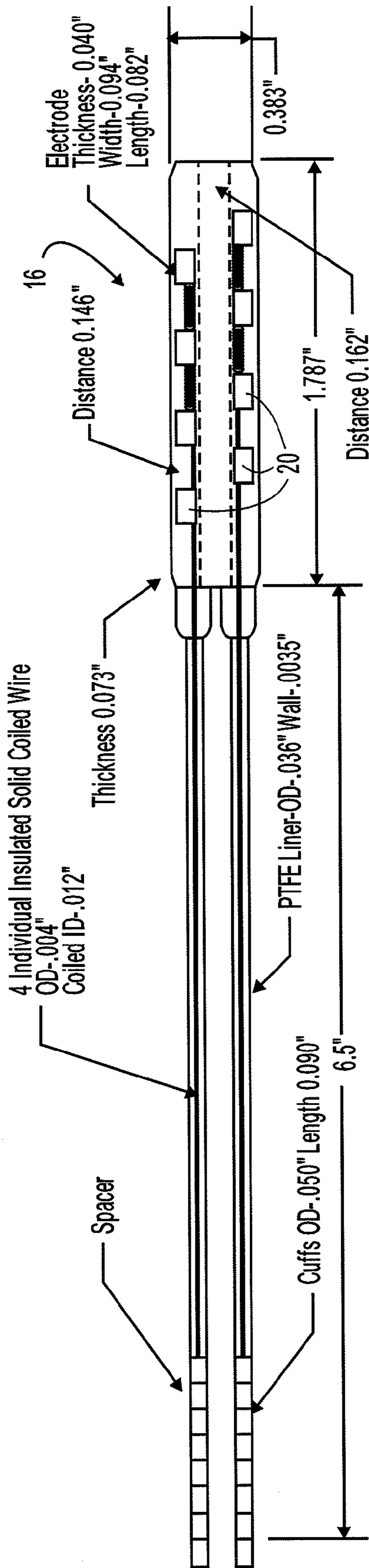
FIG. 3 (PRIOR ART)
