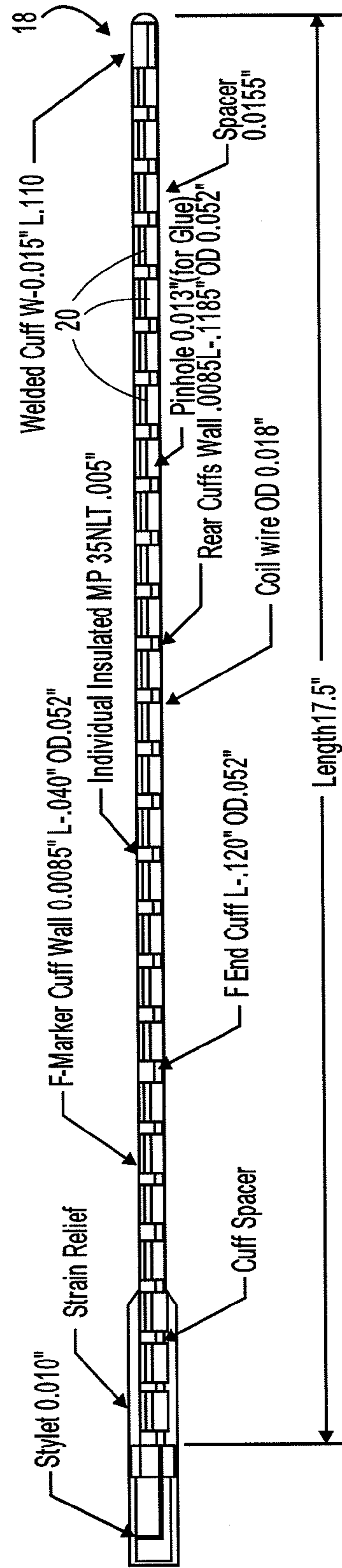
FIG. 4 (PRIOR ART)
