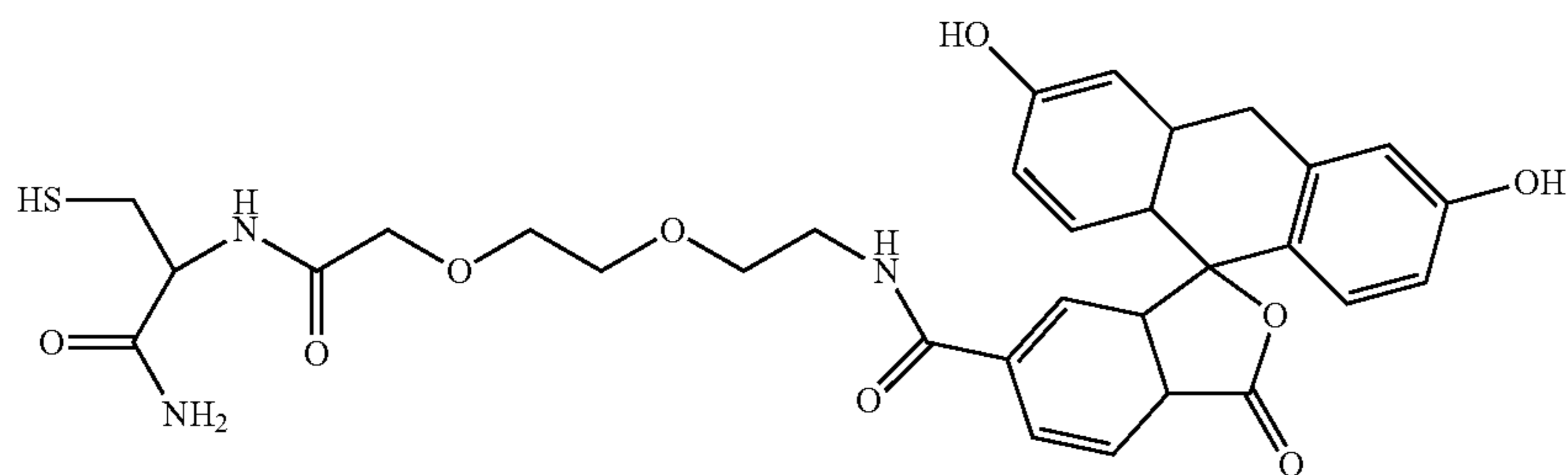
5,6-Isomers
