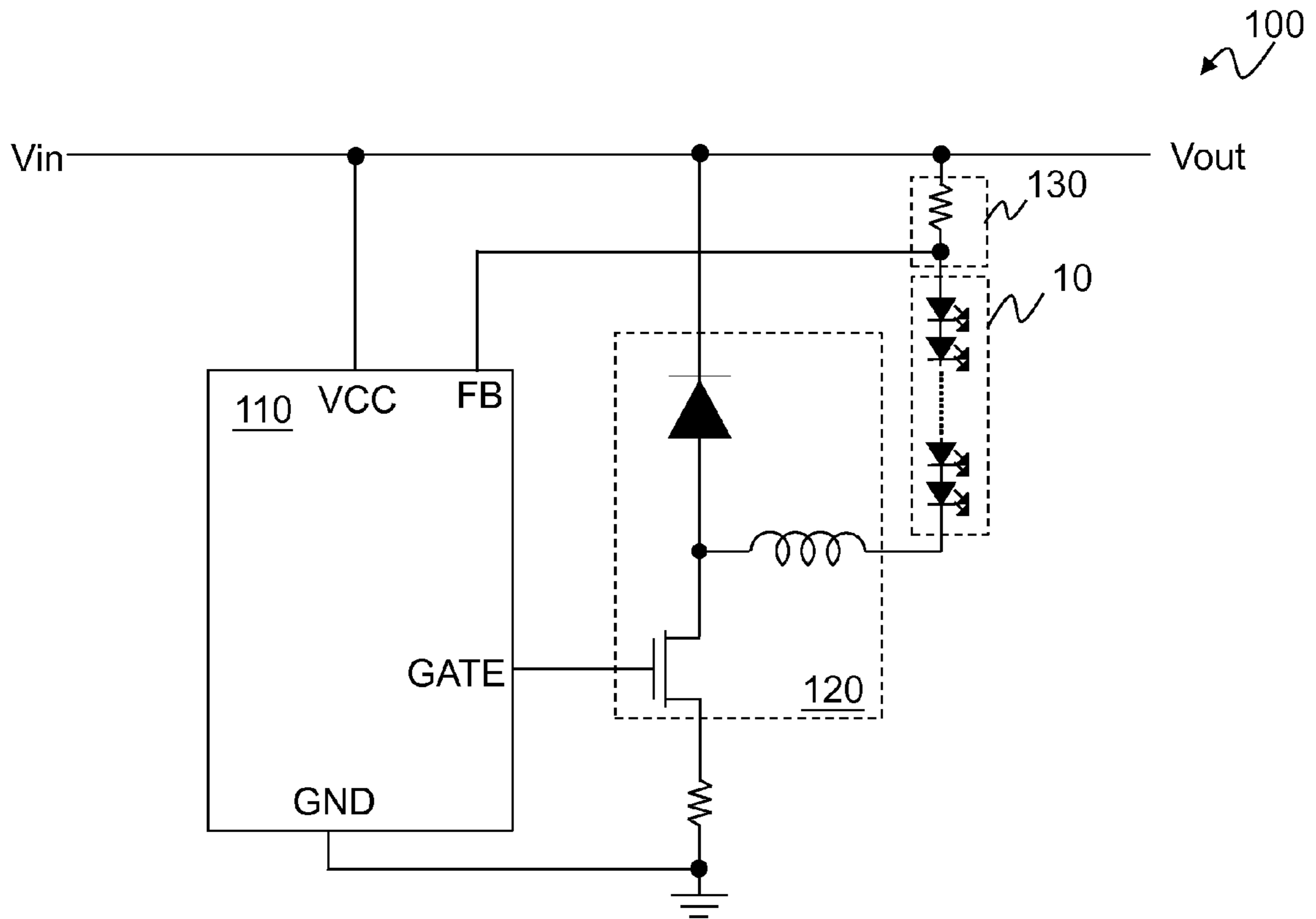
Fig. 1 (Prior Art)
