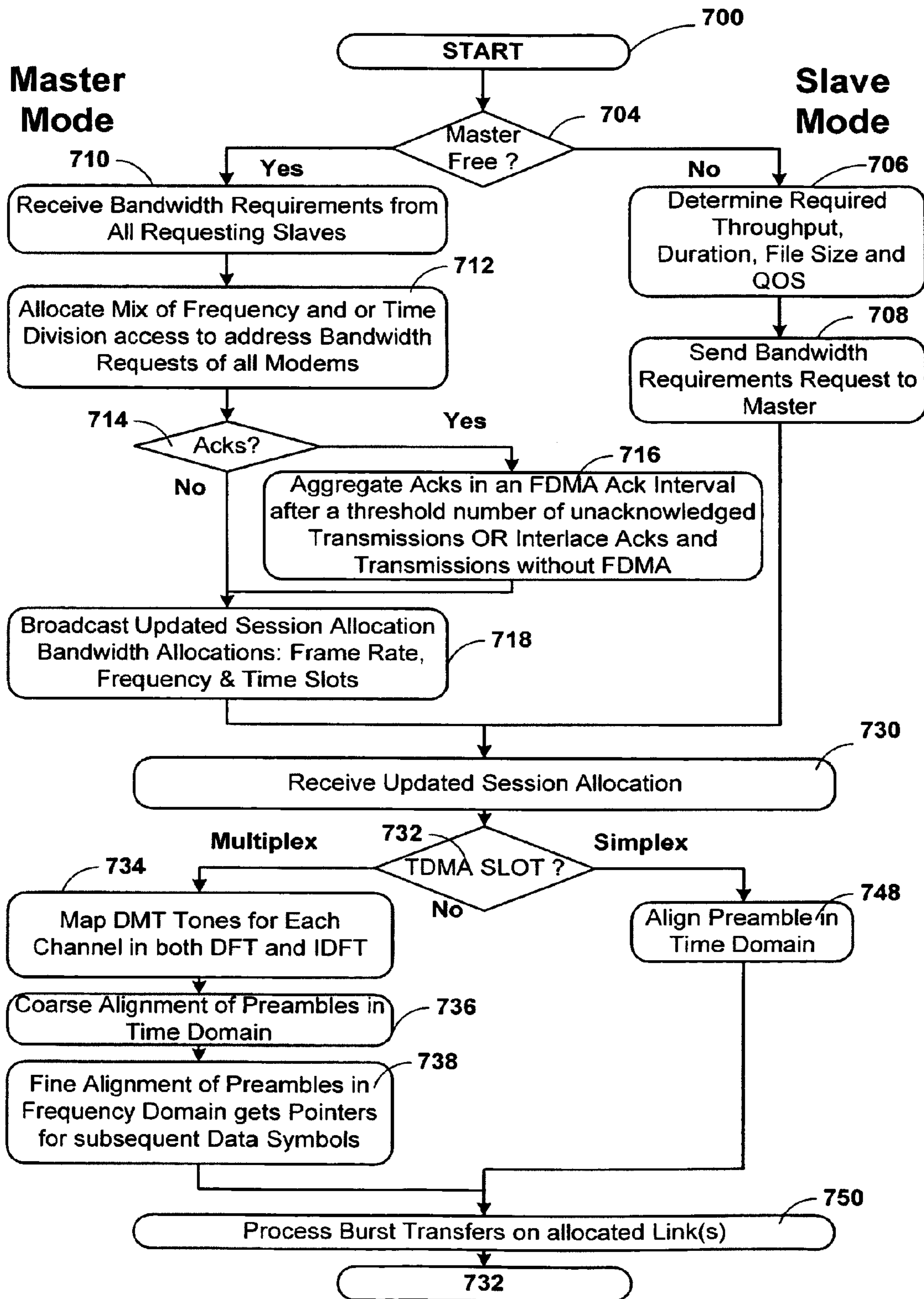
FIG. 7 Network Modem Burst Mode Processing
