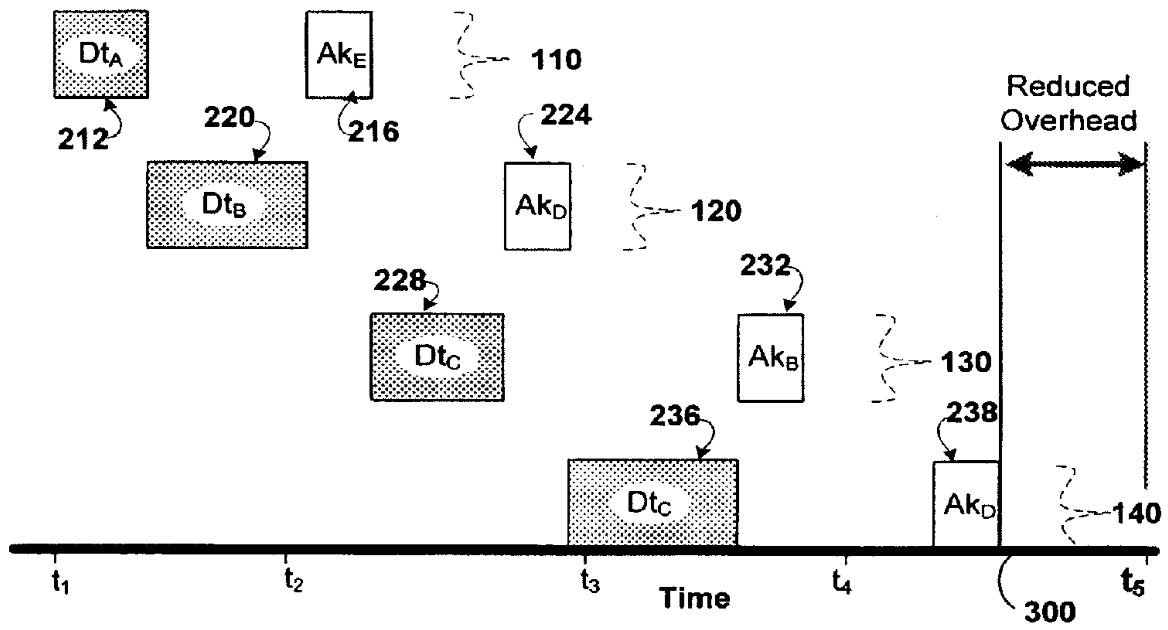
FIG. 3A Overlap Scheduling for TDMA / CSMA
