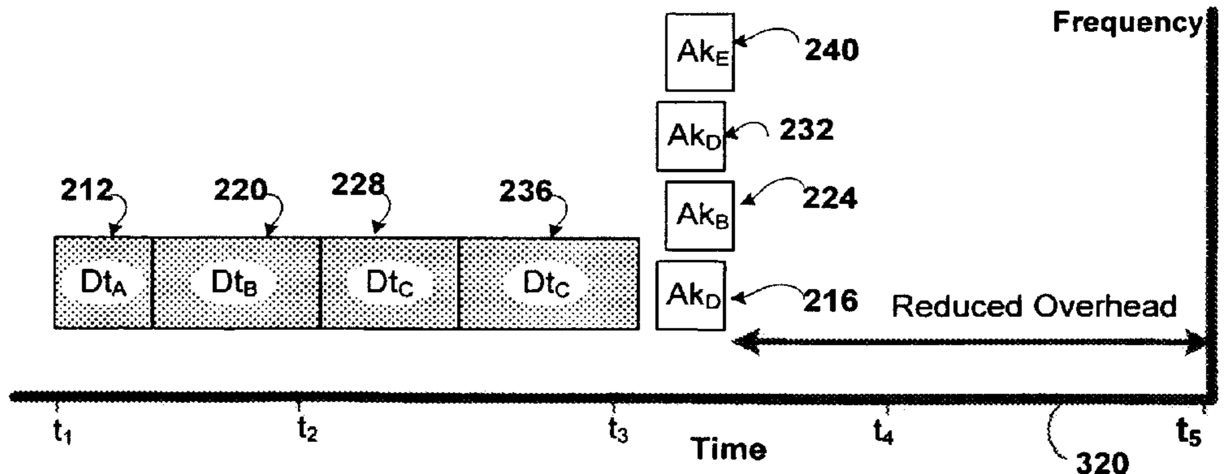
FIG. 3B Overlap Scheduling for TDMA / CSMA
