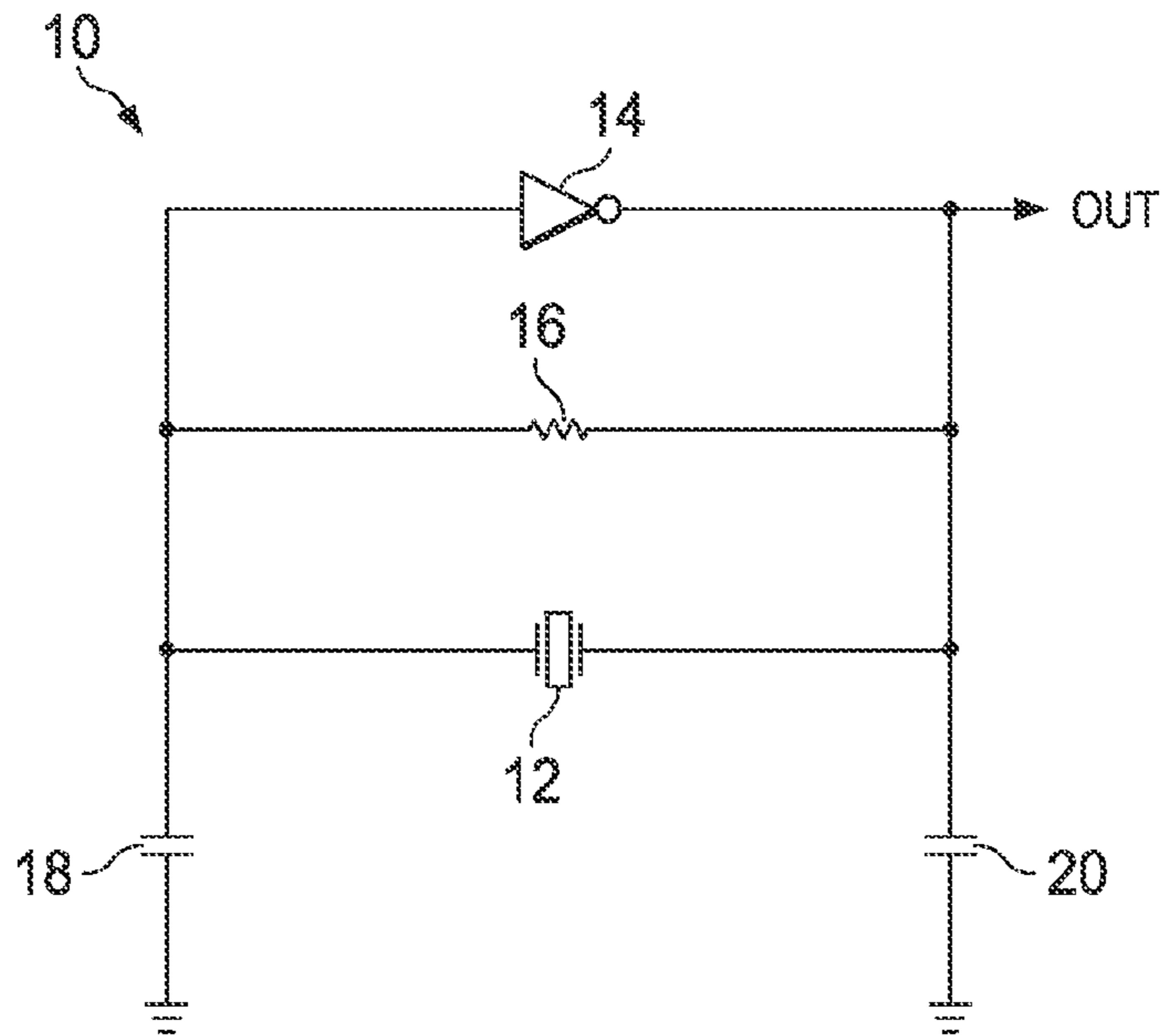
FIG. 1 (PRIOR ART)
