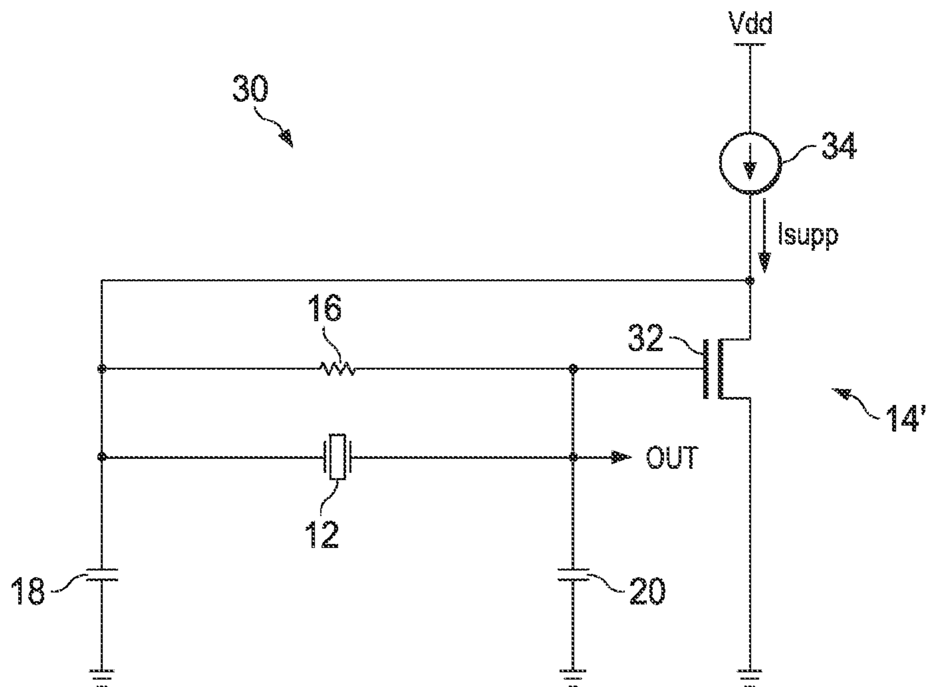
FIG. 2 (PRIOR ART)
