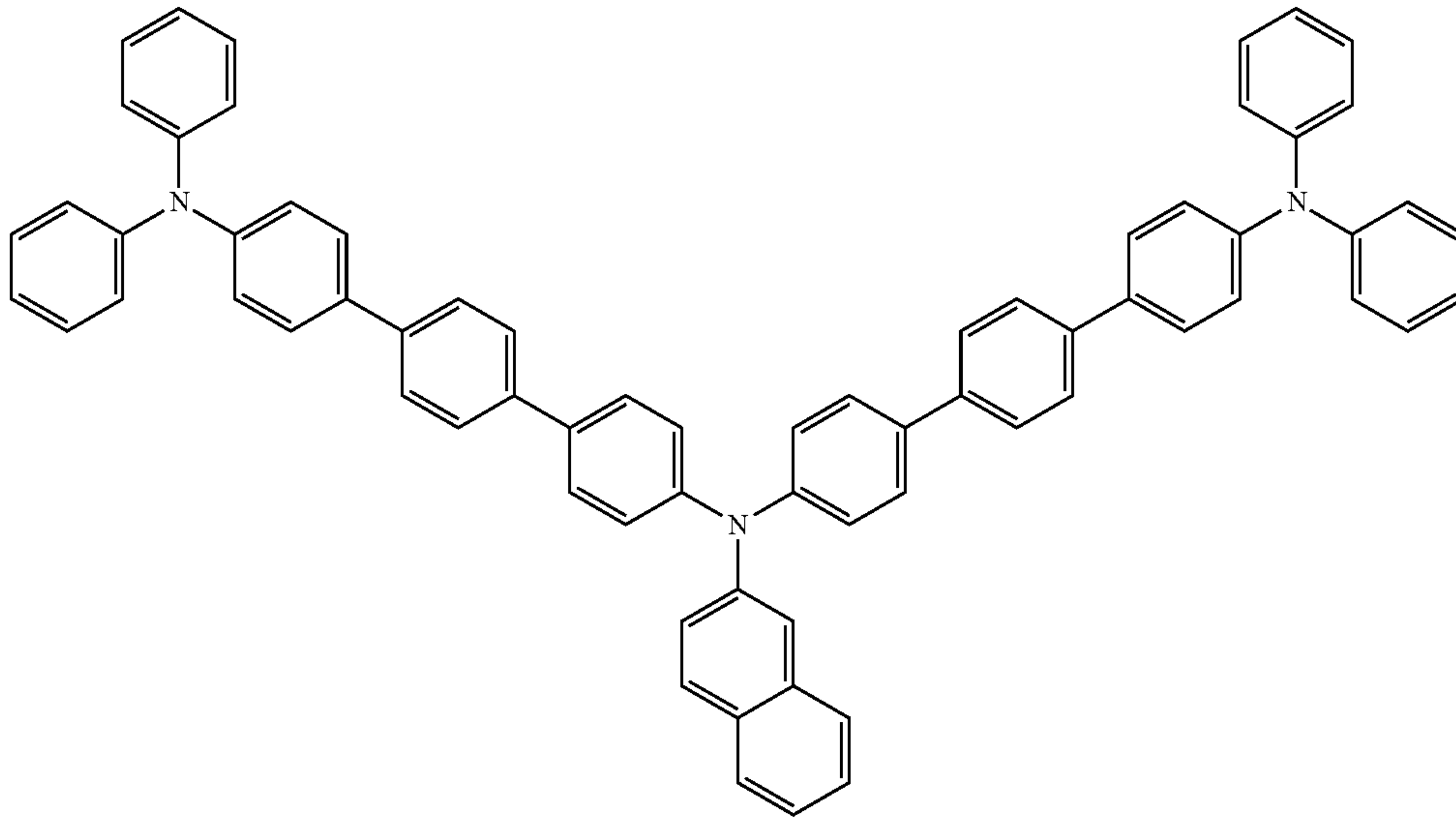
Chemical Formula 15
