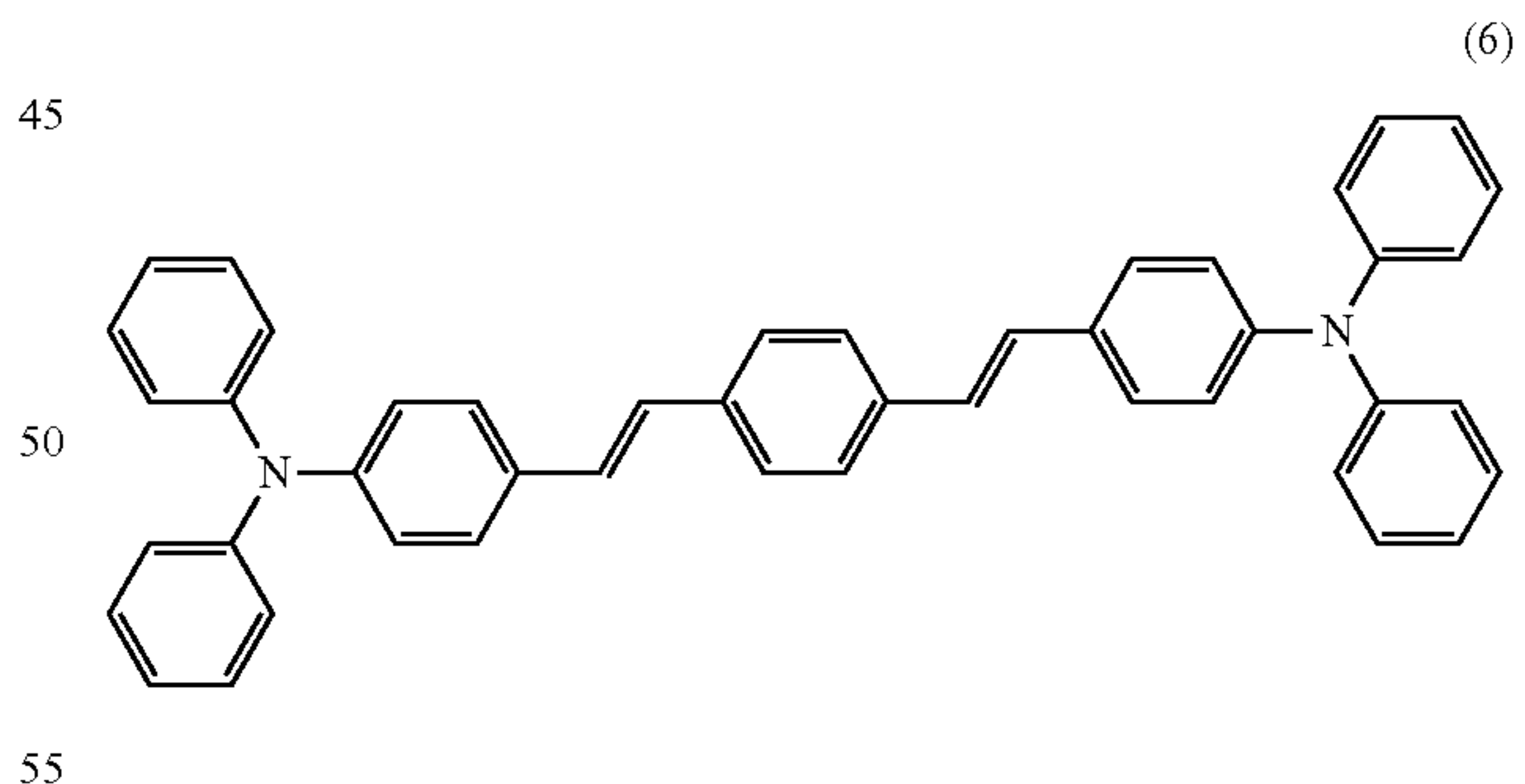
Chemical Formula 21
