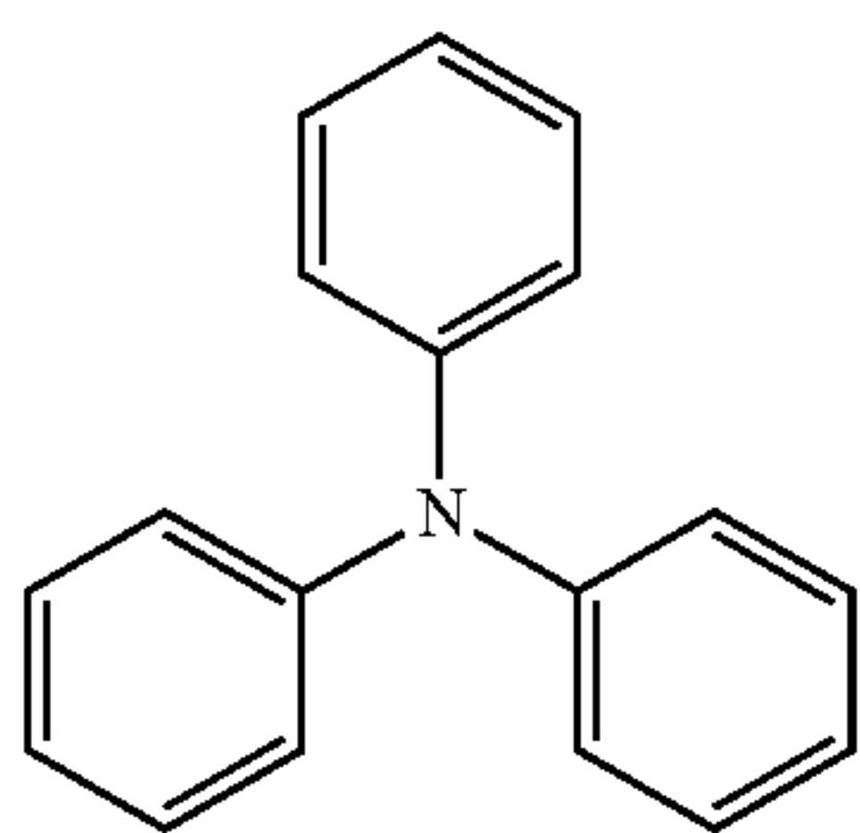
Chemical Formula 4
