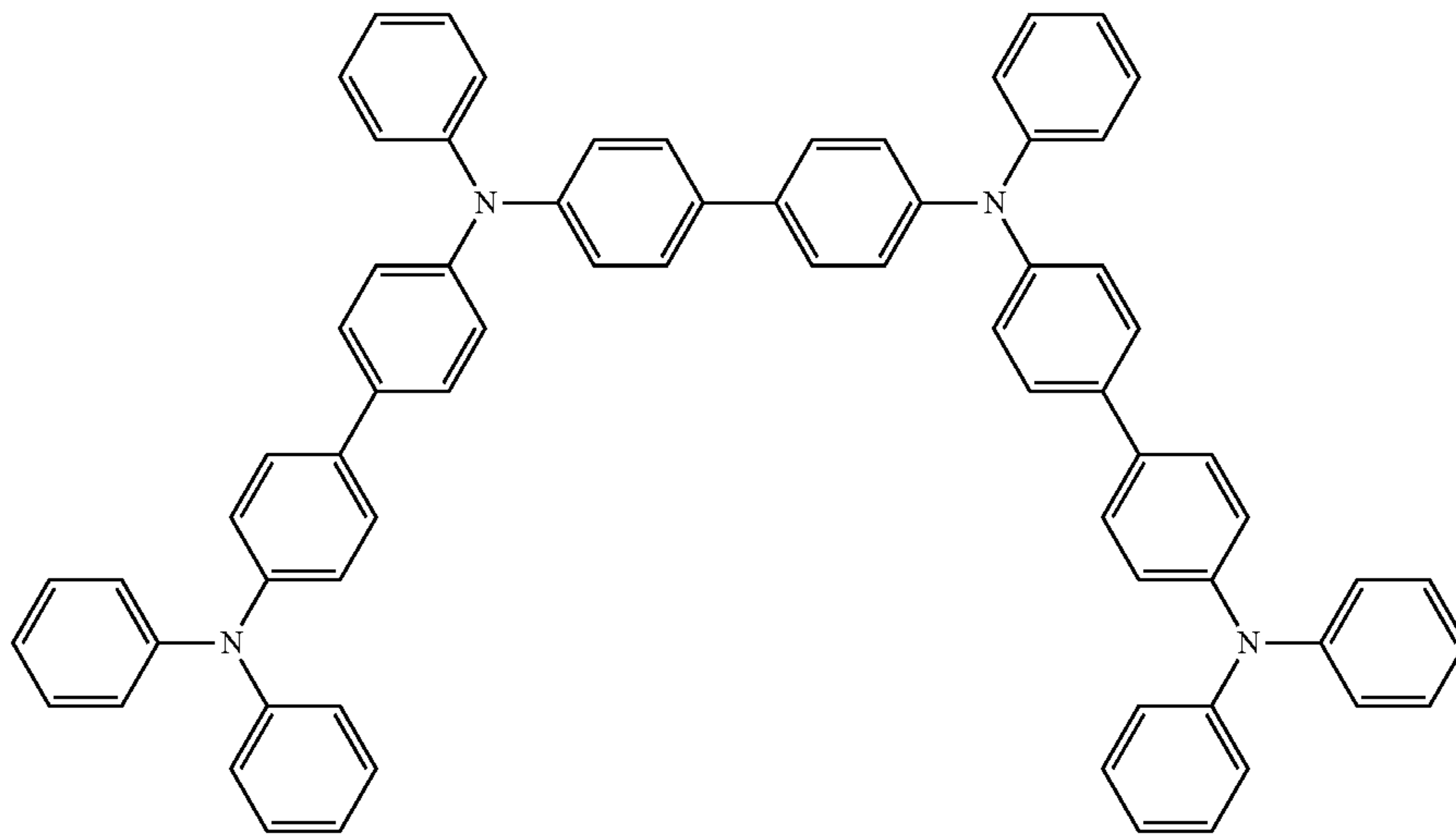
Chemical Formula 15
