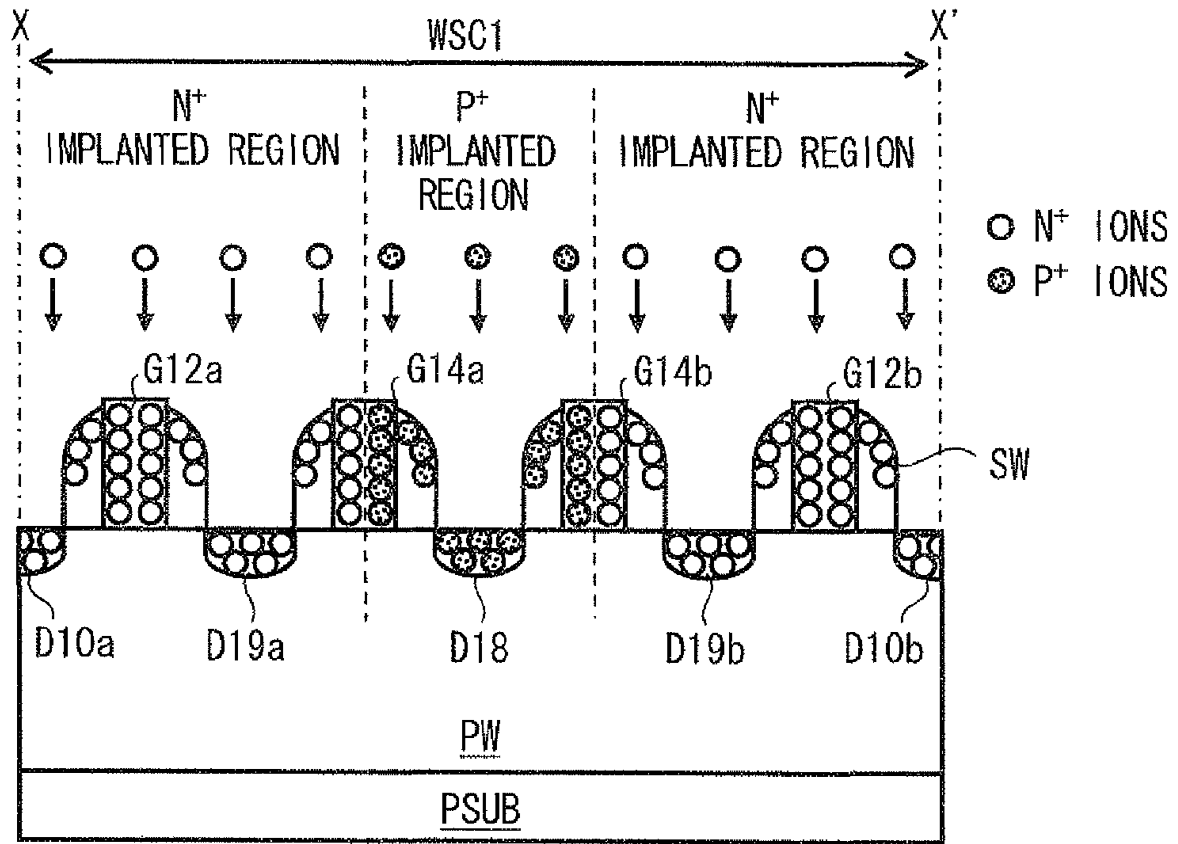
ION IMPLANTATION
