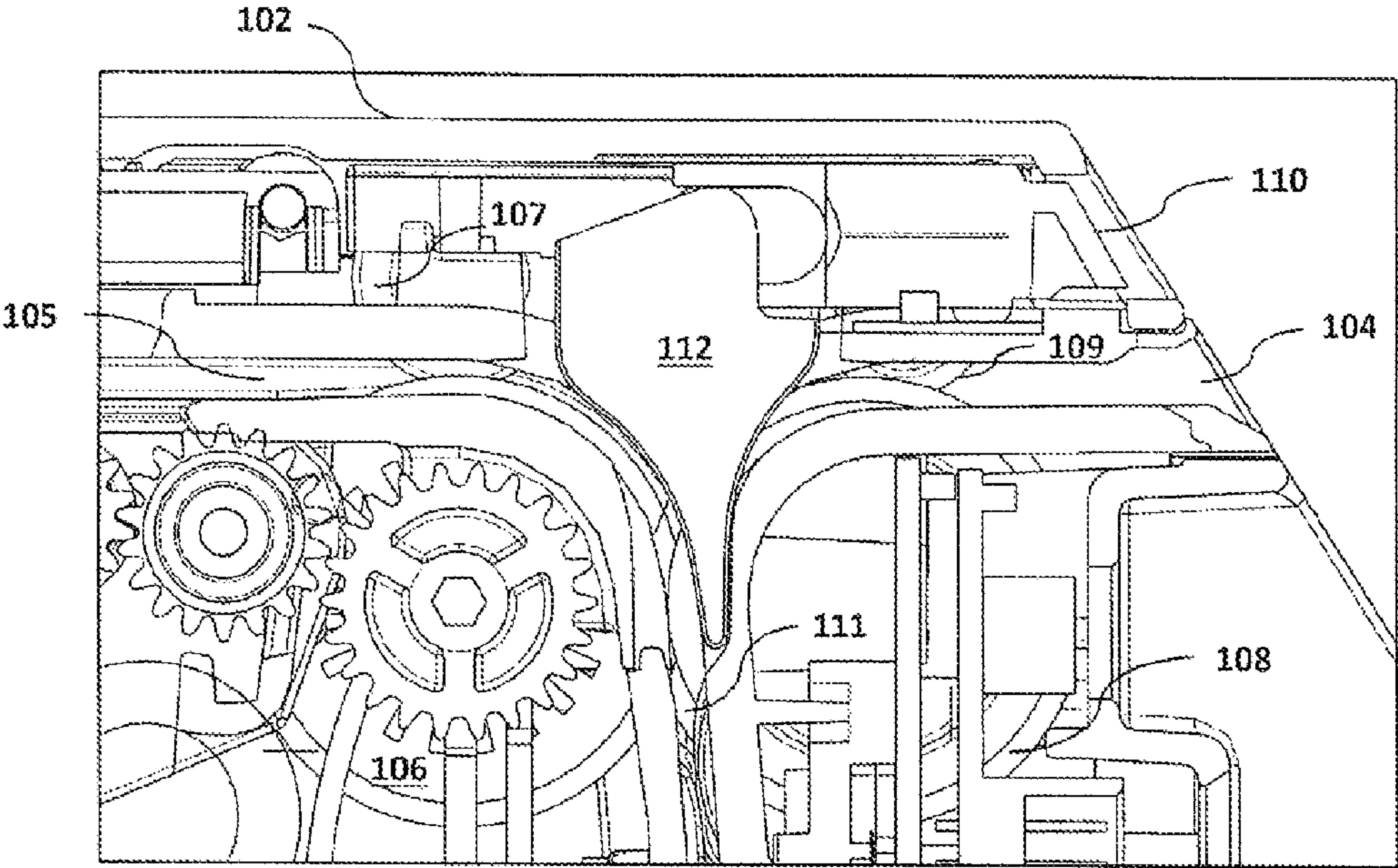
PRIOR ART
