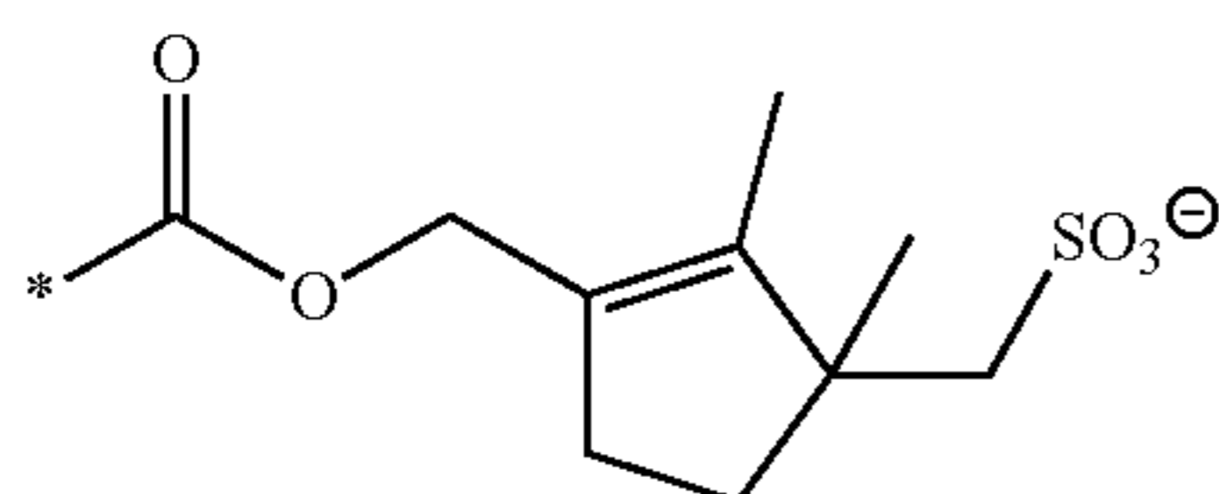
[Chemical formula 5]
