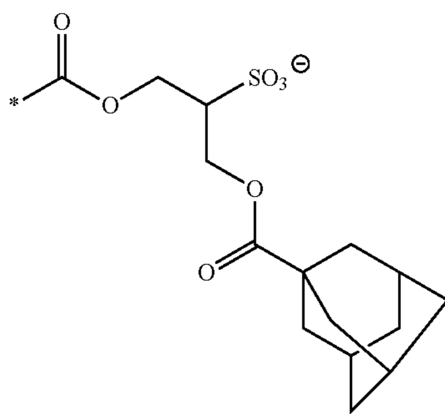
[Chemical formula 5]
