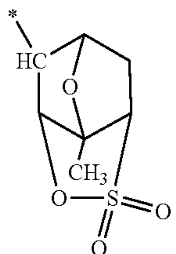
[Chemical formula 39]
