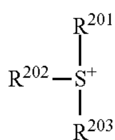
[Chemical formula 6]
