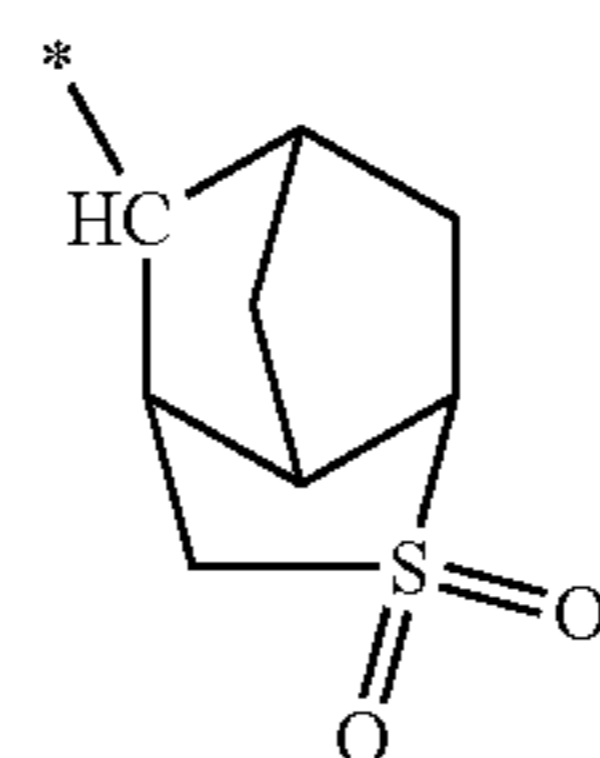
[Chemical formula 40]
