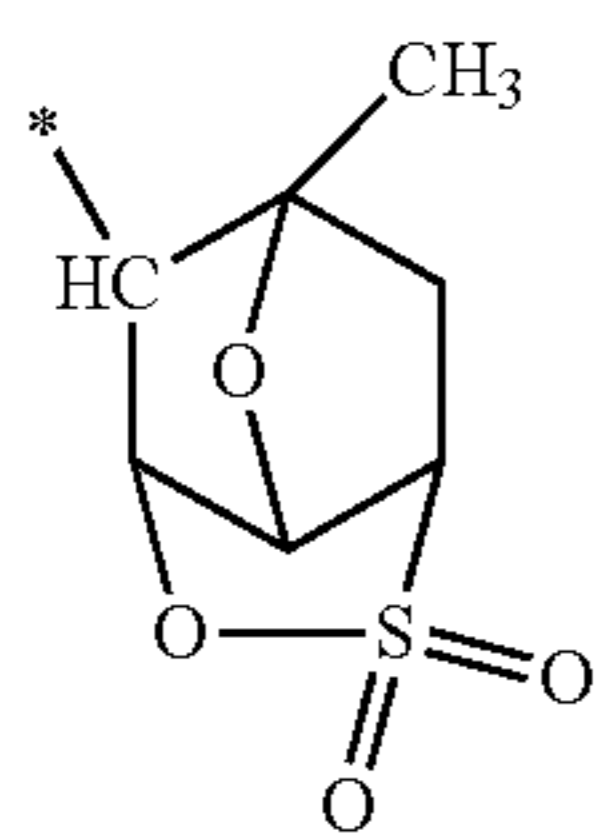
[Chemical formula 39]
