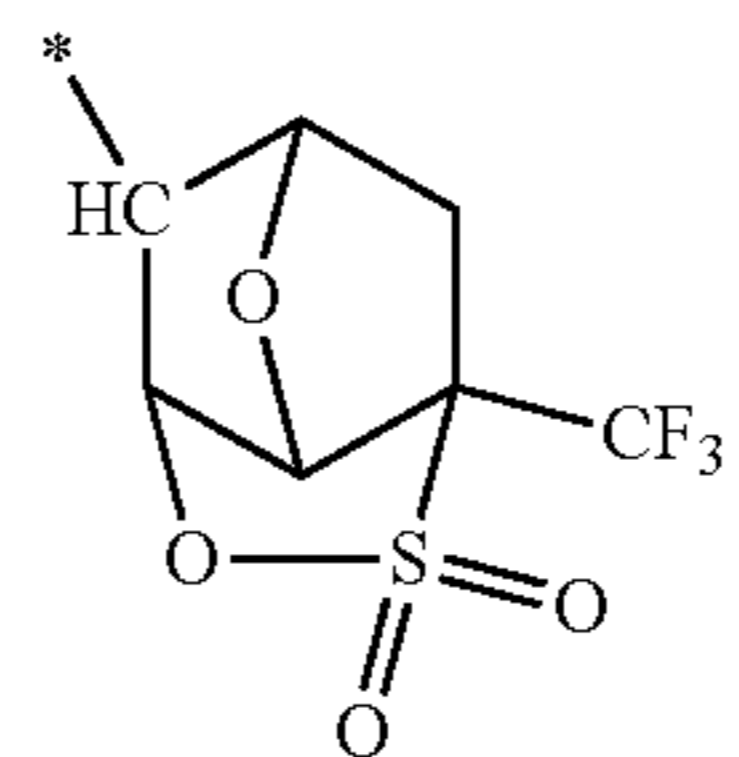
[Chemical formula 40]
