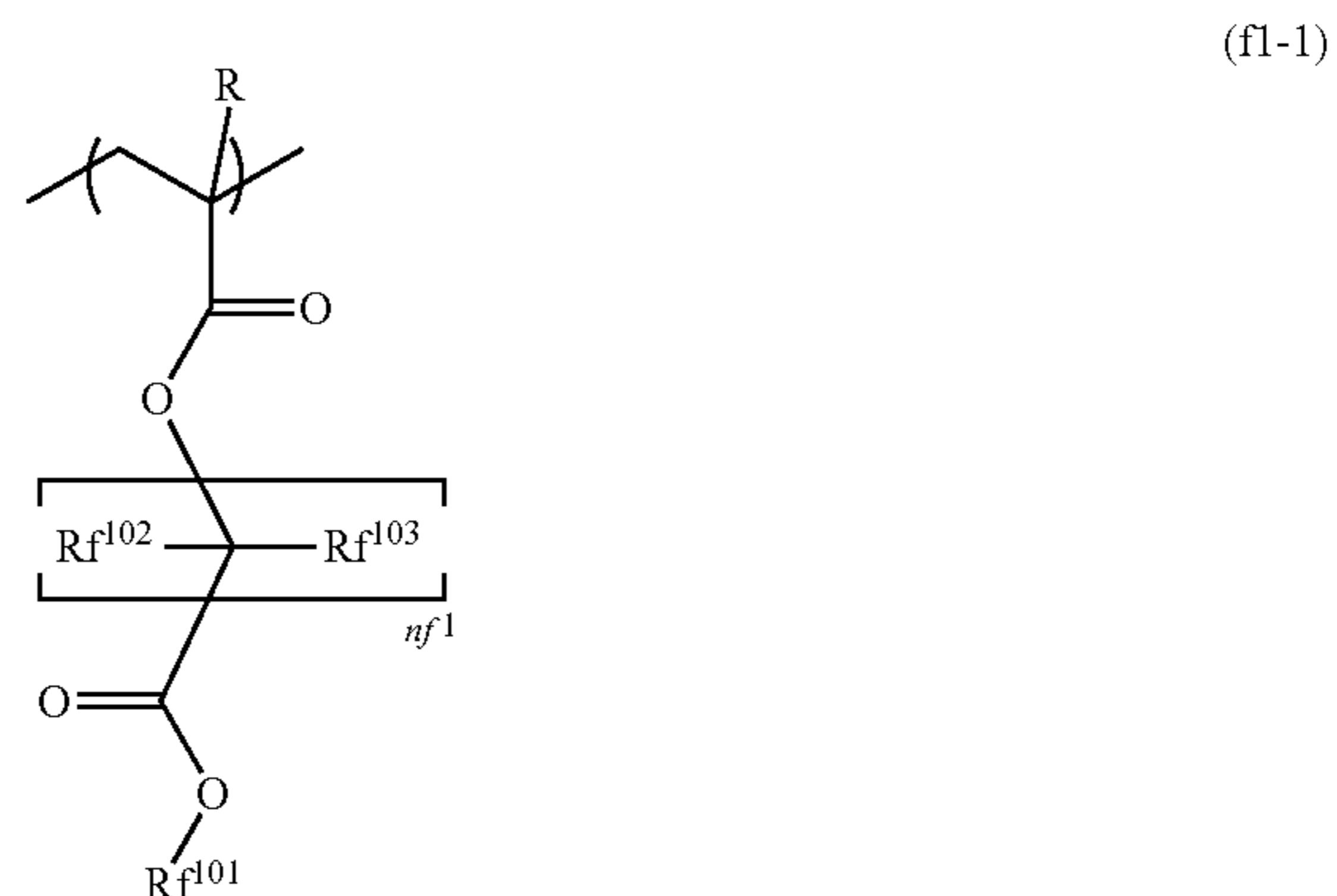
[Chemical formula 57]
