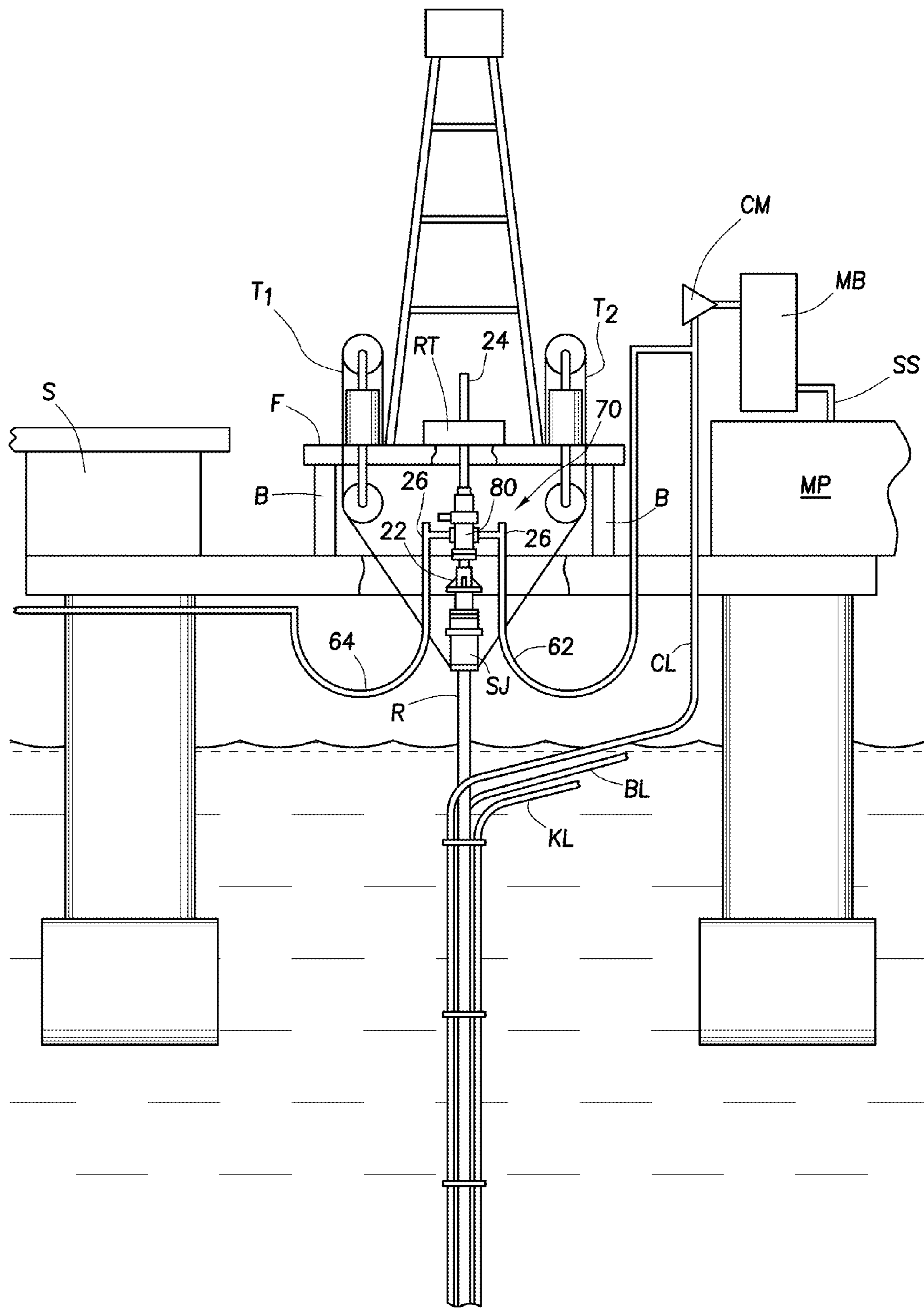
FIG. 2 (PRIOR ART)
