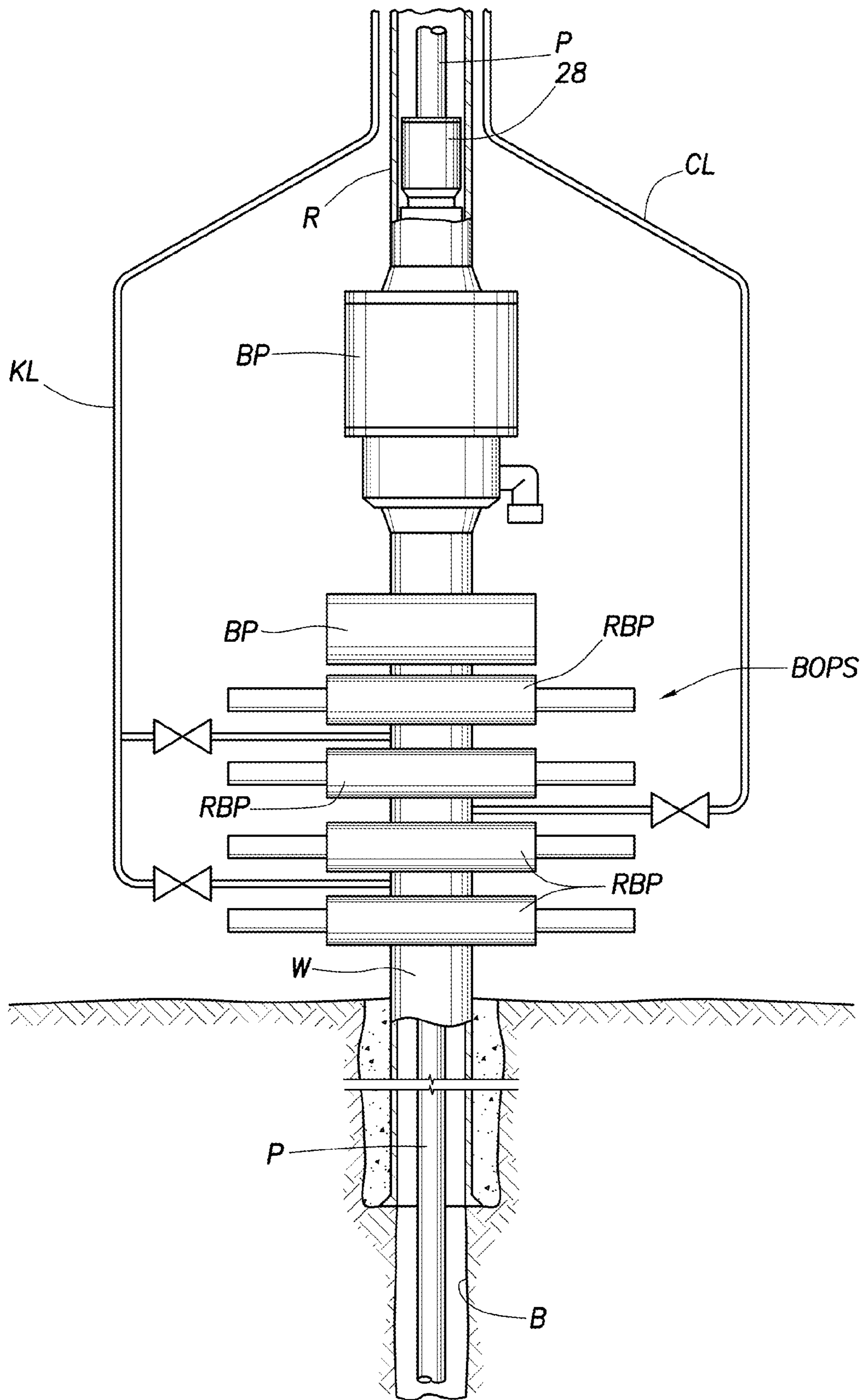
FIG. 5 (PRIOR ART)
