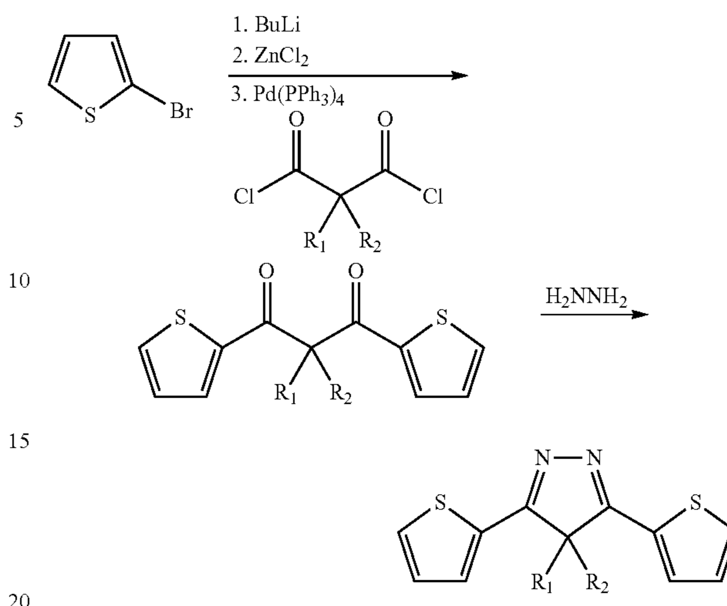
Diagram 2. Synthesis of 3,5-dithien-2-yl-4,4-disubstituted pyrazole
