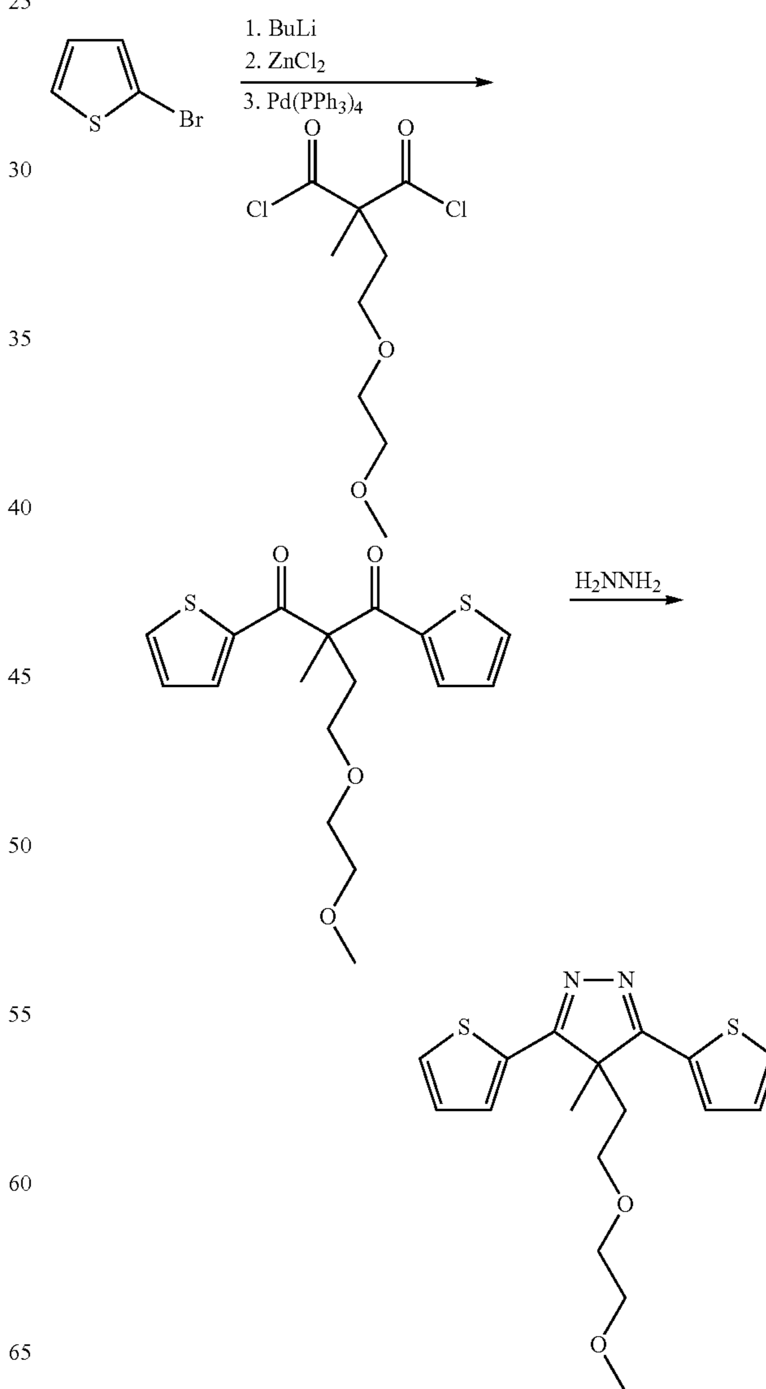
Diagram 1. Synthesis of 3,5-dithien-2-yl-4,4-disubstituted pyrazole (DTDSPy).
