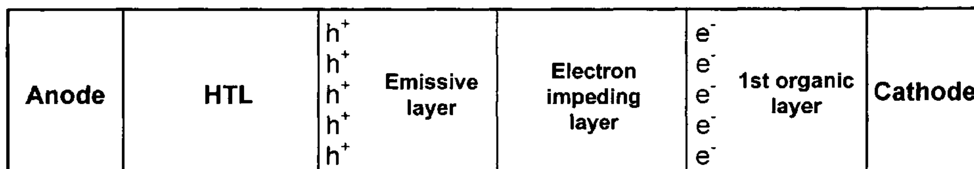
Figure 63a: Device Having an Electron Impeding Layer
