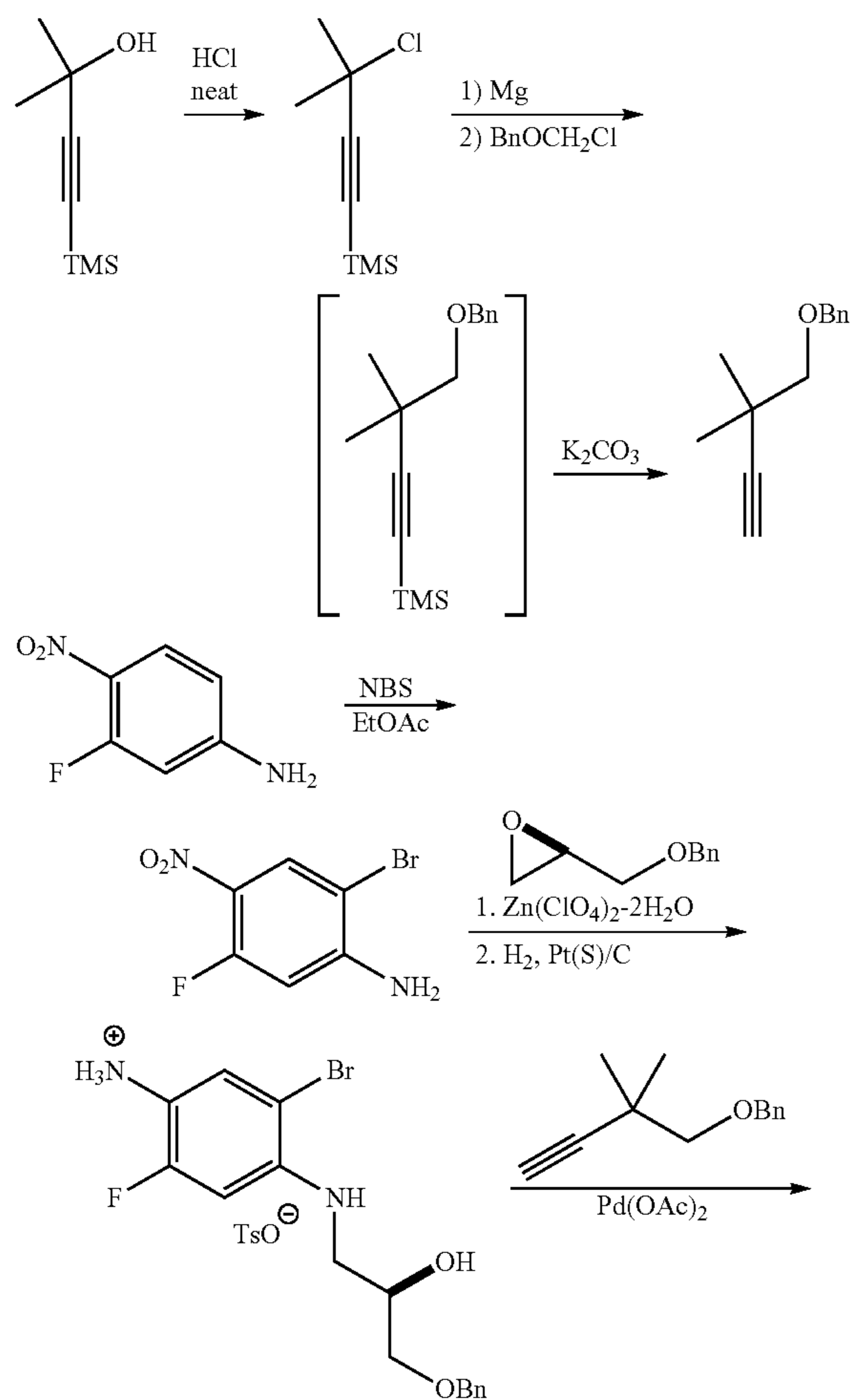
Scheme 3. Synthesis of the amine moiety.
