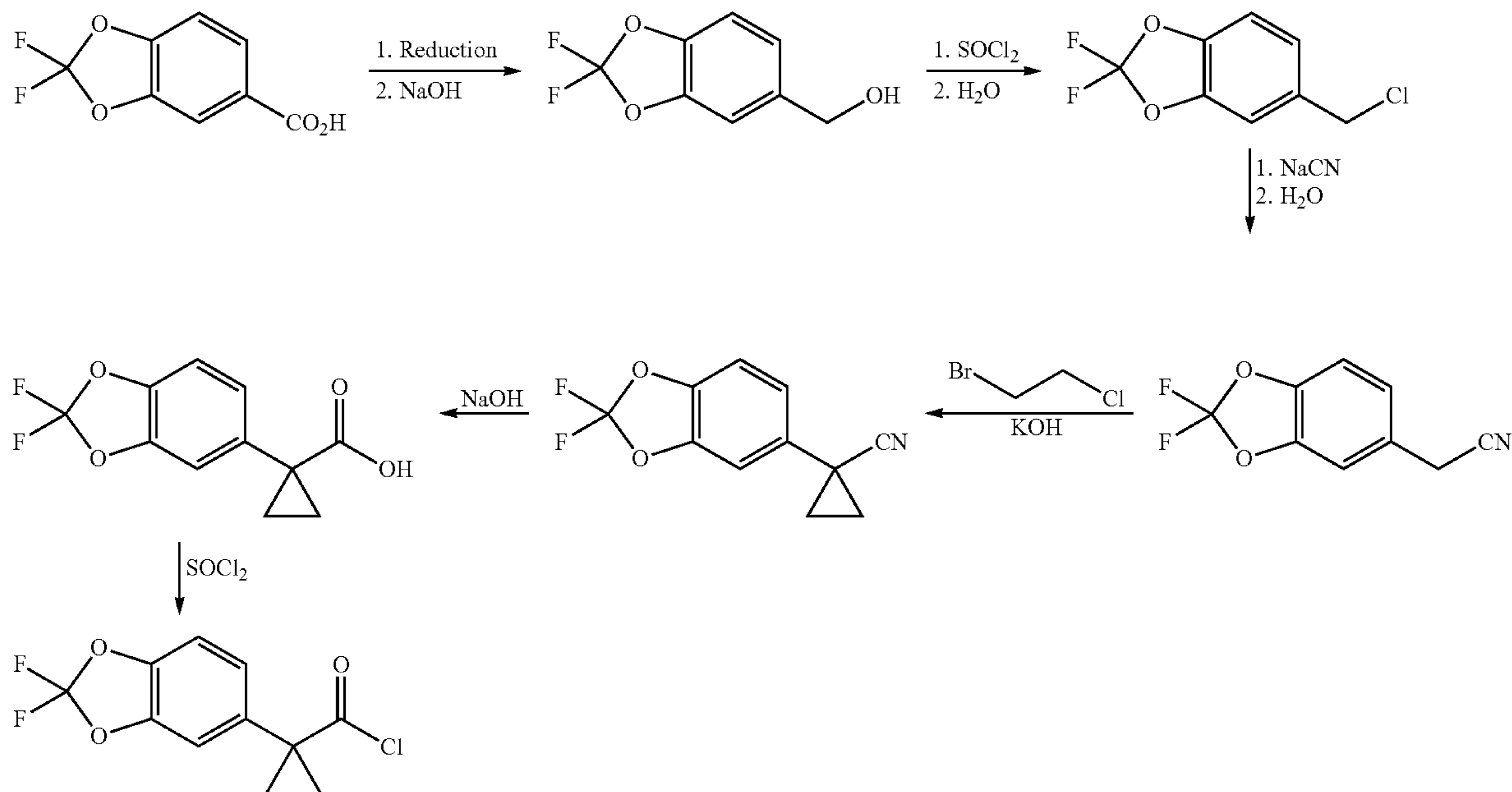
Scheme 1. Synthesis of the acid chloride moiety.
