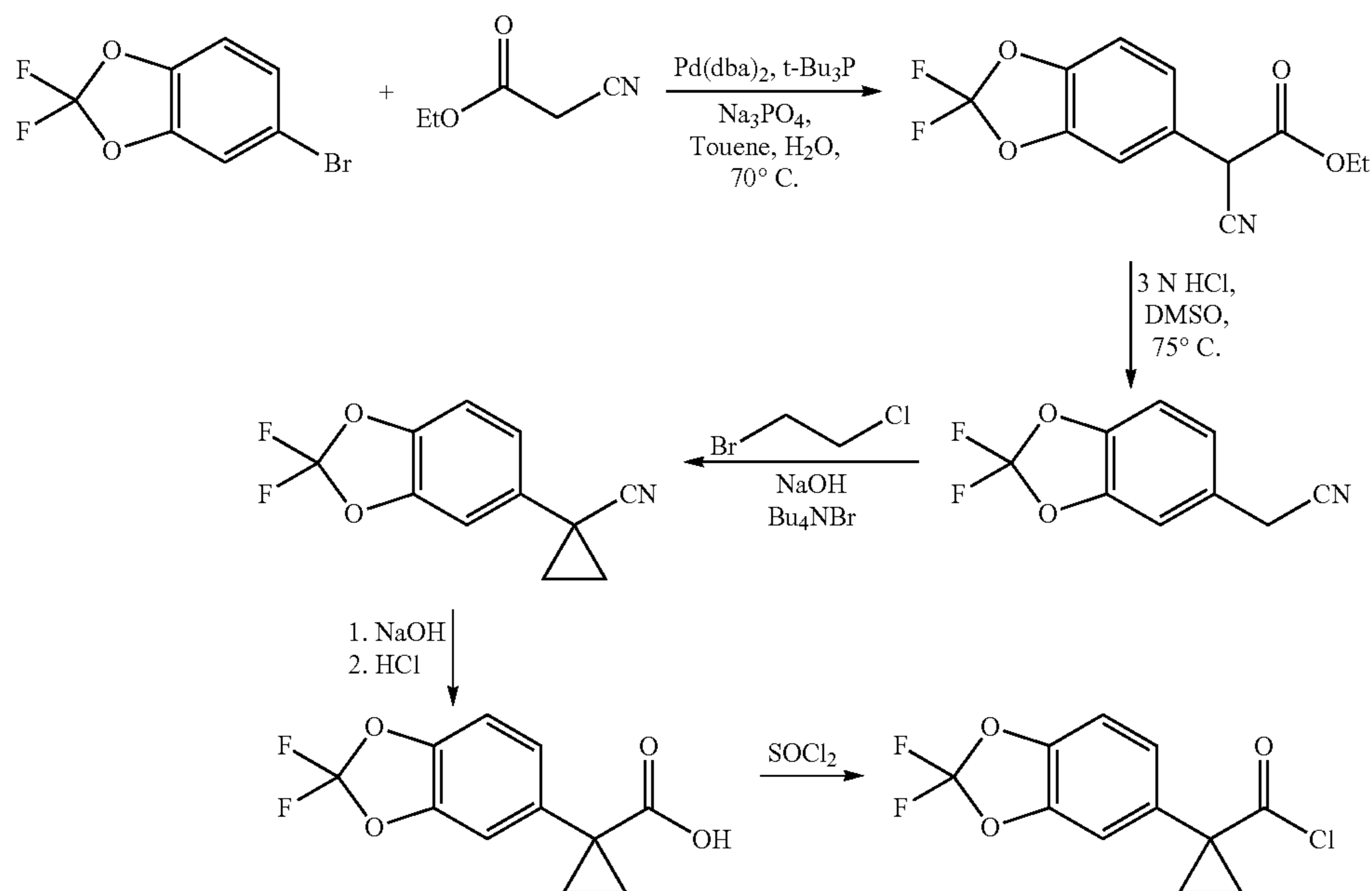
Scheme 2. Alternative synthesis of the acid chloride moiety.
