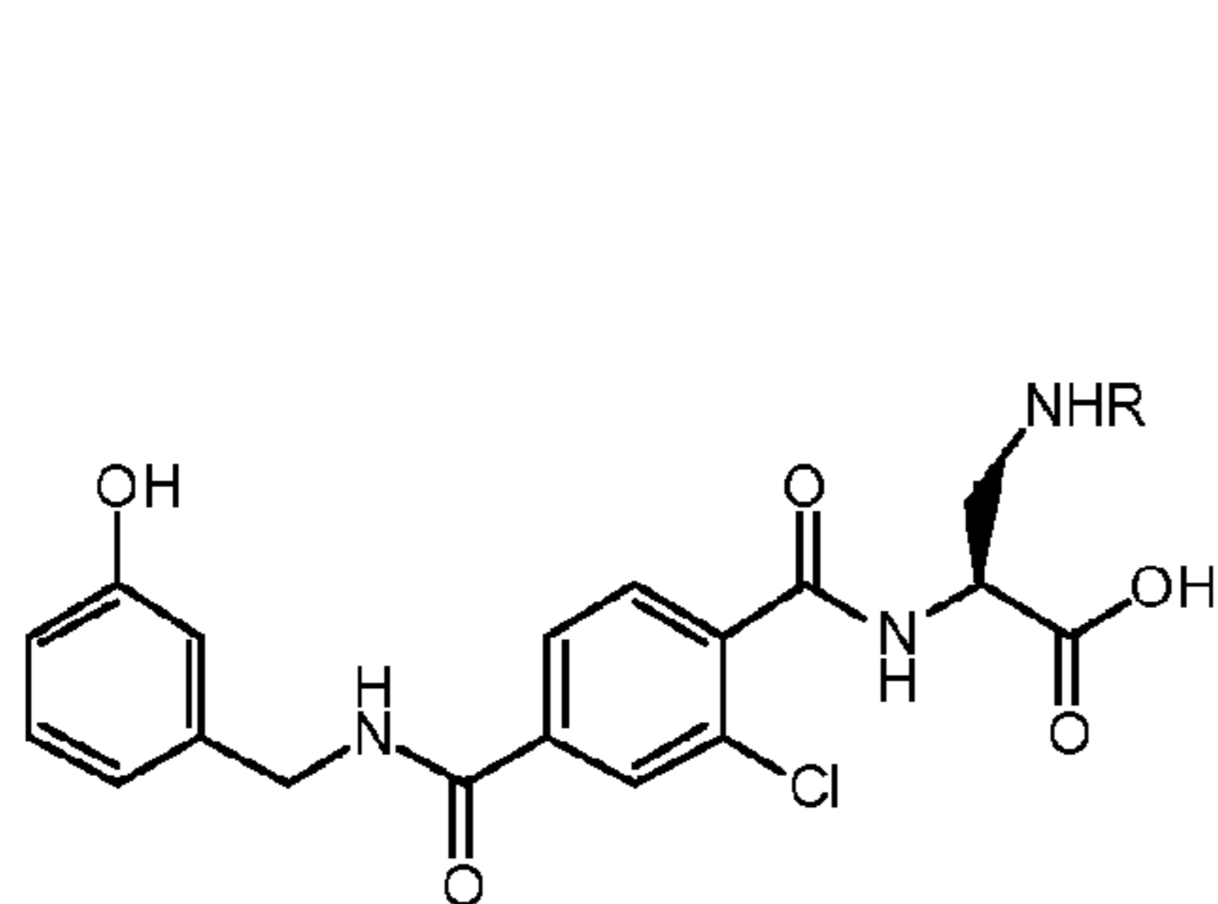
Compound 1, R = (C=S)NH-Fluorescein
