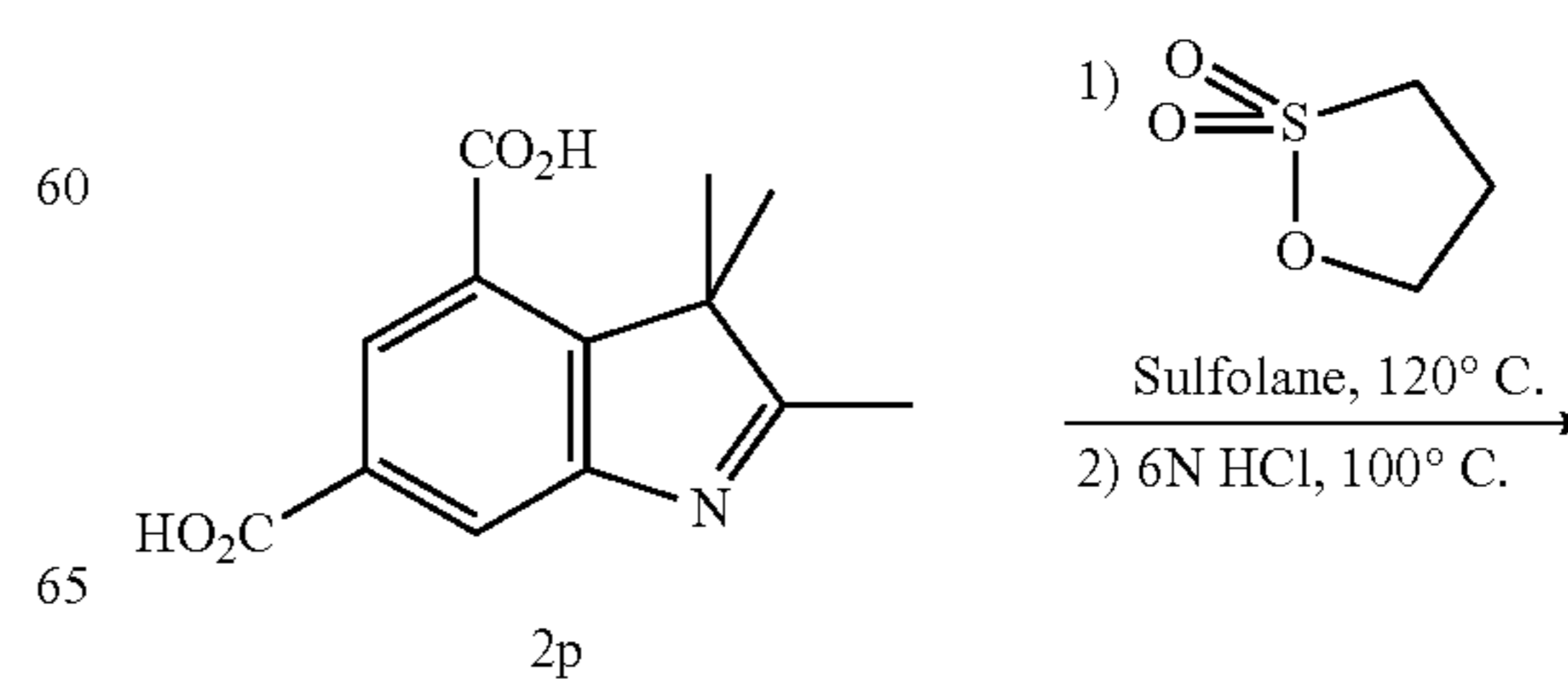
Scheme 3: Synthesis of carboxyl indolenine cyanine dyes
