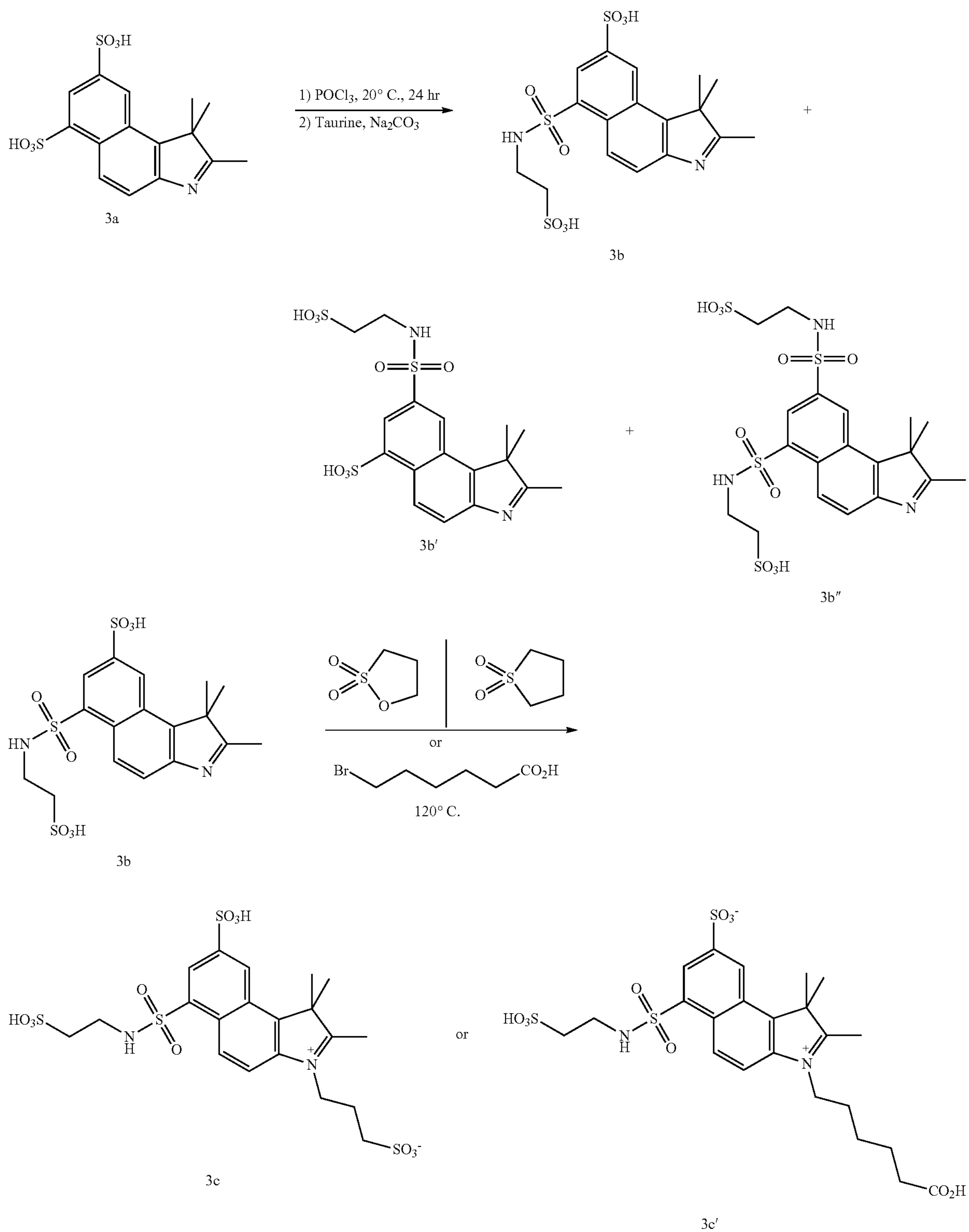
Scheme 5: Synthesis of taurine amide benzindole cyanine dyes
