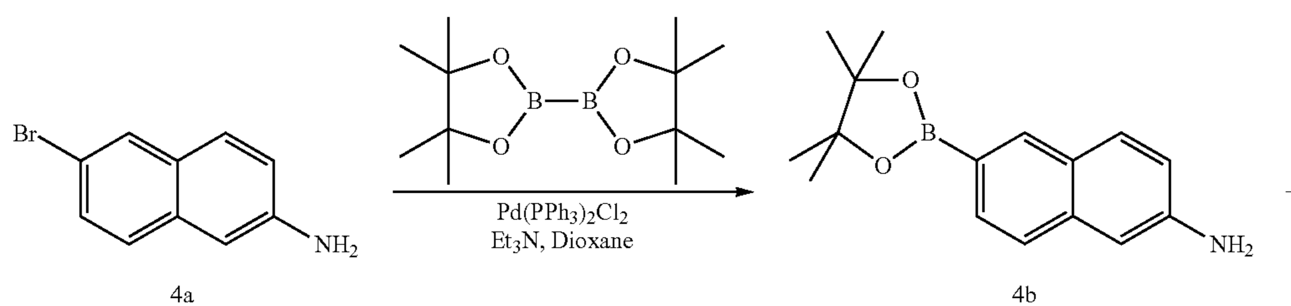
Scheme 6: Synthesis of pyridyl benzindole cyanine dyes
