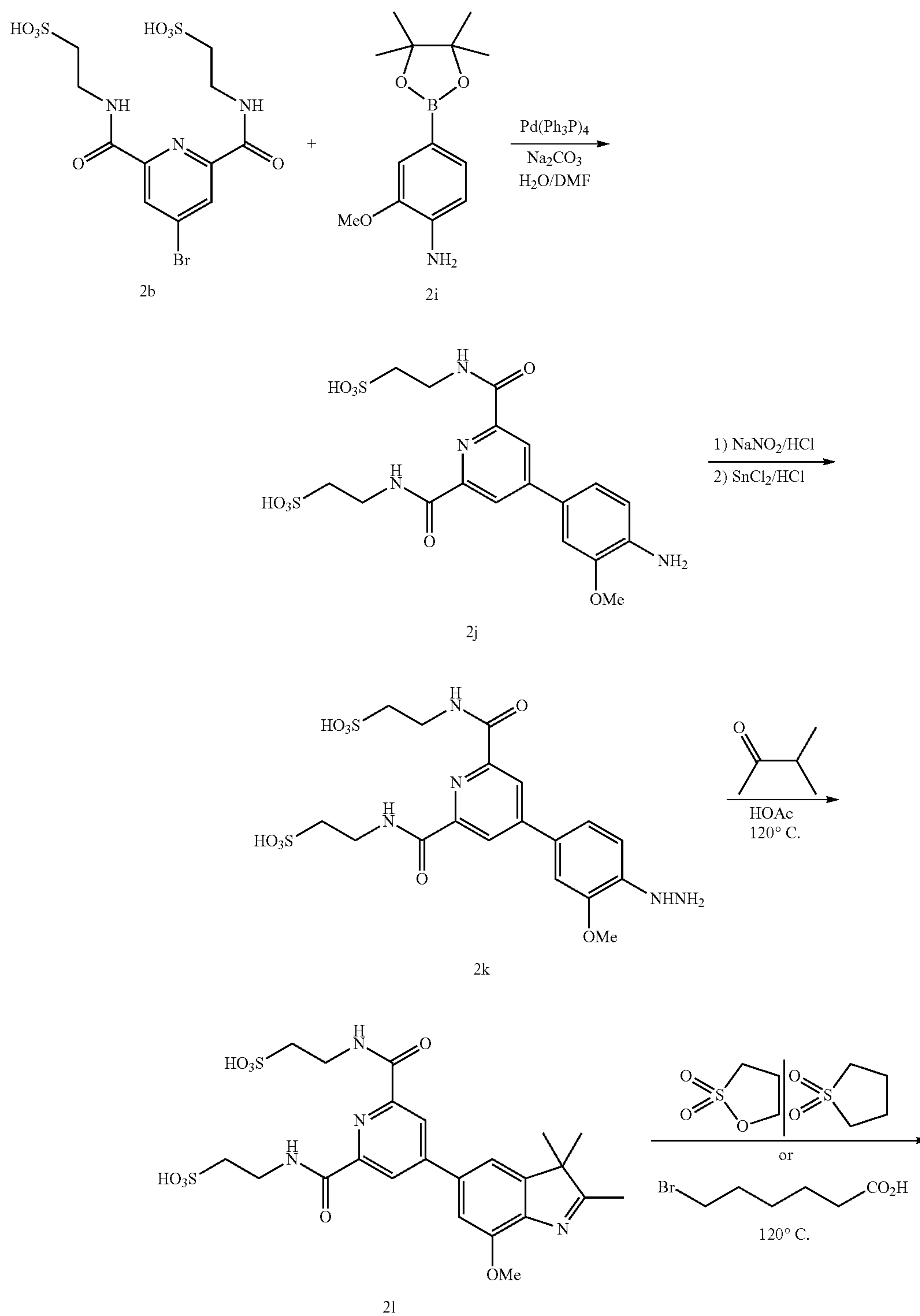
Scheme 2: Synthesis of pyridyl methoxyindolenine cyanine dyes
