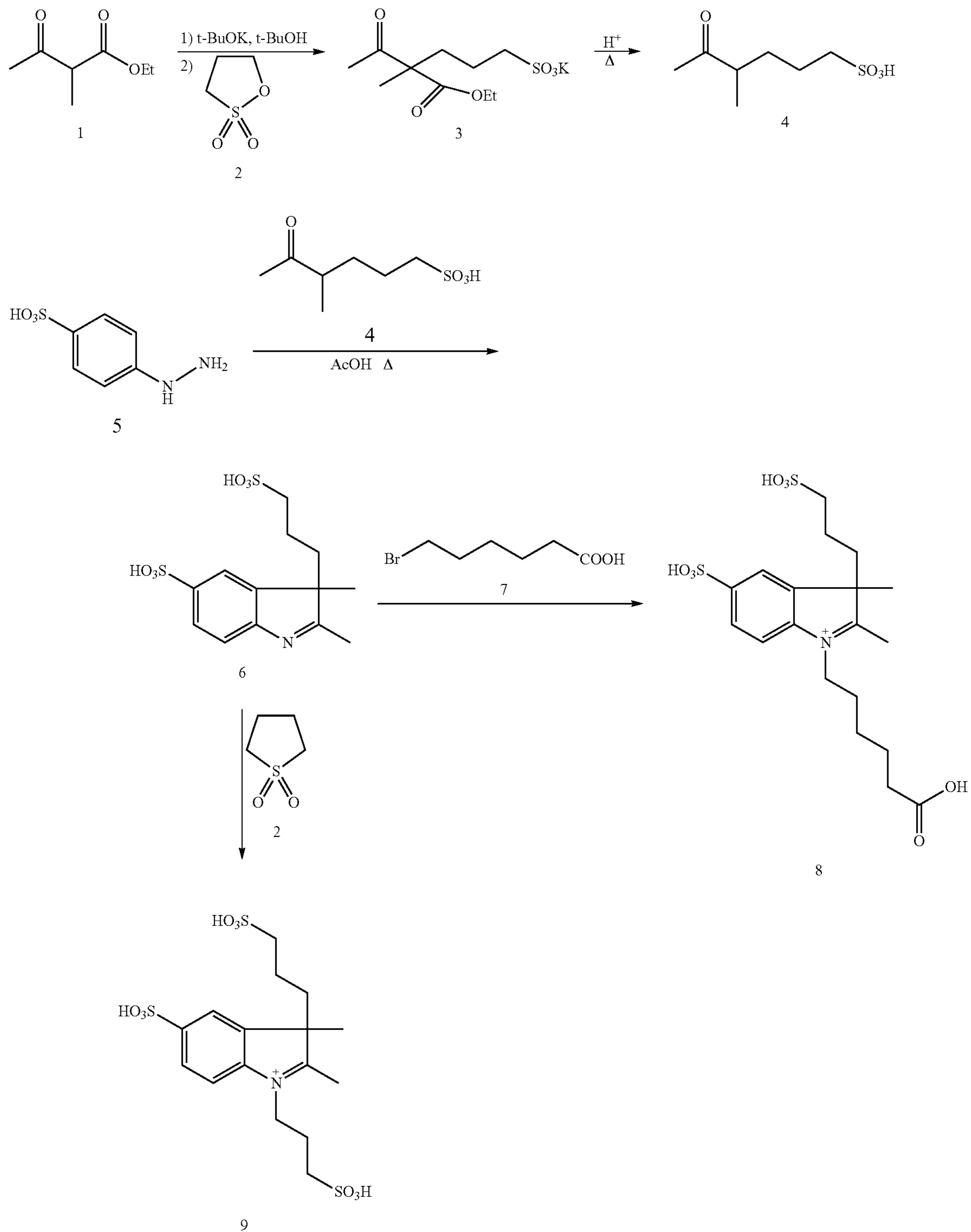
Scheme 1. Synthesis of Pentasulfonated Cyanine Dyes
