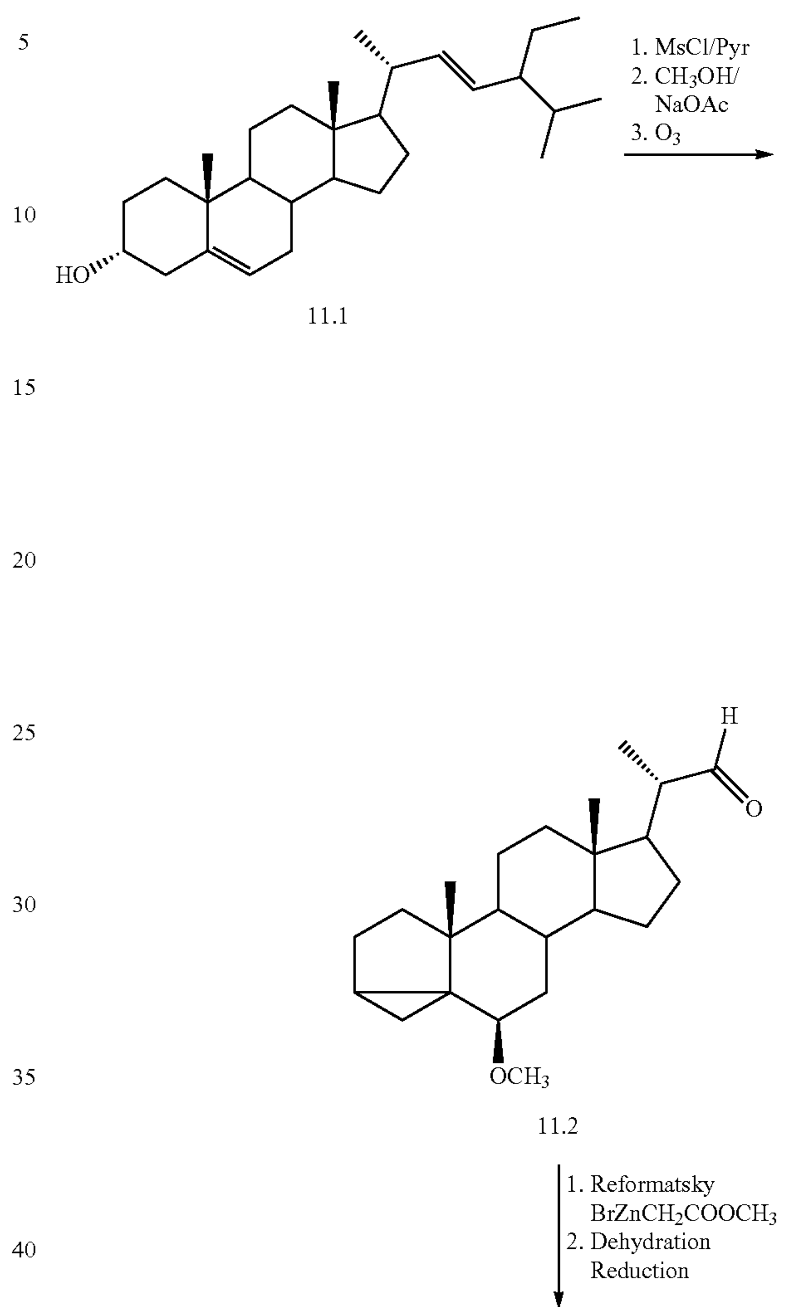
Scheme 11. Ozonolysis of i-steroid and side chain reduction
