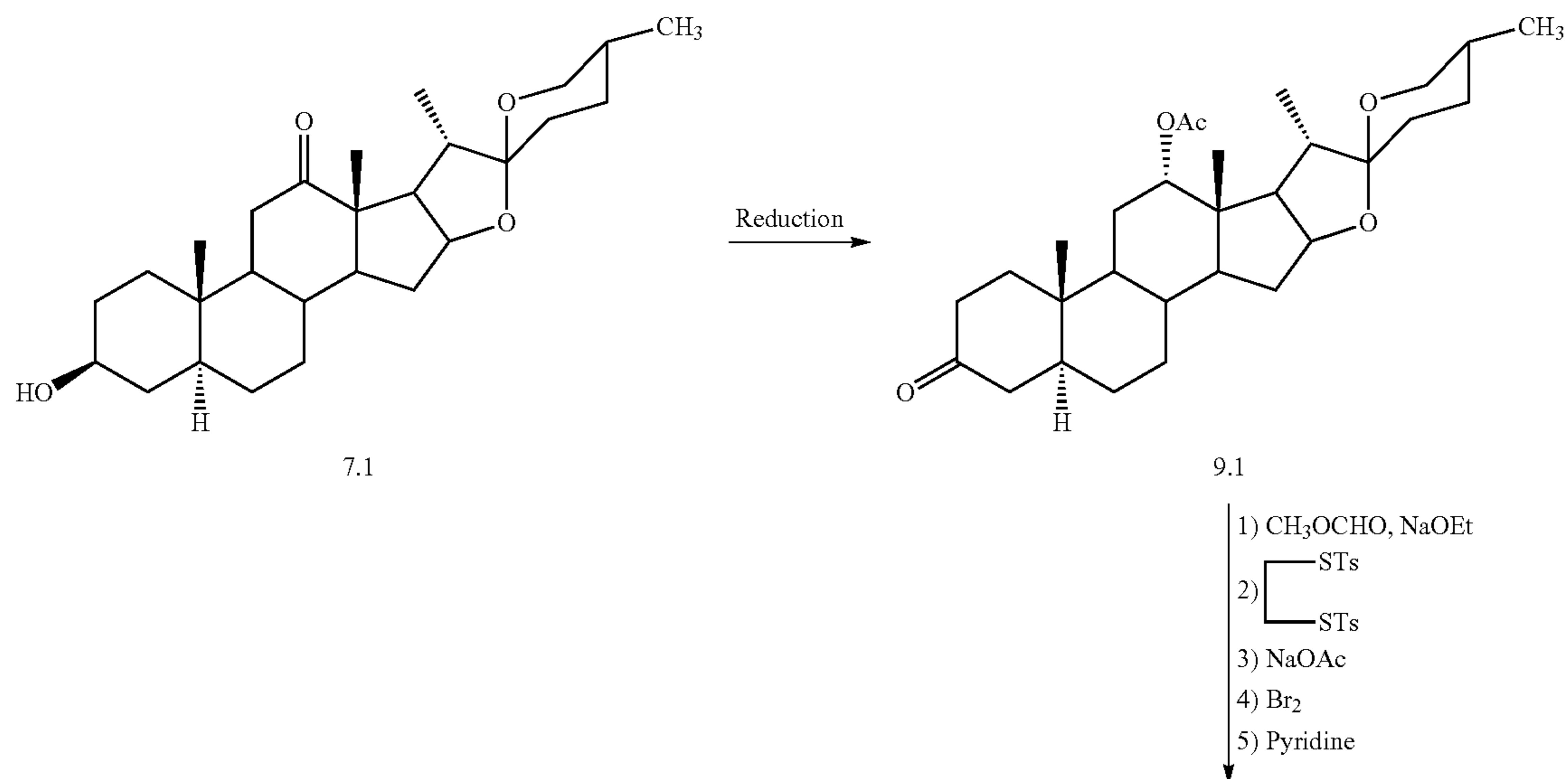
Scheme 9. Dithioethane route to 3-keto-4-ene
