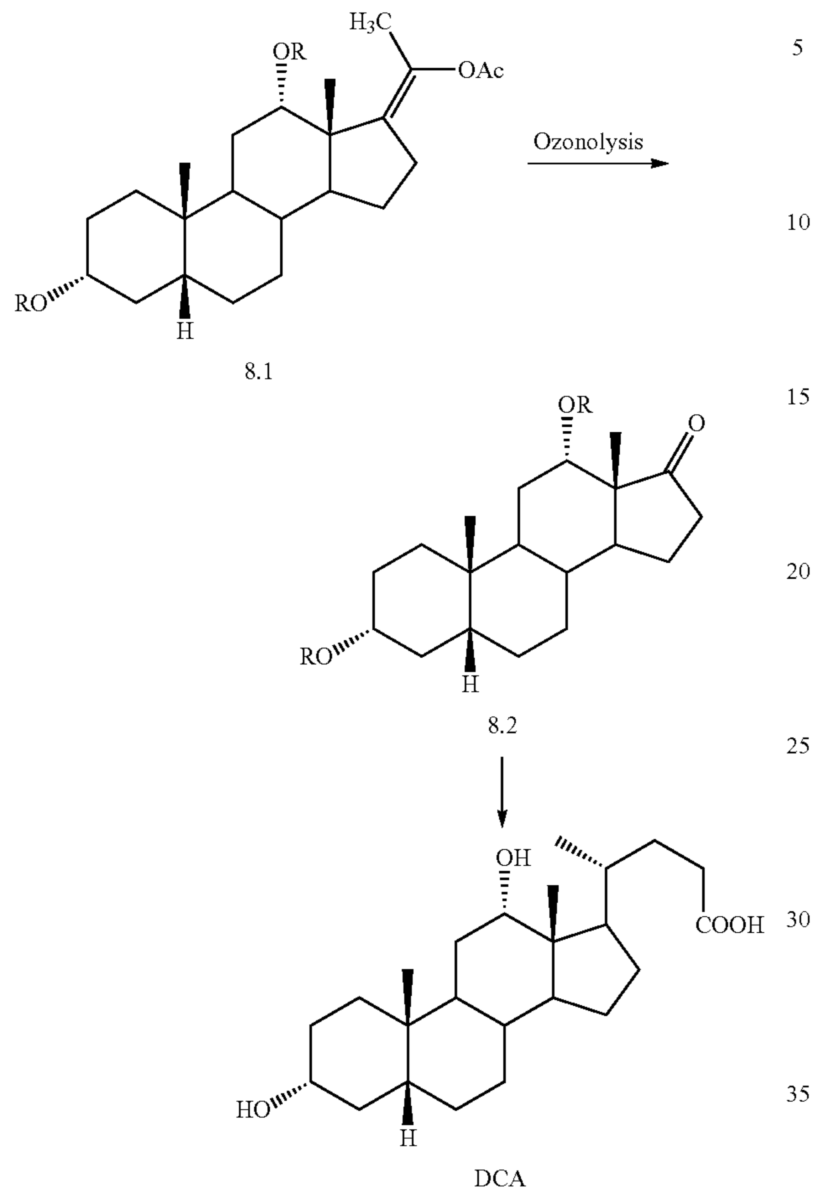
Scheme 8. Side-chain introduction
