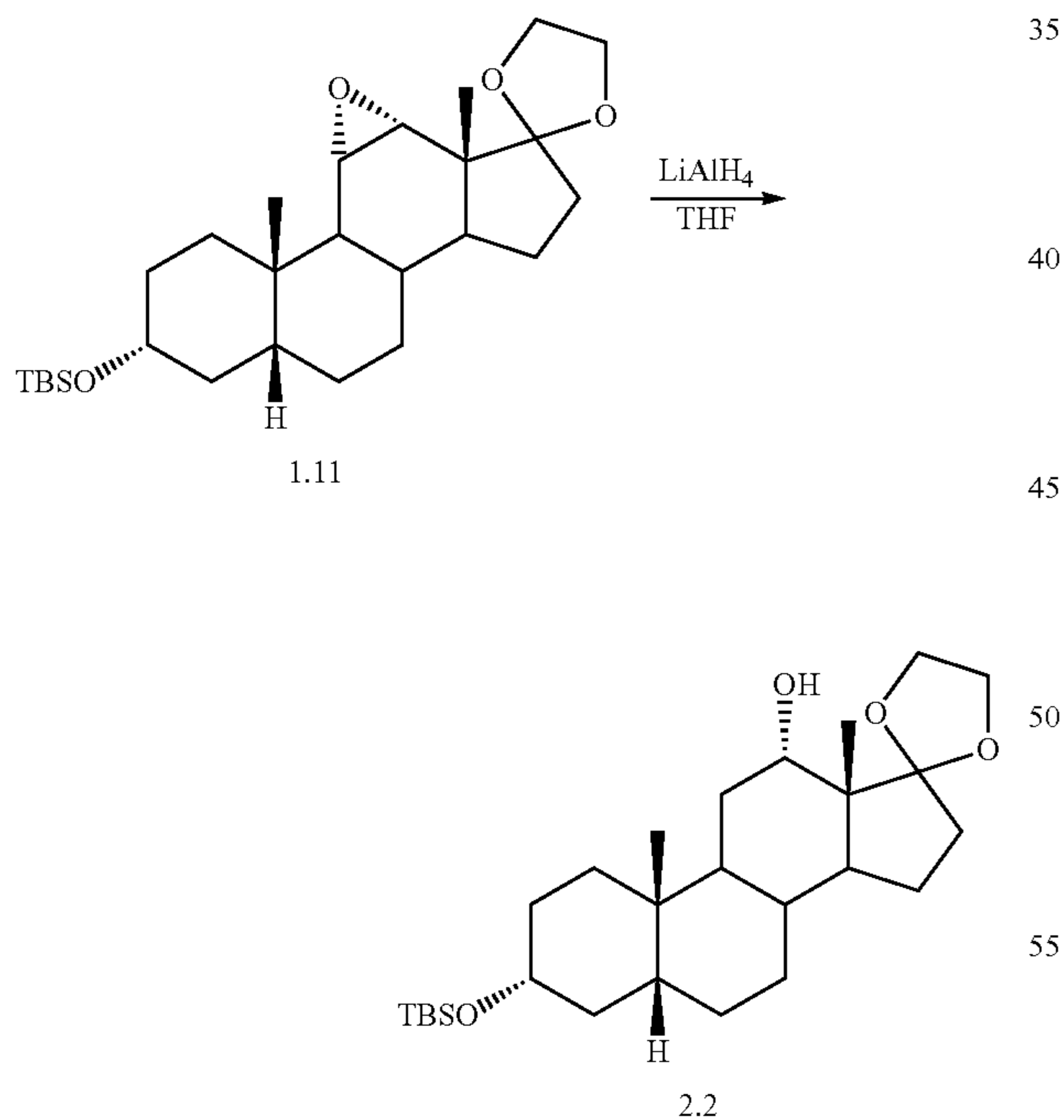
Scheme 3. Stereoselective Reduction of C 11 -C 12 epoxide.
