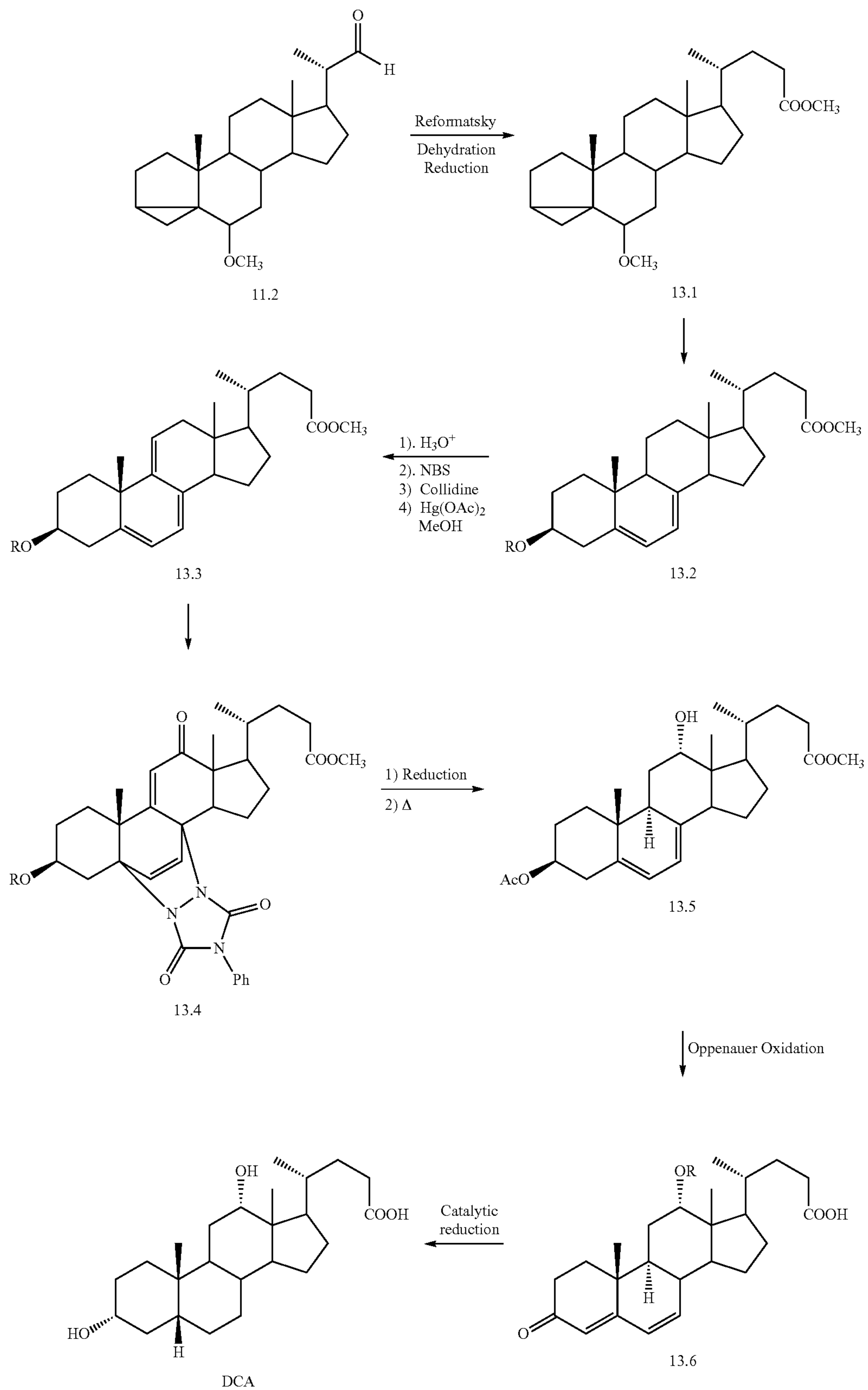
Scheme 13. Triene Formation and Diels-Alder Protection of the Ring B Diene.
