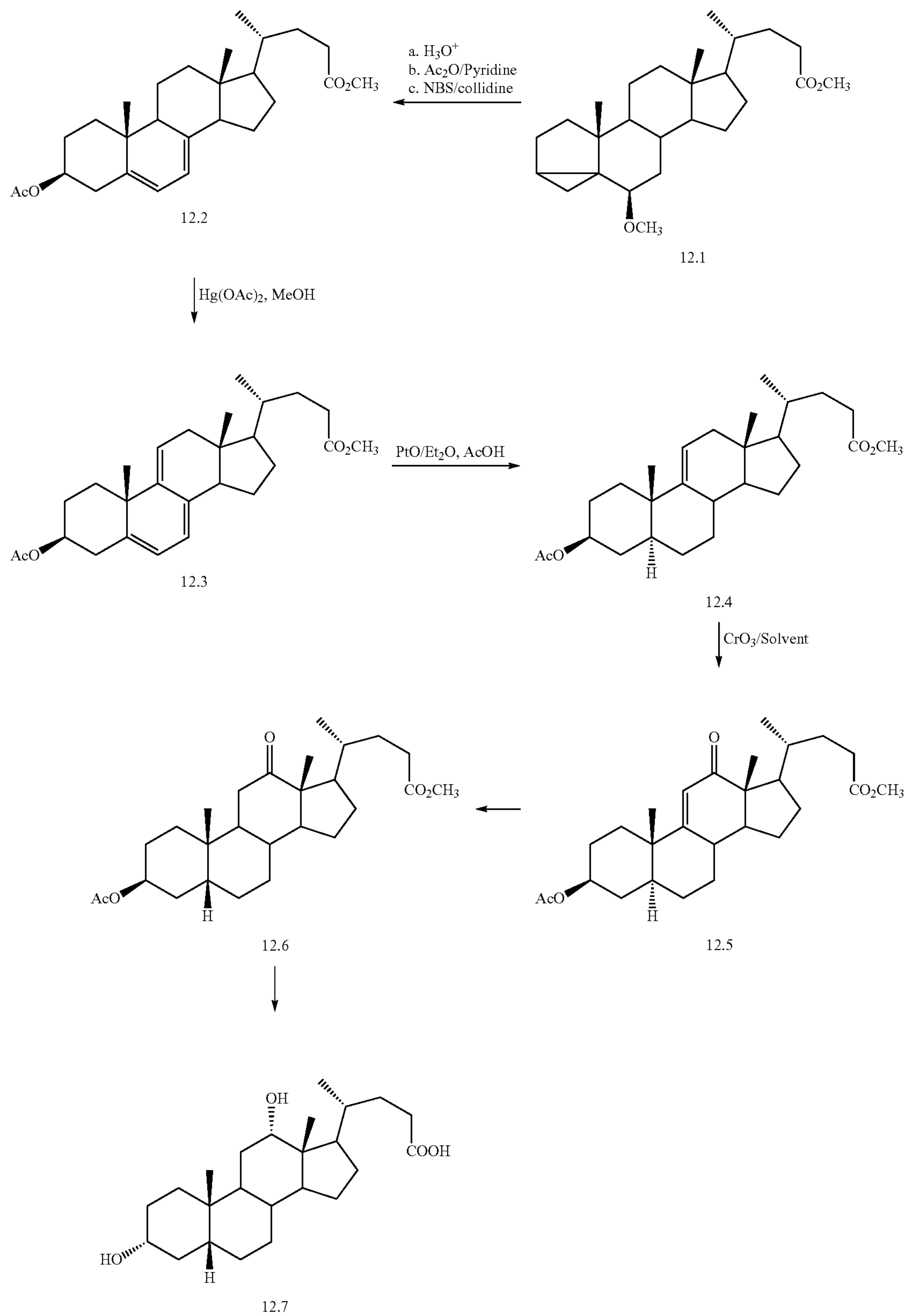
Scheme 12. Triene formation and allylic oxidation
