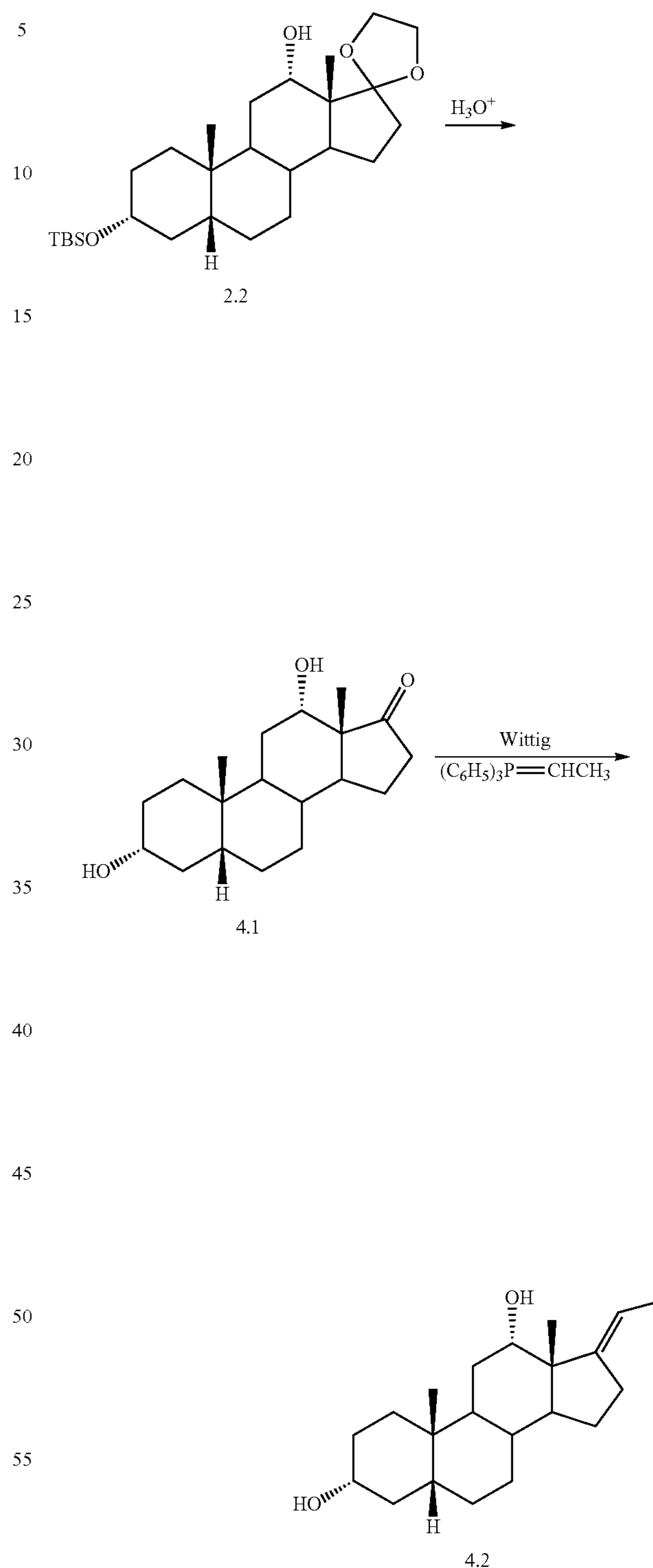
Scheme 4. Deprotection and Wittig Reaction
