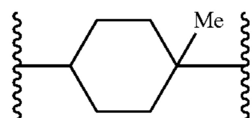
4-methyl-cyclohexane-1,4-di-yl
