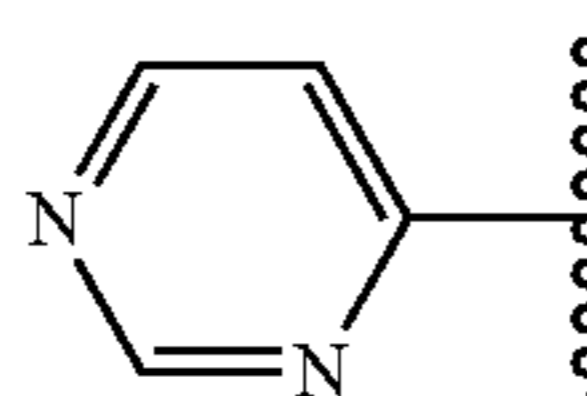
pyrimidin-4-yl
