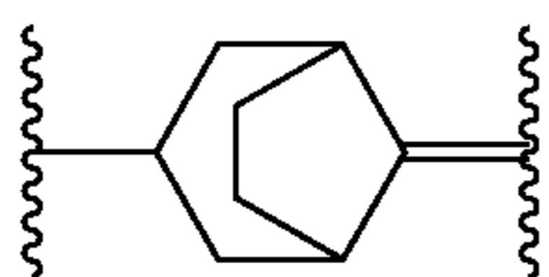
bicyclo[3.2.1]octane-3-yl-8-ylidene
