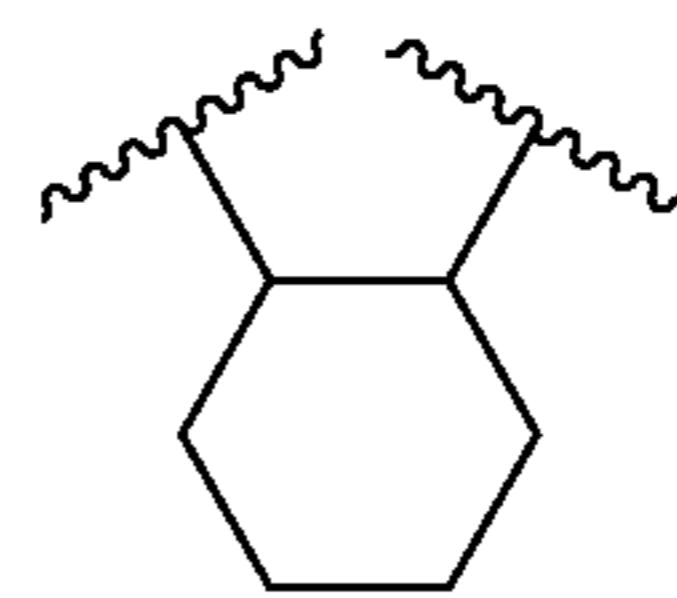
cyclohexane-1,2-di-yl
