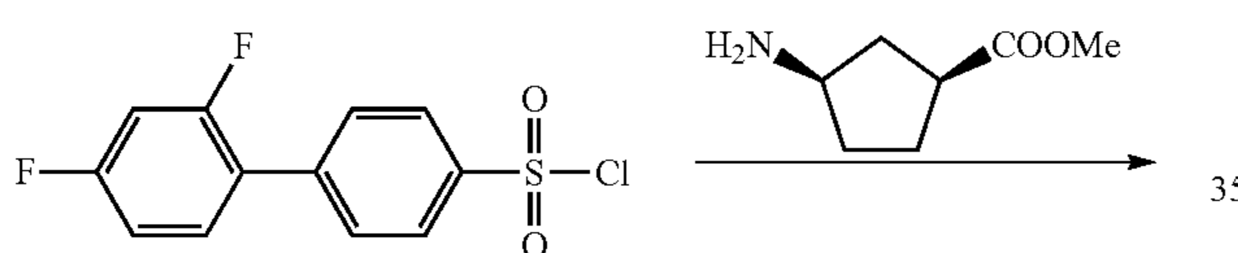
Scheme 7
