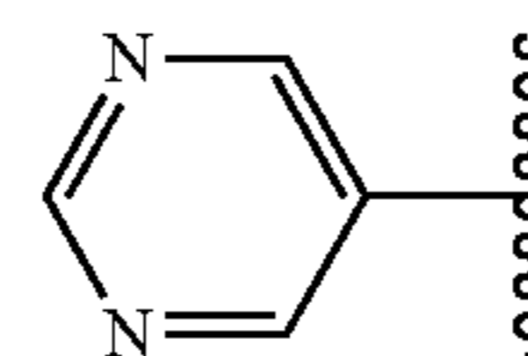
pyrimidin-5-yl
