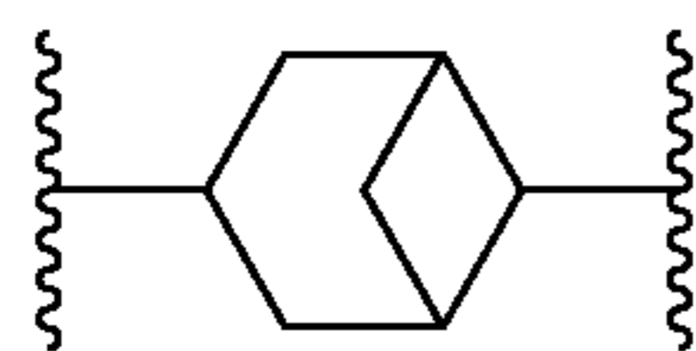
bicyclo[3.1.1]heptane-3-yl-6-ylidene
