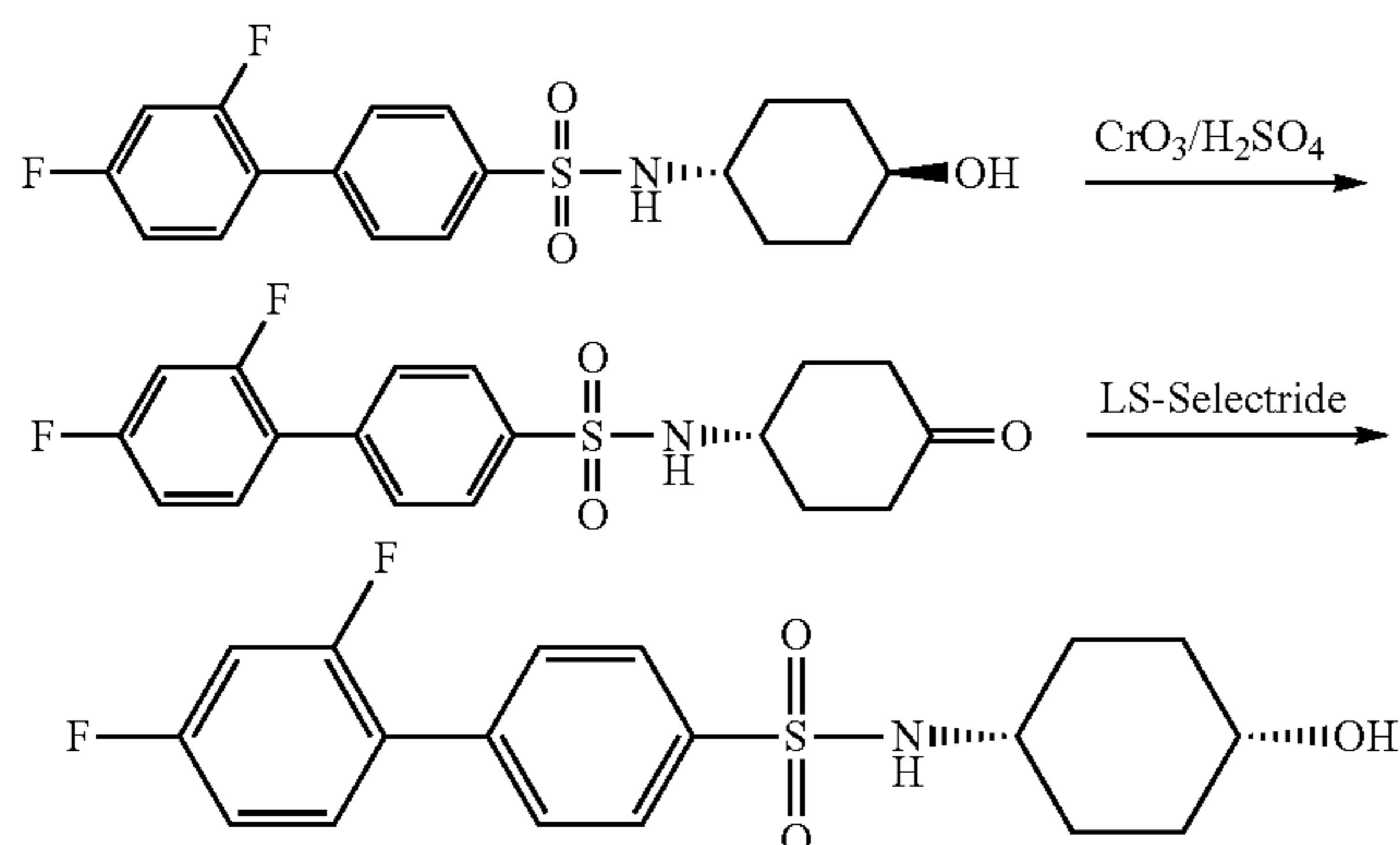
Scheme 14
