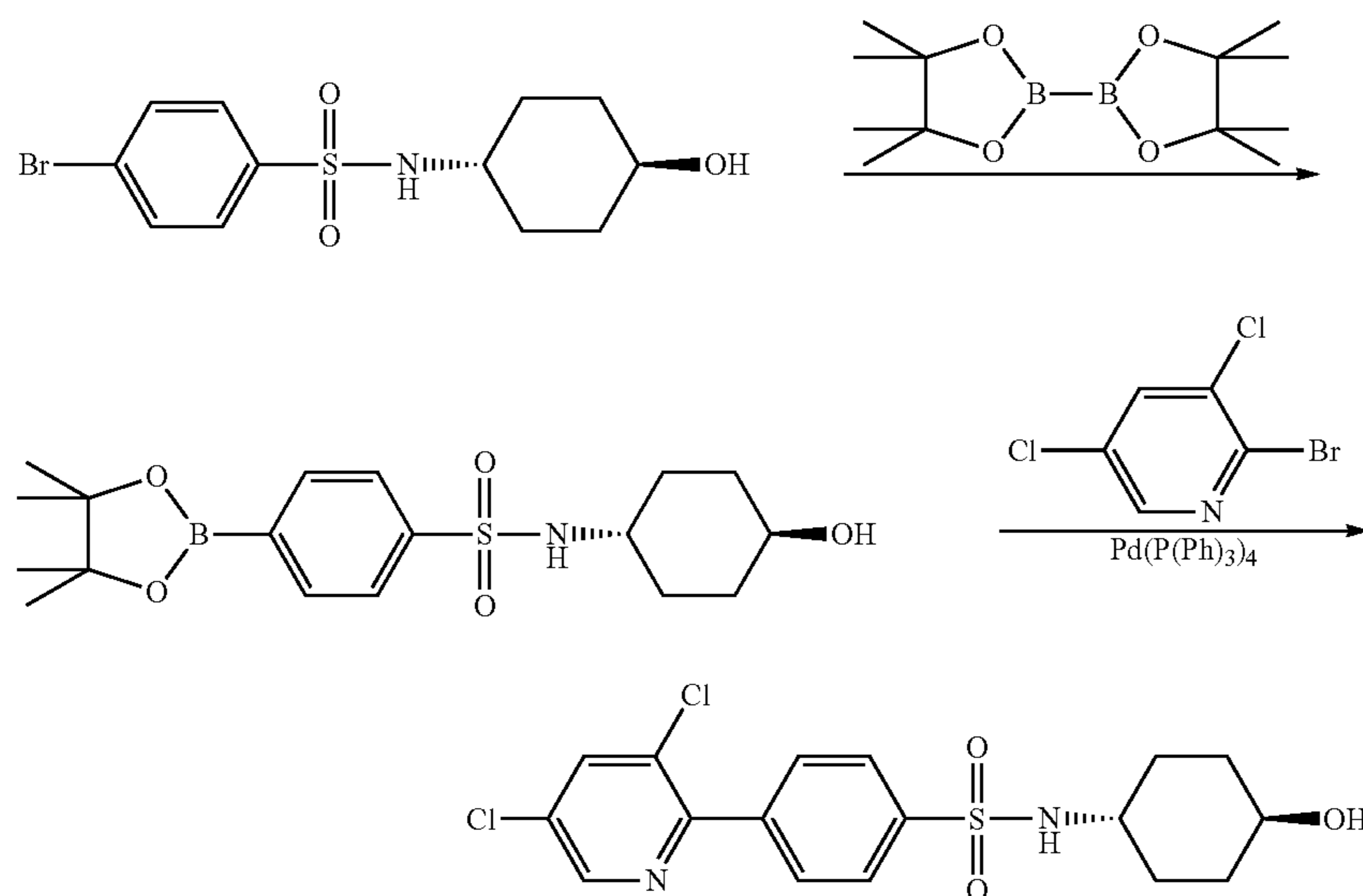
Scheme 18
