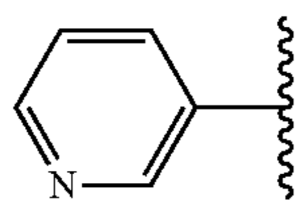
pyridin-3-yl
