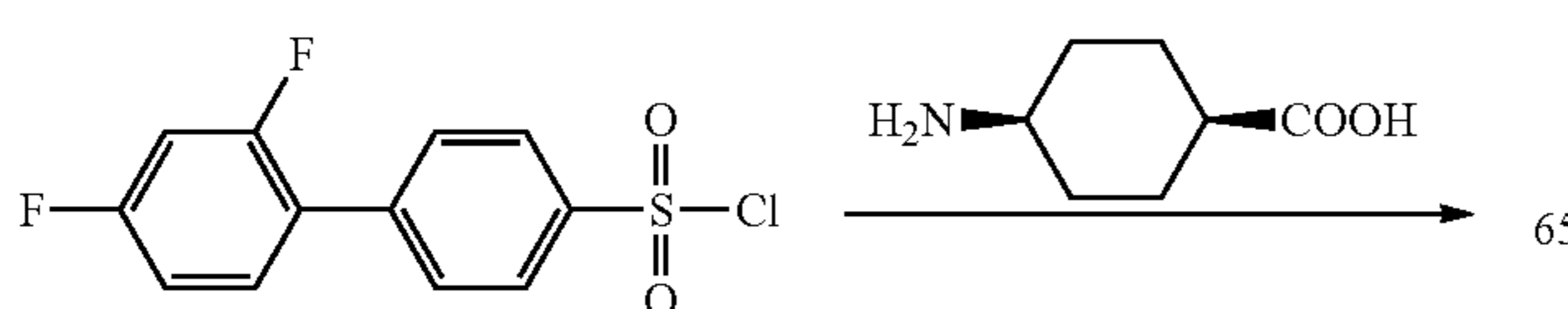
Scheme 8
