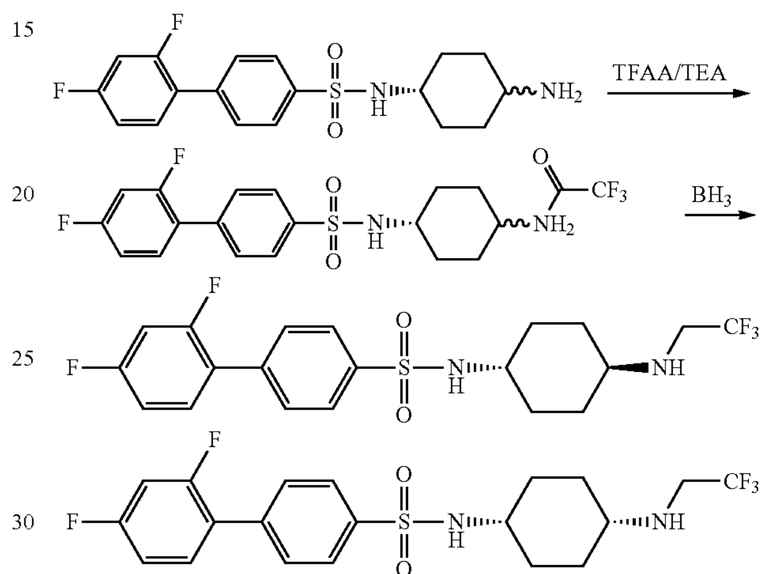
Scheme 13
