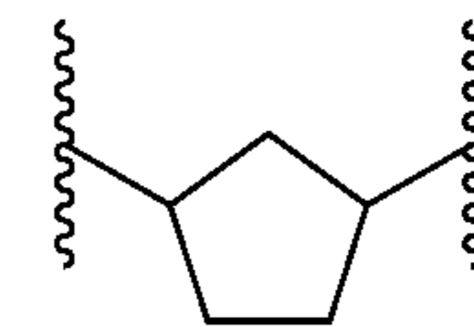
cyclopentane-1,3-di-yl
