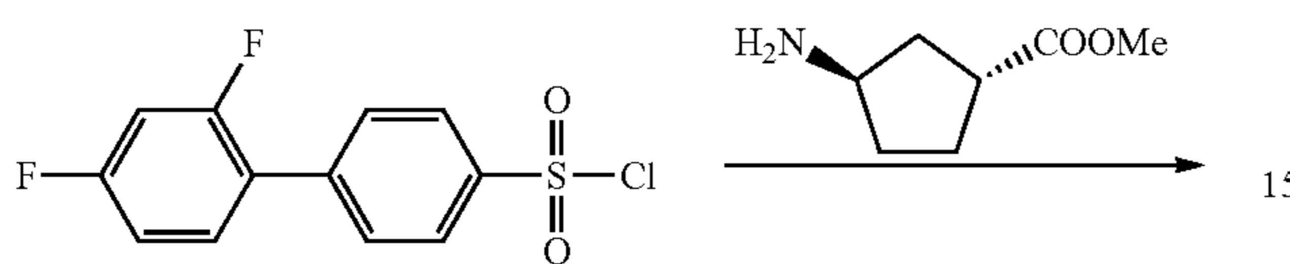
Scheme 6
