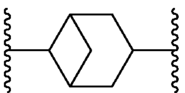
bicyclo[3.1.1]heptane-6-yl-3-ylidene
