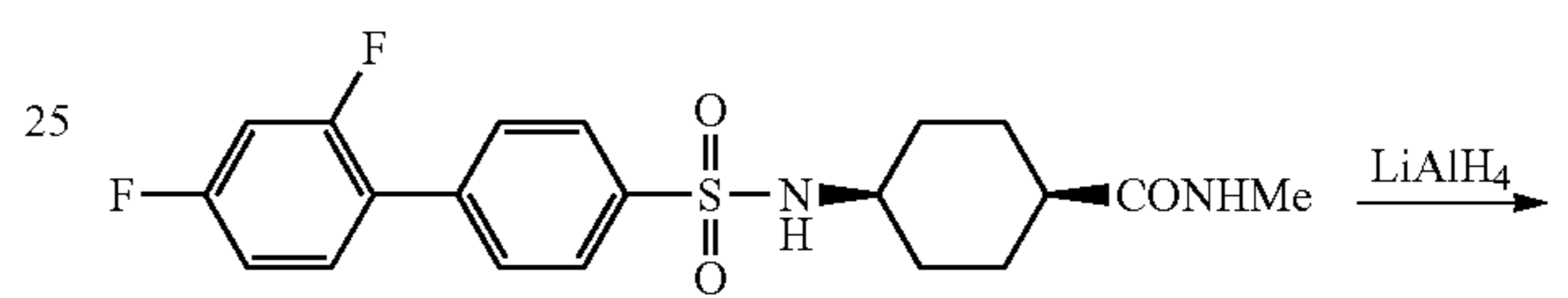
Scheme 9
