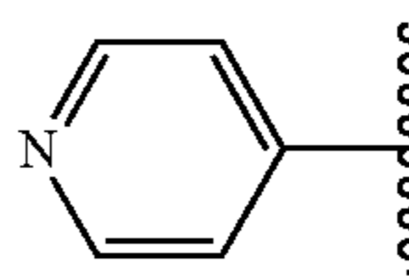
pyridin-4-yl
