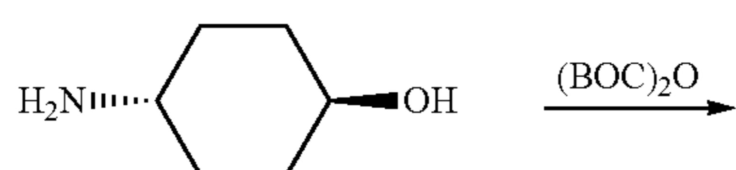
Scheme 16
