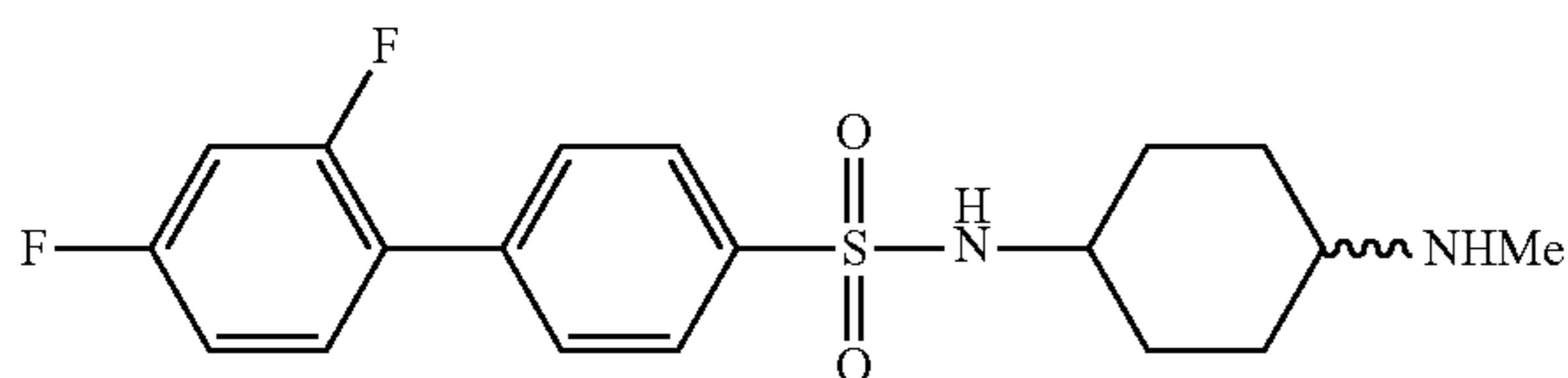
2',4'-Difluoro-N-(4-(methylamino)cyclohexyl)biphenyl-4-sulfonamide (ABD816)
