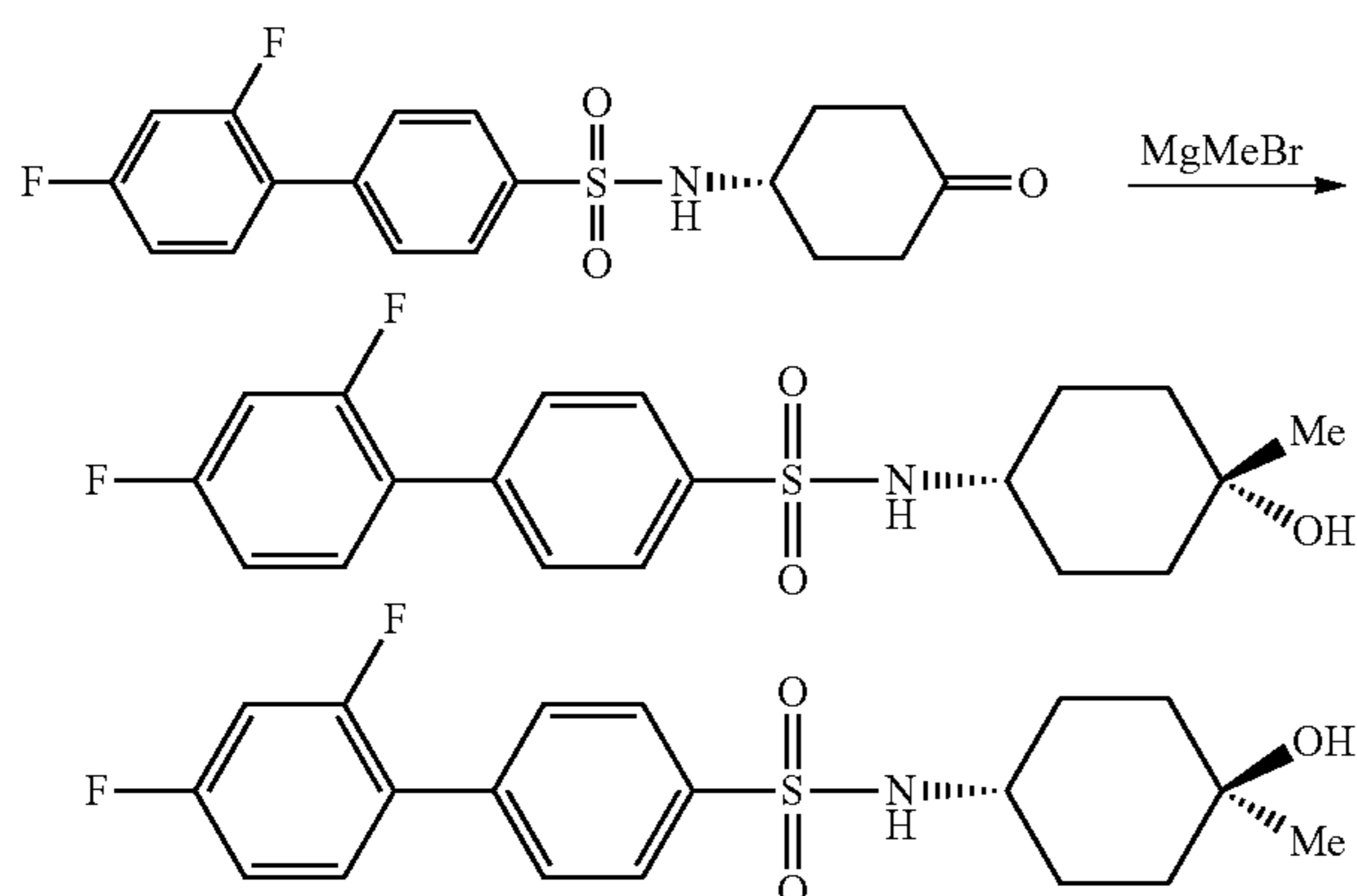
Scheme 15
