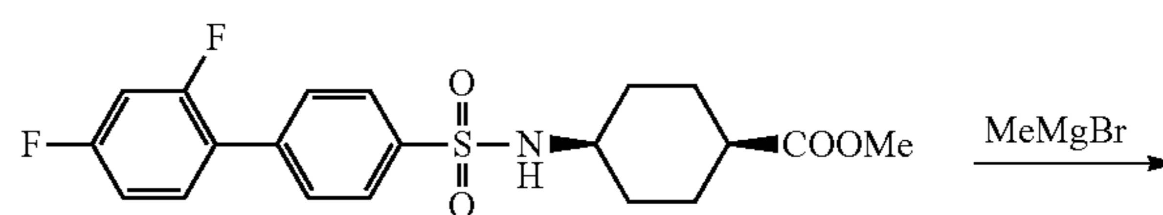
Scheme 17
