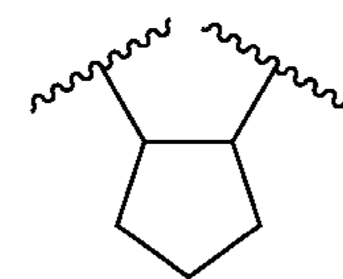
cyclopentane-1,2-di-yl
