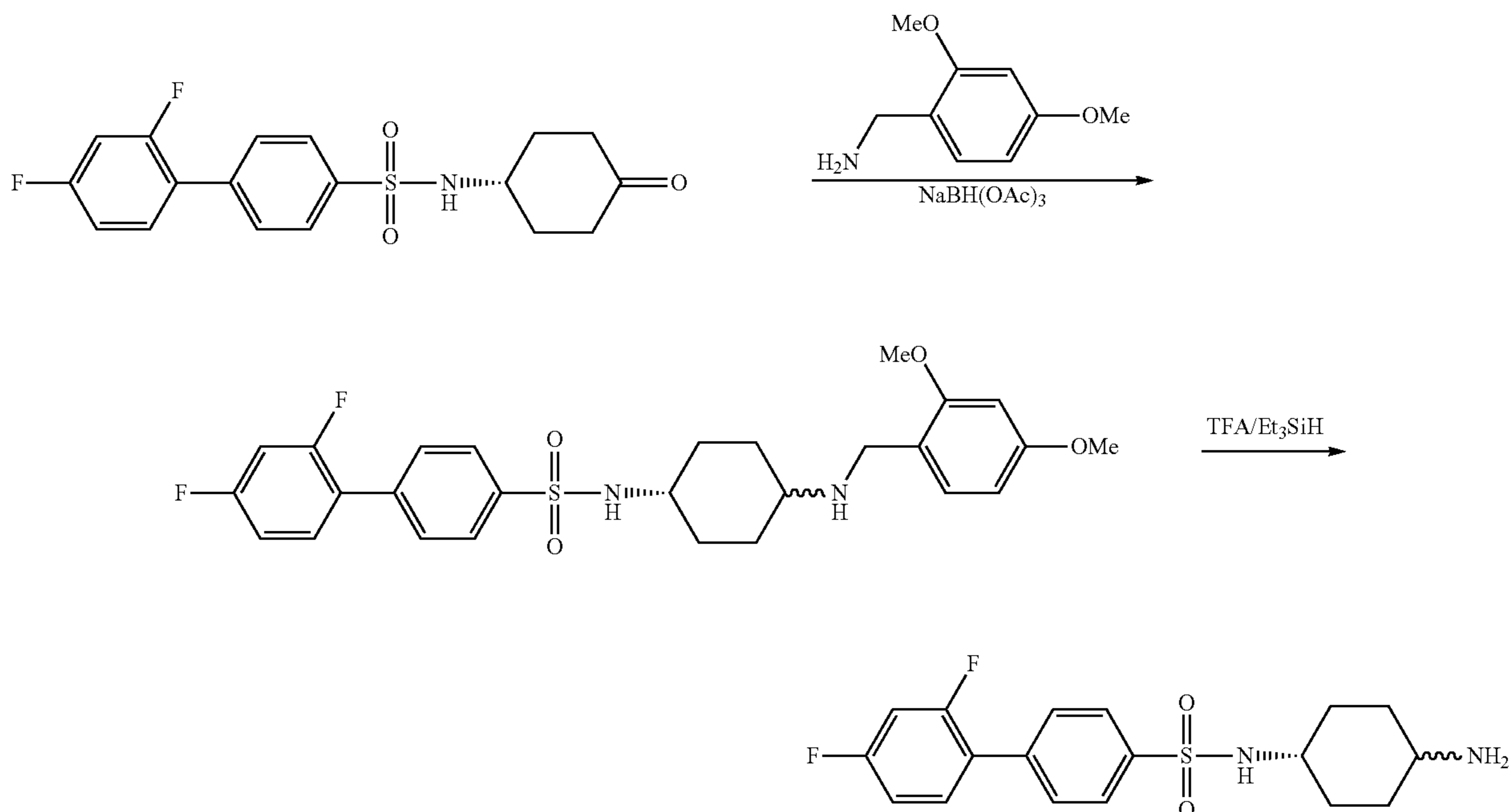
Scheme 12
