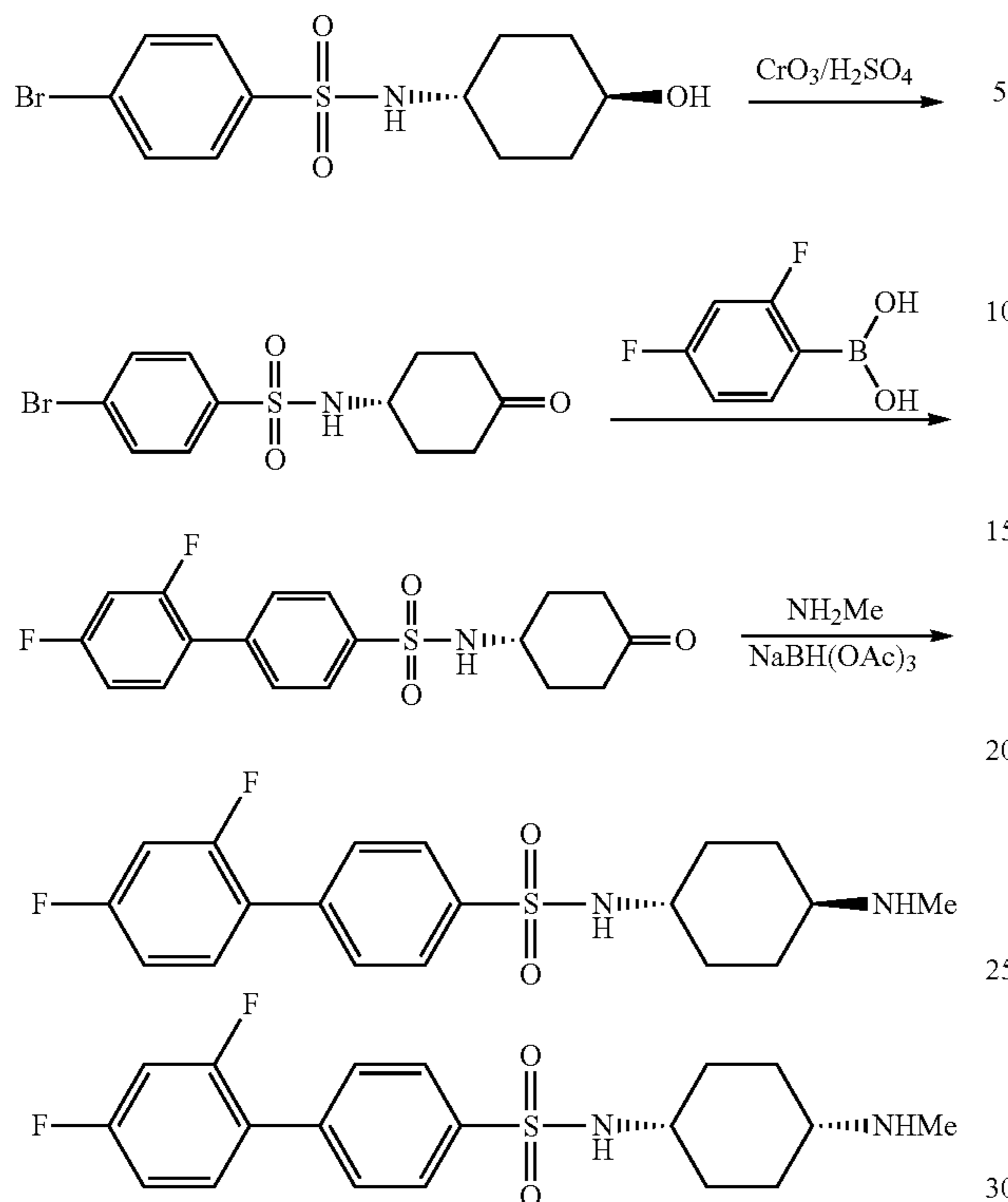
Scheme 11
