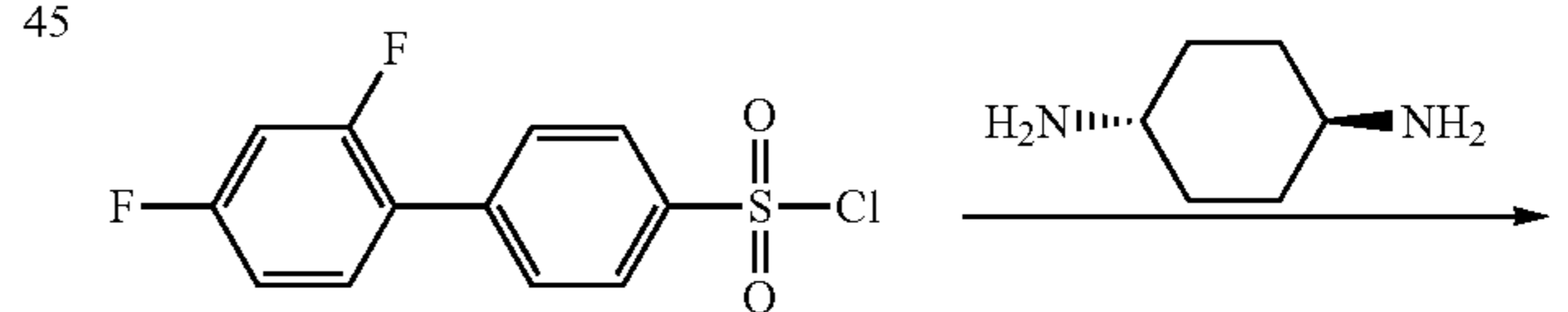
Scheme 10
