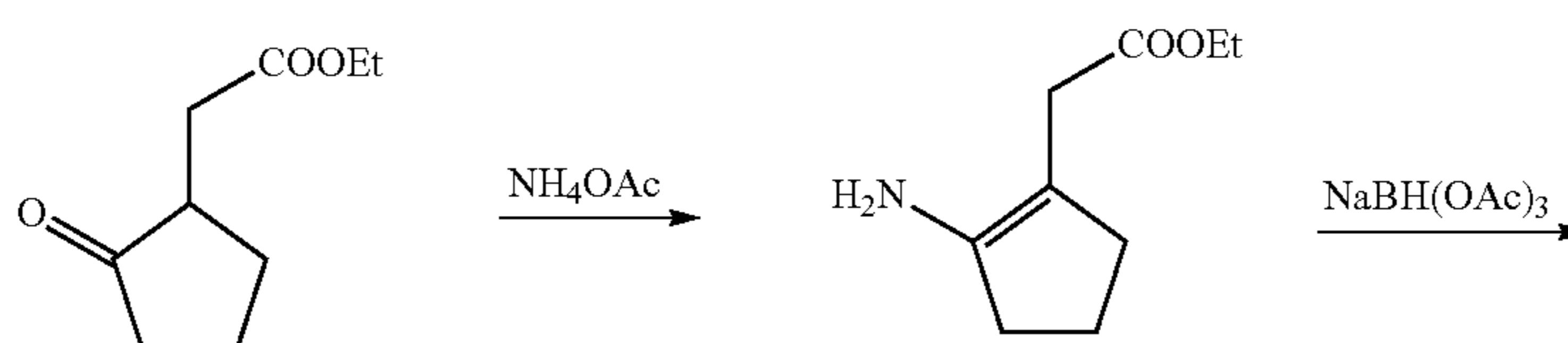
Scheme 20
