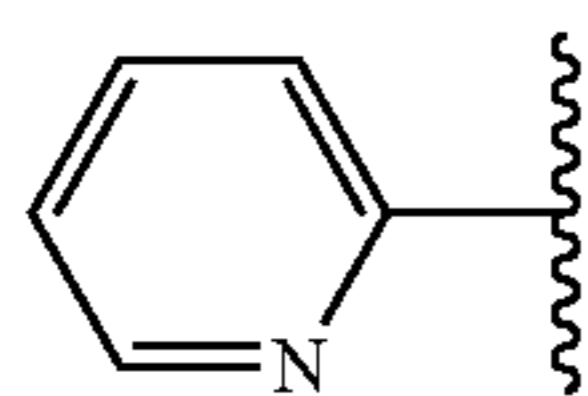
pyridin-2-yl
