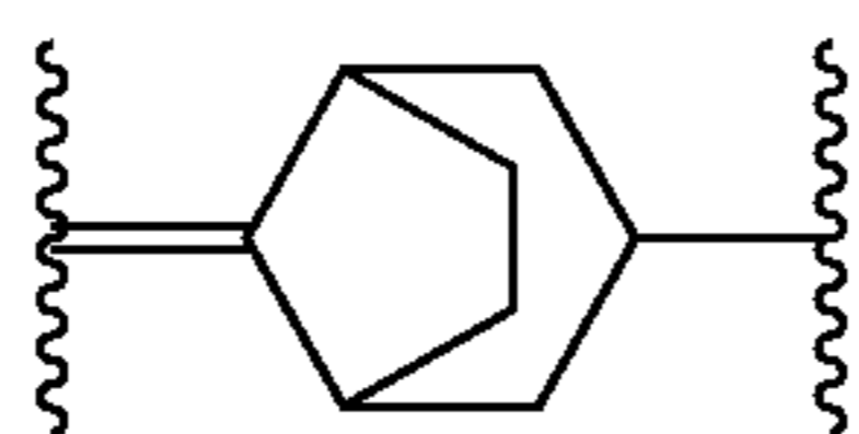
bicyclo[3.2.1]octane-8-yl-3-ylidene
