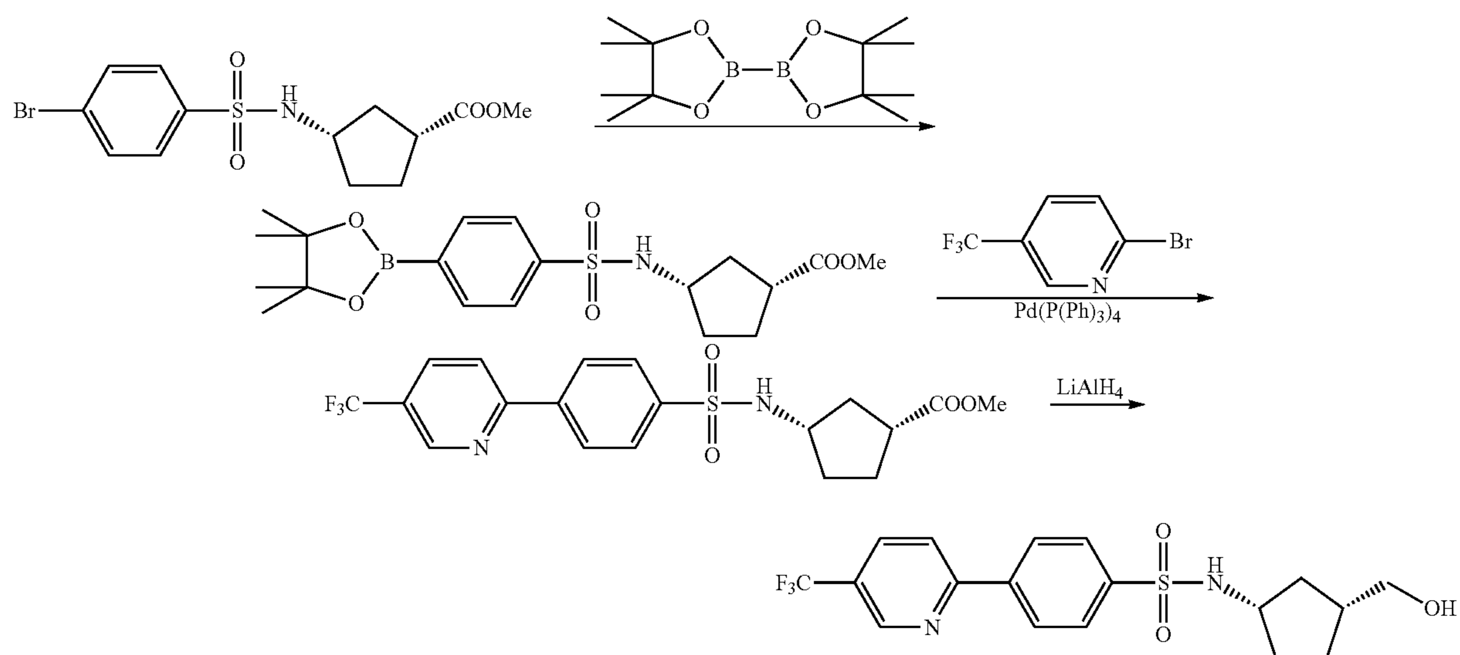
Scheme 19
