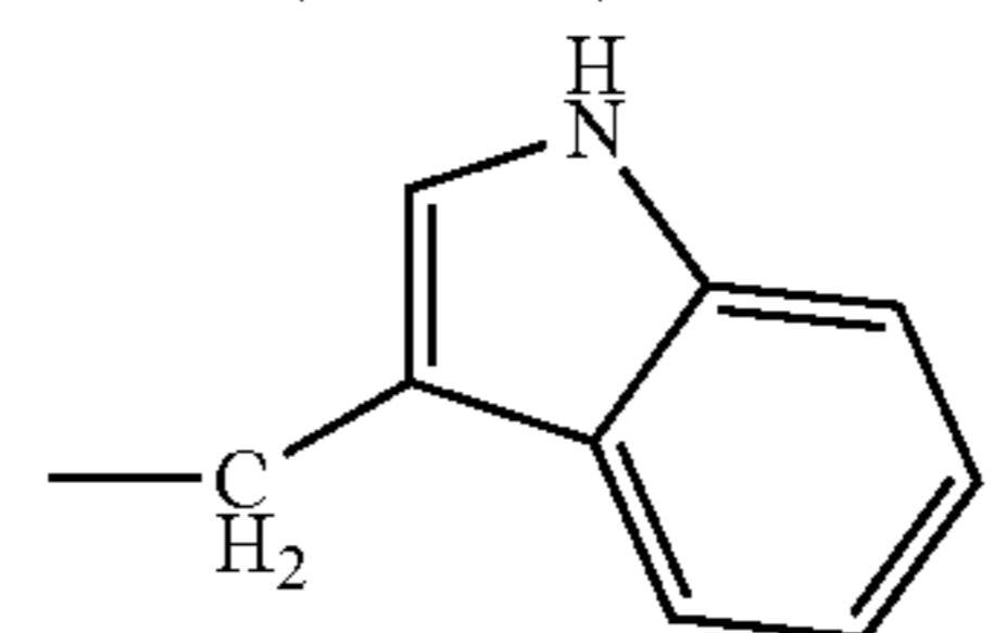
(tryptophan)
