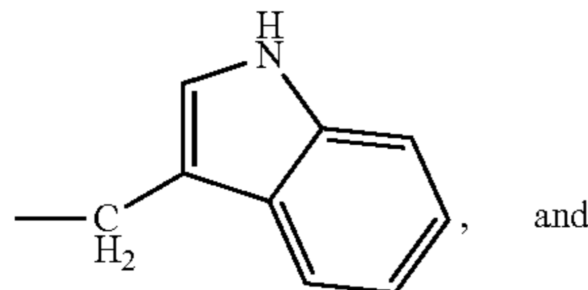
(tryptophan)
