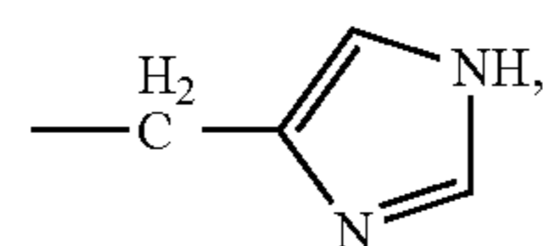
(histidine)
