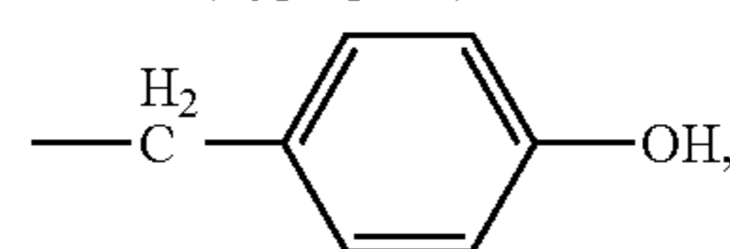
(tyrosine)
