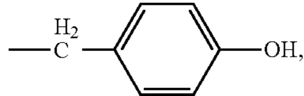
(tyrosine)
