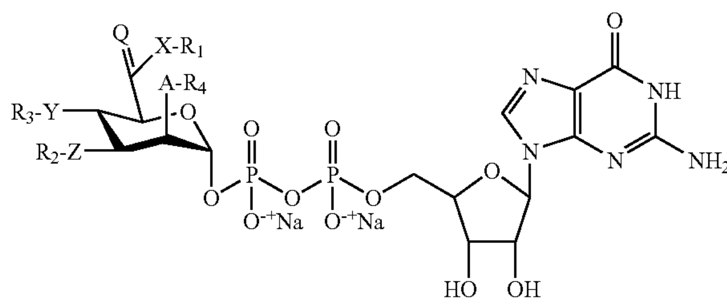
GDP-Mannose-derivatives
