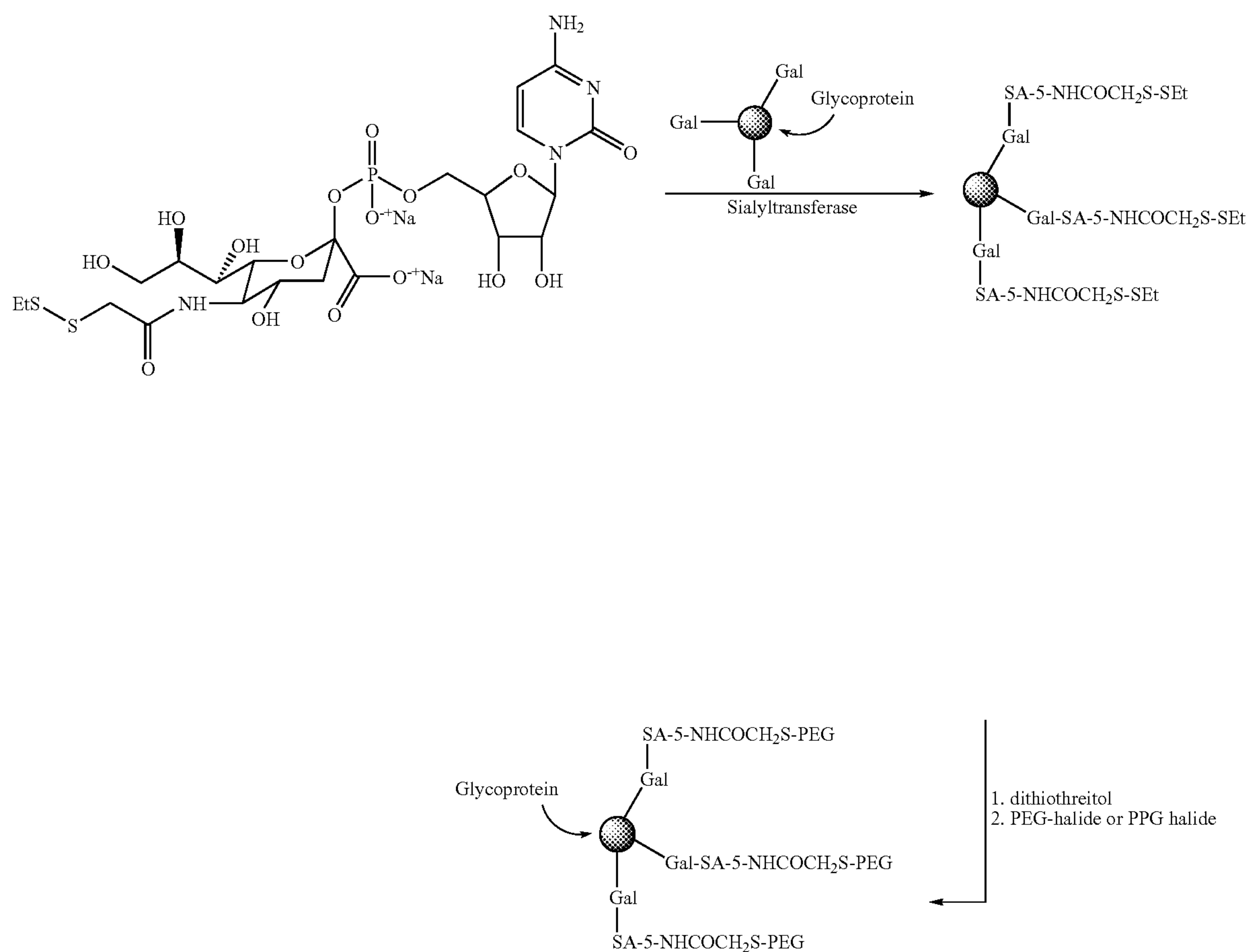
Scheme 2
