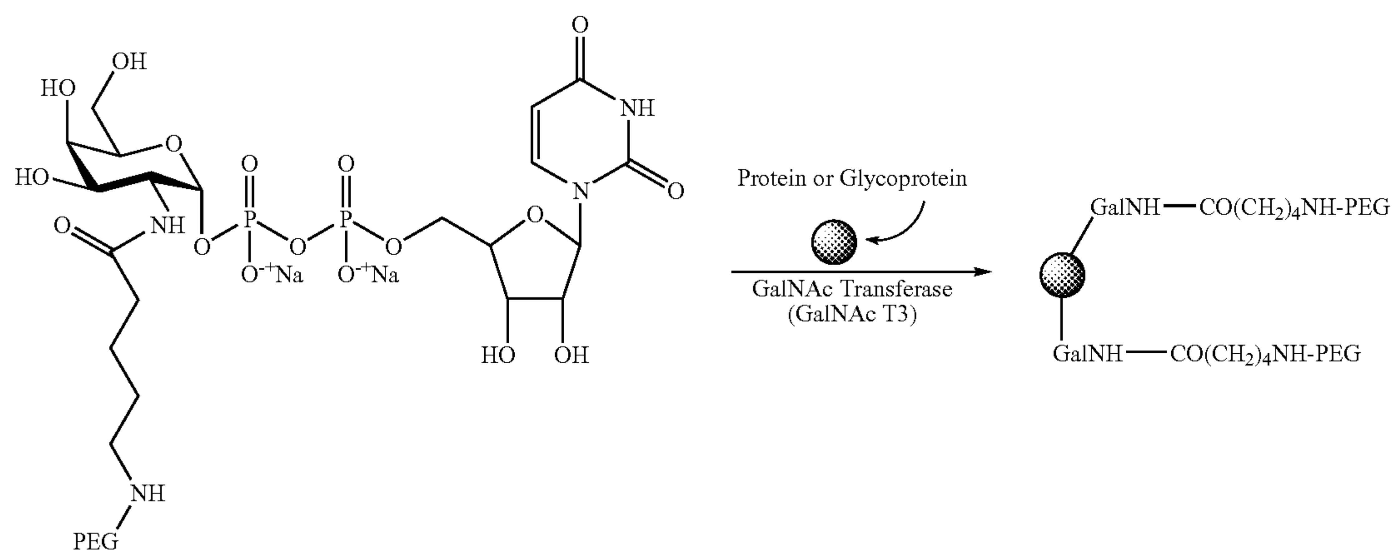
Scheme 3
