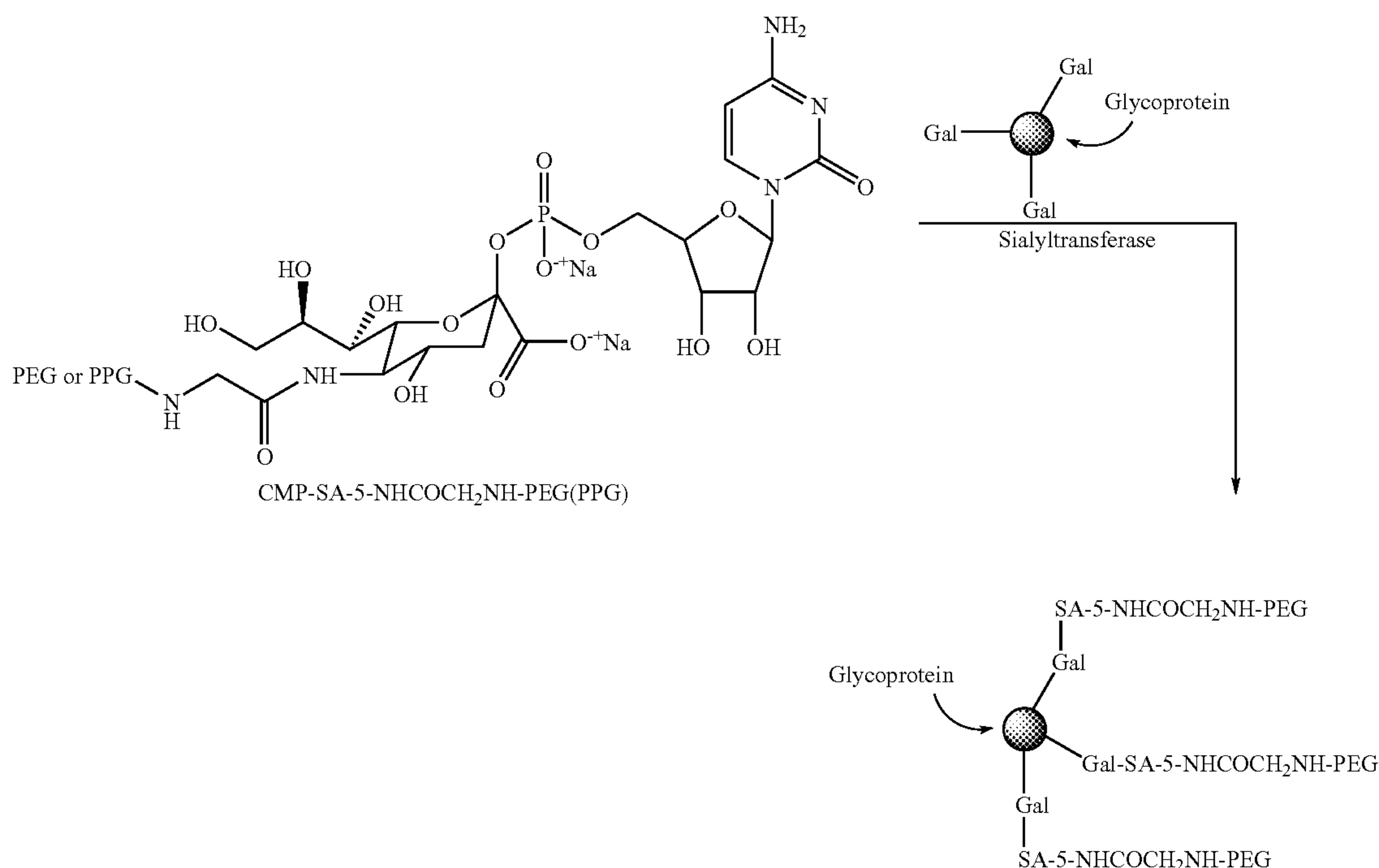
Scheme 1
