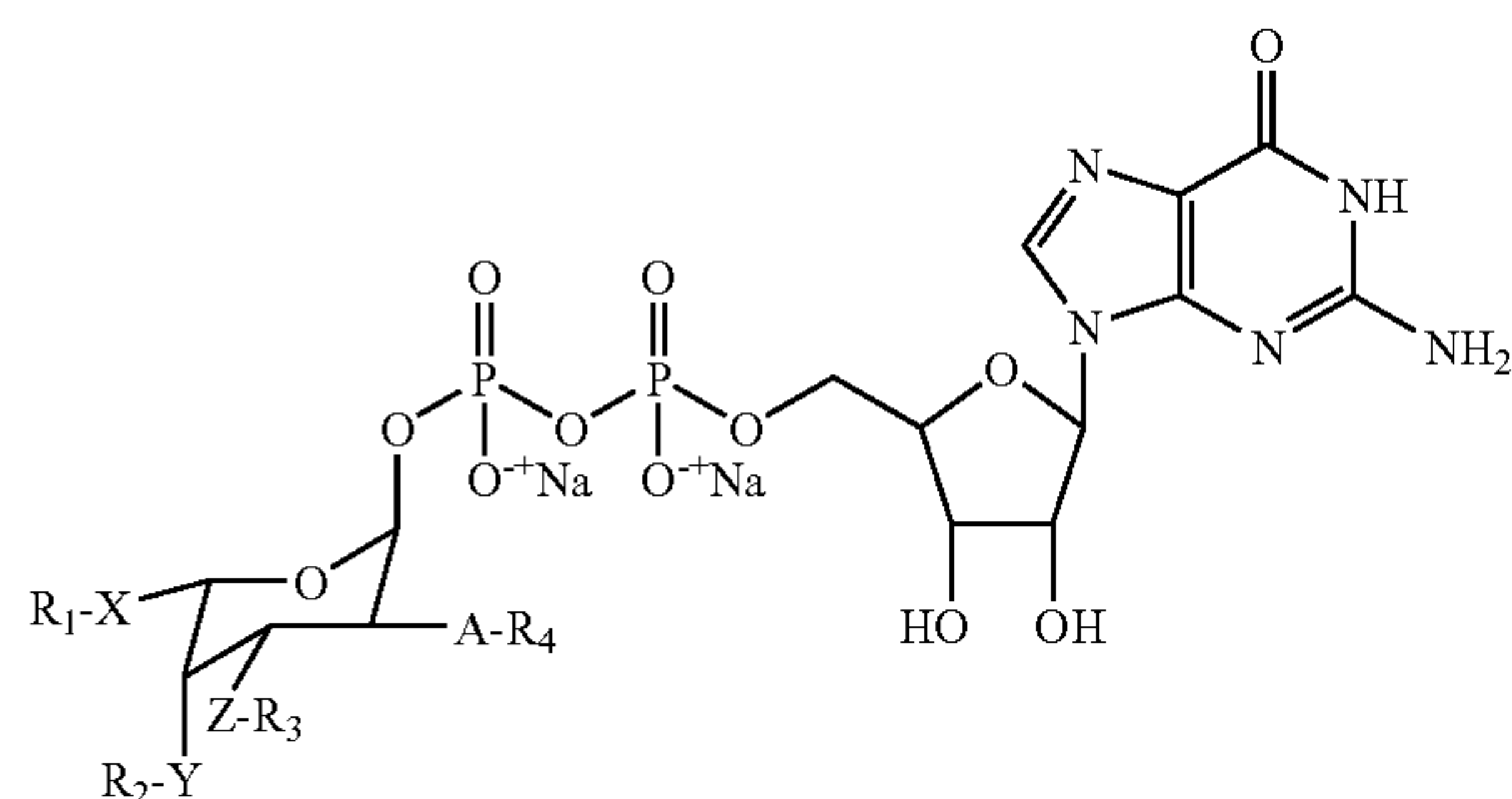
GDP-fucose-derivatives
