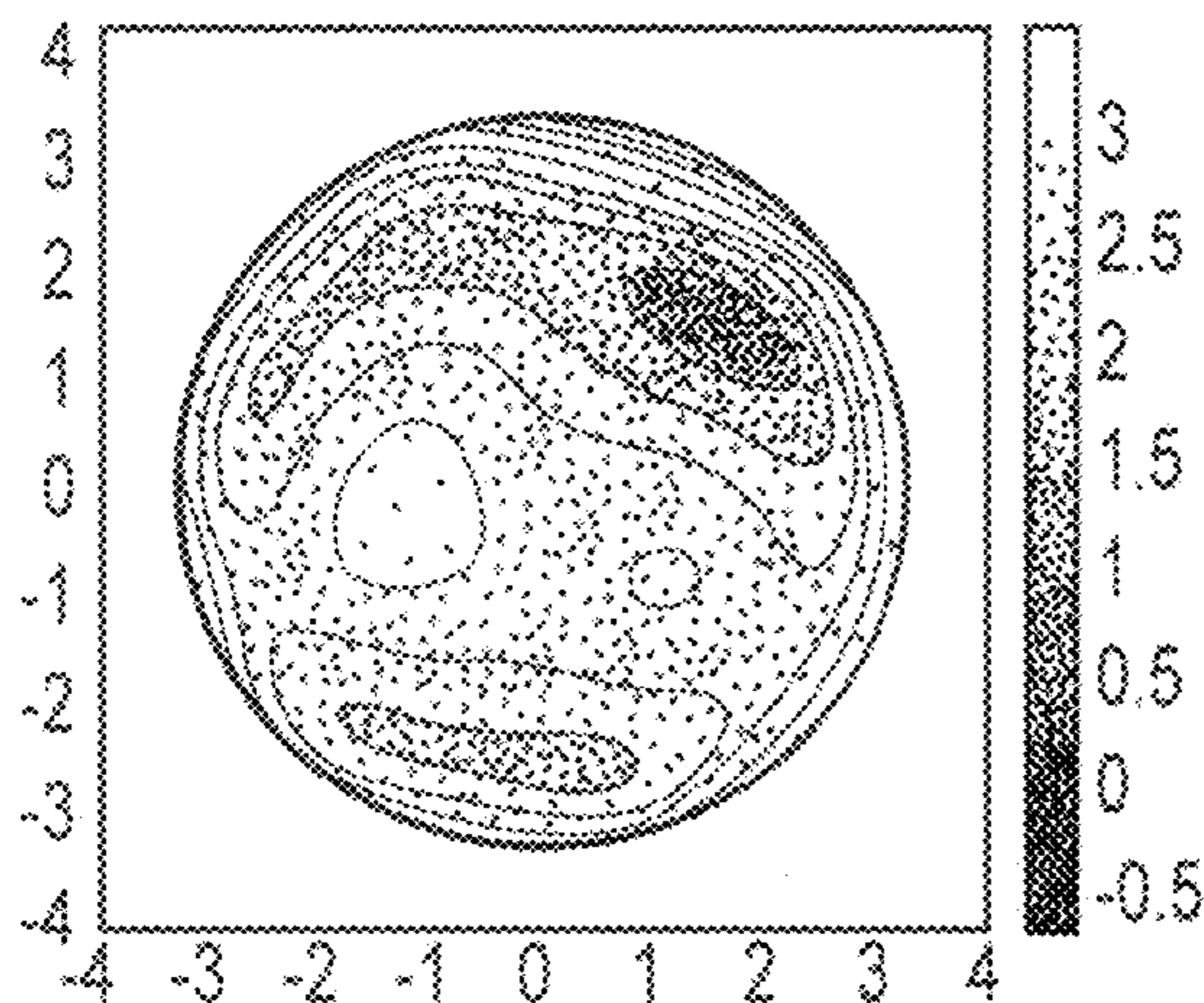
SINGLE EXAM SCALED UP. RMS ERROR = 0.154um
