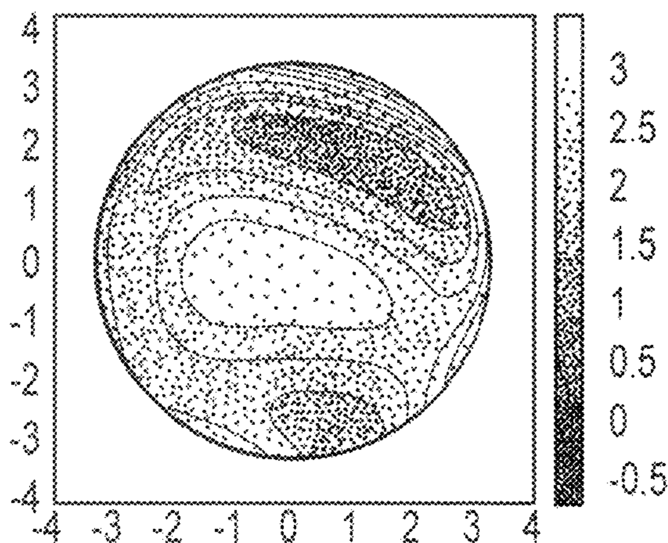
RMS ERROR = 0.061um AMONG (0.061, 0.124, 0.057, 0.094)
