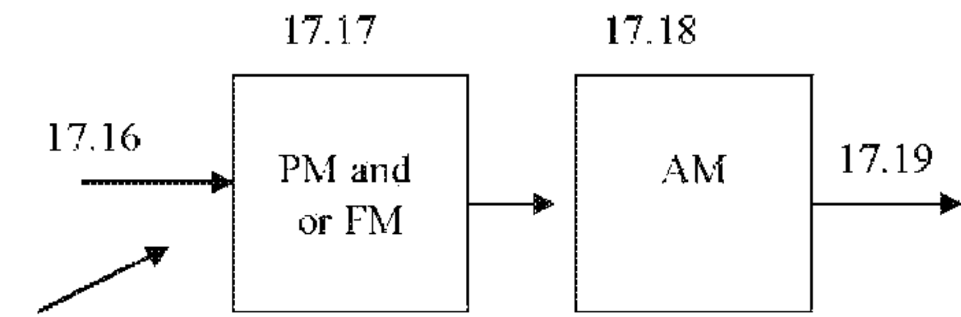
Fig. 17c An other prior art Non Quadrature Modulator
