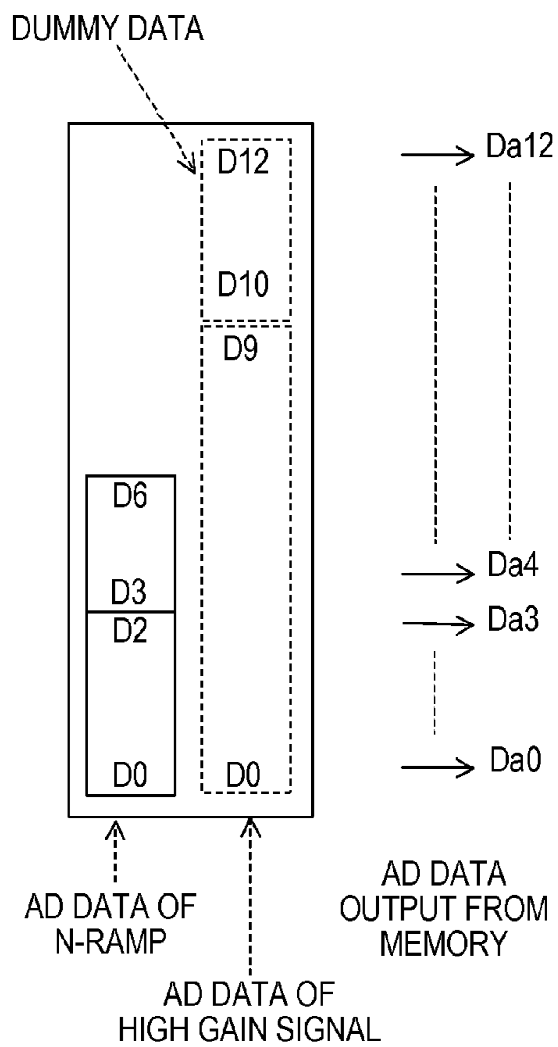
AD DATA IMAGE OF HIGH GAIN SIGNAL
