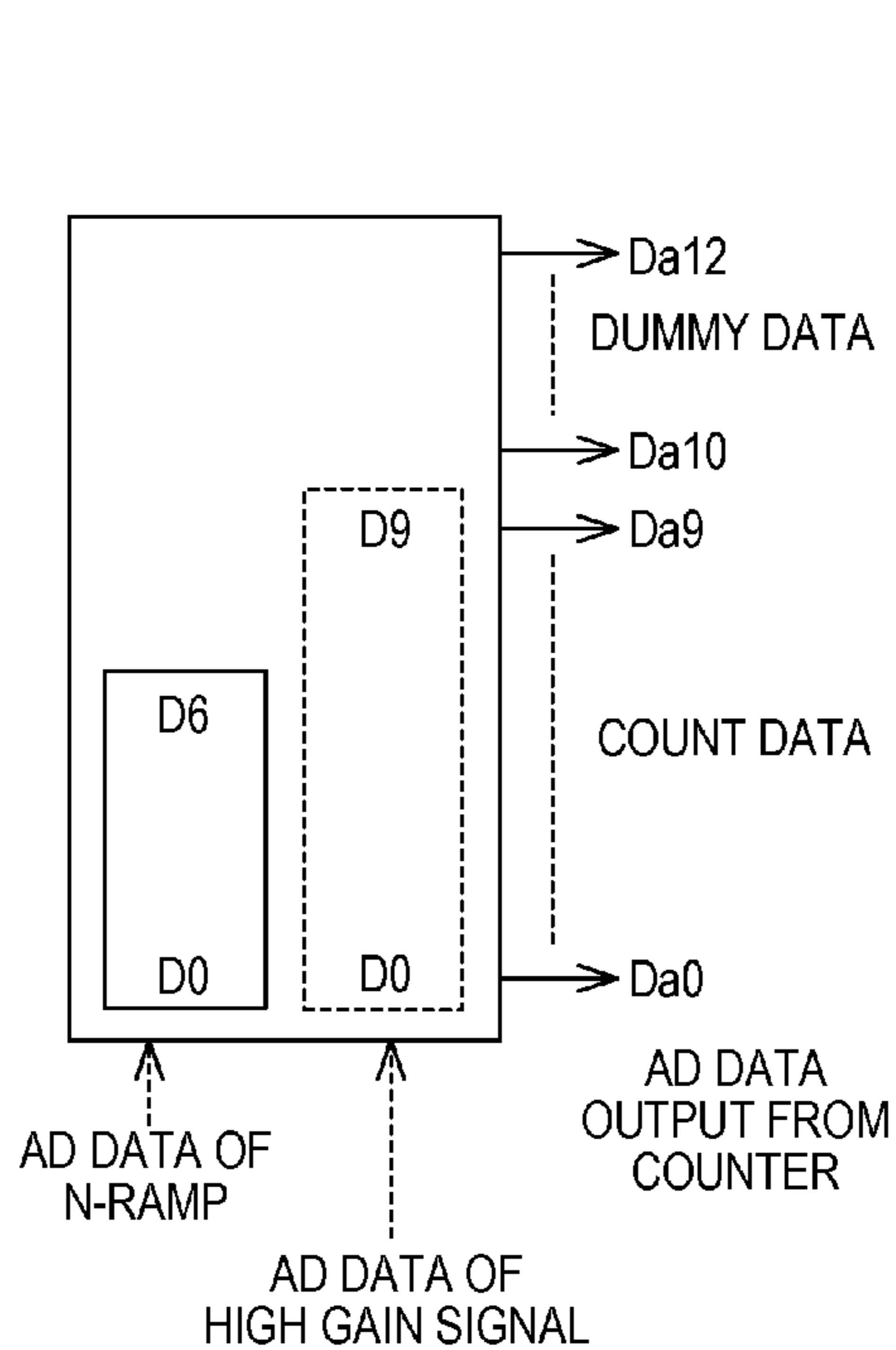
AD DATA IMAGE OF HIGH GAIN SIGNAL
