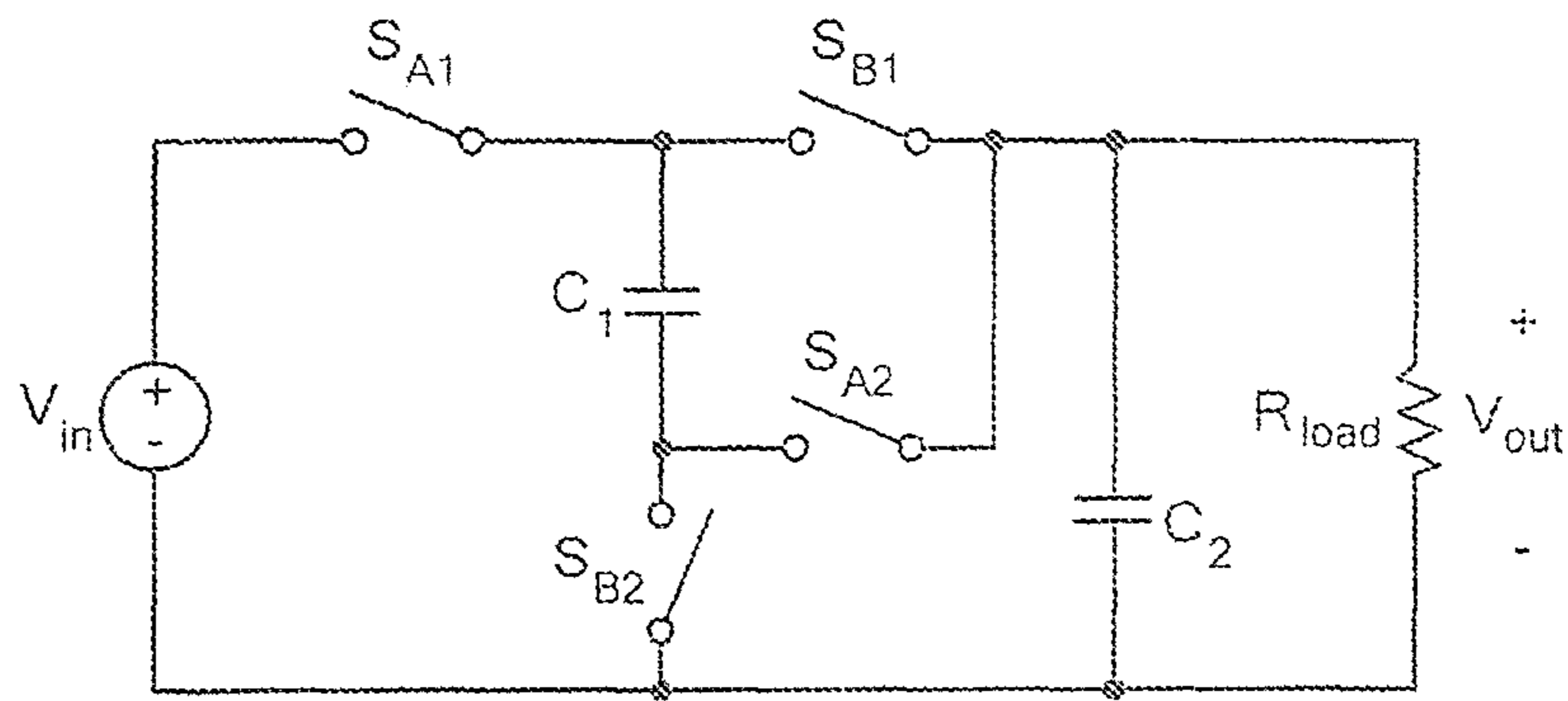
FIG. 1 PRIOR ART
